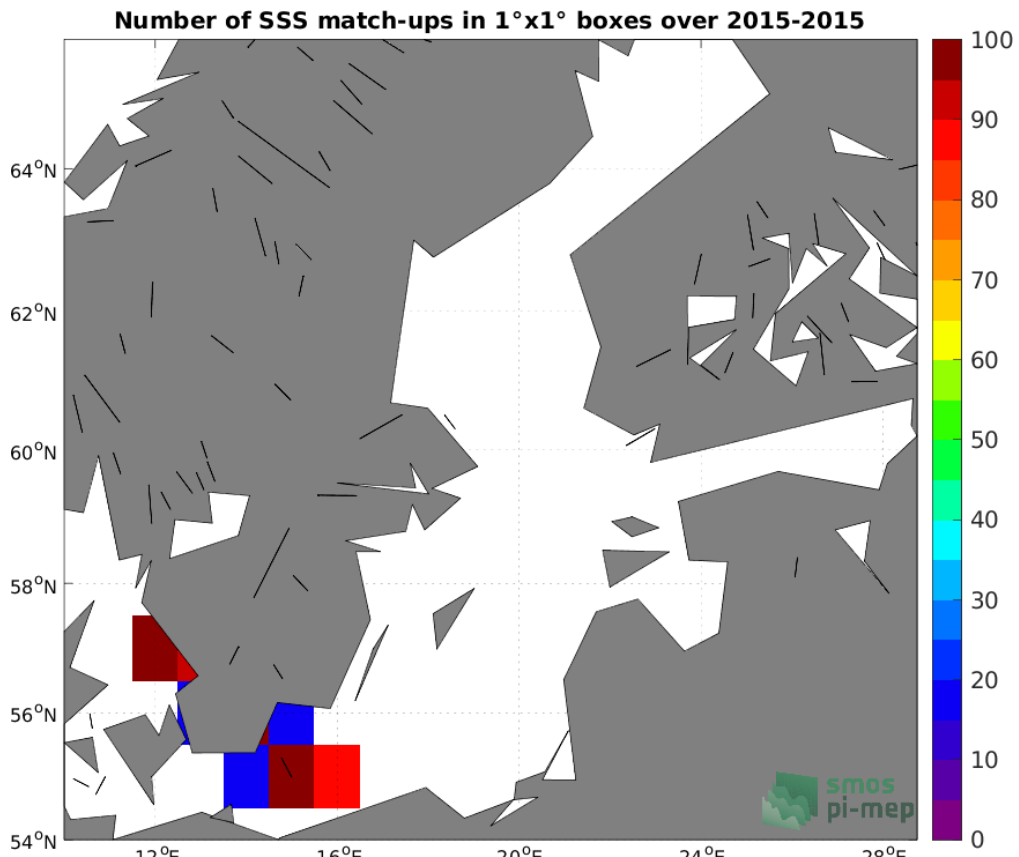
Figure 4: Number of SSS match-ups between TSG (GOSUD-Research-vessel) SSS and the SMOS SSS L3 v2 - 9-Days (BEC) SSS product for the Baltic Sea Pi-MEP region over 1°×1° boxes and for the full satellite product period.
