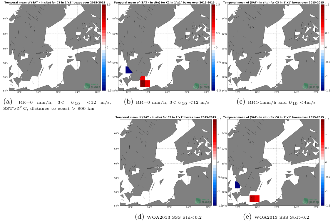
Figure 12: Temporal mean gridded over spatial boxes of size 1^{\circ}\times 1^{\circ} of \Delta SSS (SMOS SSS L3 v2 - 9-Days (BEC) - TSG (GOSUD-Research-vessel)) for 5 different subdatasets corresponding to:RR=0 mm/h, 3 < U_{10} < 12 m/s, SST >5^{\circ}\text{C} , distance to coast > 800 km (a), RR=0 mm/h, 3 < U_{10} < 12 m/s (b), RR >1 mm/h and U_{10} < 4 m/s (c), WOA2013 SSS Std <0.2 (d), WOA2013 SSS Std >0.2 (e).
