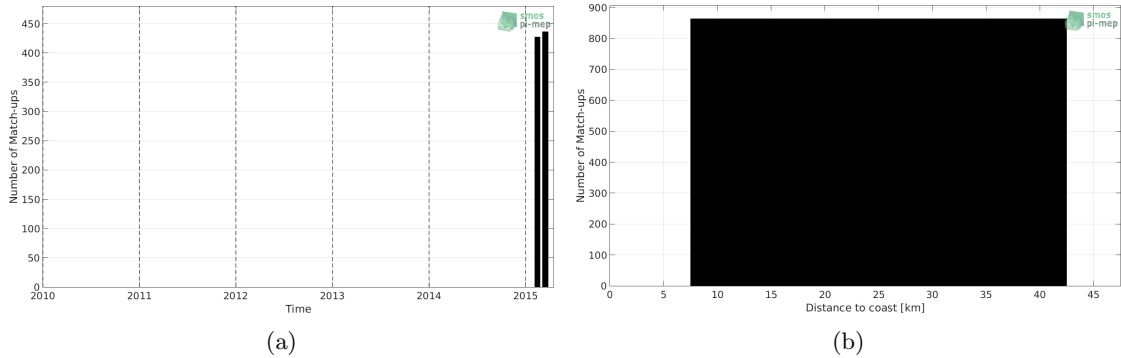
Figure 1: Number of match-ups between TSG (GOSUD-Research-vessel) and SMOS L3 v2 - 9-Days (BEC) SSS as a function of time (a) and as function of the distance to coast (b) over the Baltic Sea Pi-MEP region and for the full satellite product period.
