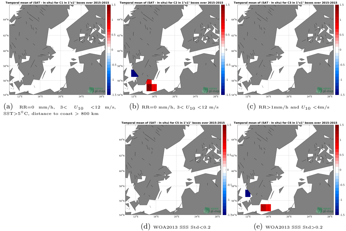
Figure 12: Temporal mean gridded over spatial boxes of size 1^\circ \times 1^\circ of \Delta SSS (SMOS L3 v2 - 9-Days (BEC) - TSG (GOSUD-Research-vessel)) for 5 different subdatasets corresponding to: RR=0 mm/h, 3 < U_{10} < 12 m/s, SST > 5^\circ\text{C} , distance to coast > 800 km (a), RR=0 mm/h, 3 < U_{10} < 12 m/s (b), RR > 1 mm/h and U_{10} < 4 m/s (c), WOA2013 SSS Std < 0.2 (d), WOA2013 SSS Std > 0.2 (e).
