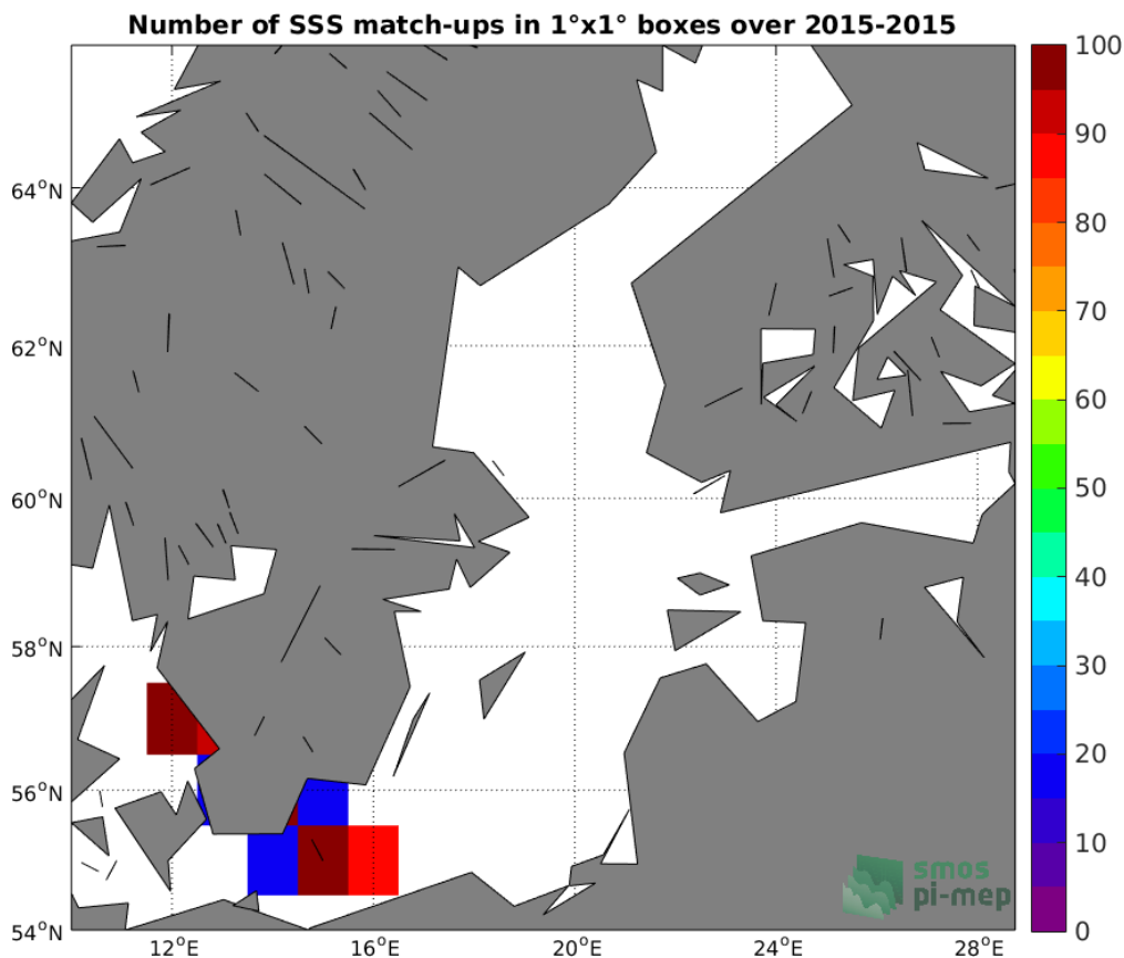
Figure 4: Number of SSS match-ups between TSG (GOSUD-Research-vessel) SSS and the SMOS L3 v2 - 9-Days (BEC) SSS product for the Baltic Sea Pi-MEP region over 1°x1° boxes and for the full satellite product period.
