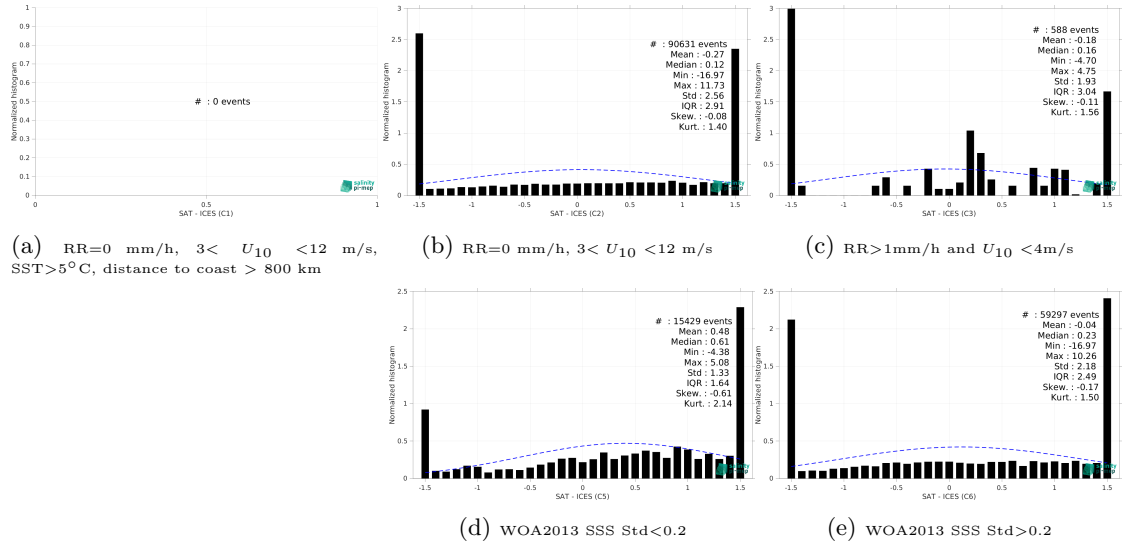
Figure 13: Normalized histogram of \Delta SSS (SMOS SSS L3 v2 - 9-Days (BEC) - ICES) for 5 different subdatasets corresponding to: RR=0 mm/h, 3 < U_{10} < 12 m/s, SST > 5°C, distance to coast > 800 km (a), RR=0 mm/h, 3 < U_{10} < 12 m/s (b), RR > 1mm/h and U_{10} < 4 m/s (c), WOA2013 SSS Std < 0.2 (d), WOA2013 SSS Std > 0.2 (e).
