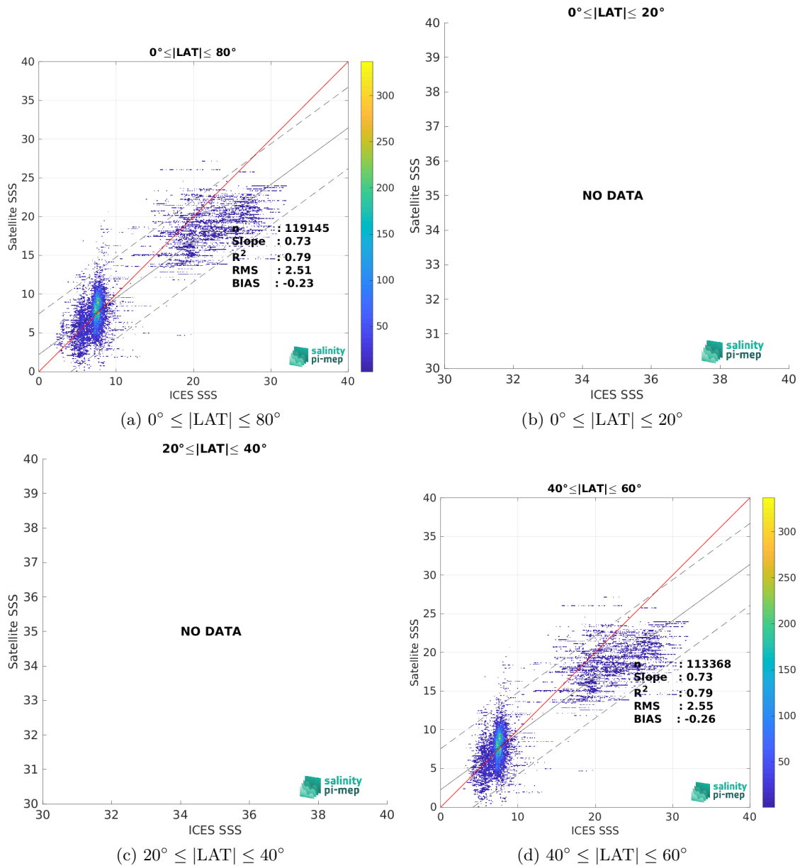
Figure 9: Contour maps of the concentration of SMOS SSS L3 v2 - 9-Days (BEC) SSS (y-axis) versus ICES SSS (x-axis) at match-up pairs for different latitude bands. For each plot, the red line shows x=y . The black thin and dashed lines indicate a linear fit through the data cloud and the \pm 95\% confidence levels, respectively. The number match-up pairs n , the slope and R^2 coefficient of the linear fit, the root mean square (RMS) and the mean bias between satellite and in situ data are indicated for each latitude band in each plots.
