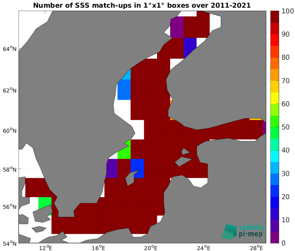
Figure 4: Number of SSS match-ups between ICES SSS and the SMOS SSS L3 v2 - 9-Days (BEC) SSS product for the Baltic Sea Pi-MEP region over 1^\circ \times 1^\circ boxes and for the full satellite product period.
