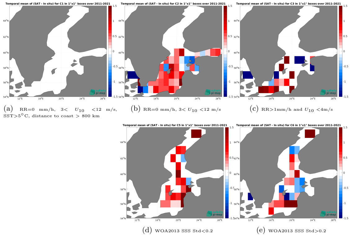
Figure 12: Temporal mean gridded over spatial boxes of size 1^{\circ}\times 1^{\circ} of \Delta\text{SSS} (SMOS SSS L3 v2 - 9-Days (BEC) - ICES) for 5 different subdatasets corresponding to:RR=0 mm/h, 3 < U_{10} < 12 m/s, SST >5^{\circ}\text{C} , distance to coast > 800 km (a), RR=0 mm/h, 3 < U_{10} < 12 m/s (b), RR >1 mm/h and U_{10} < 4 m/s (c), WOA2013 SSS Std <0.2 (d), WOA2013 SSS Std >0.2 (e).
