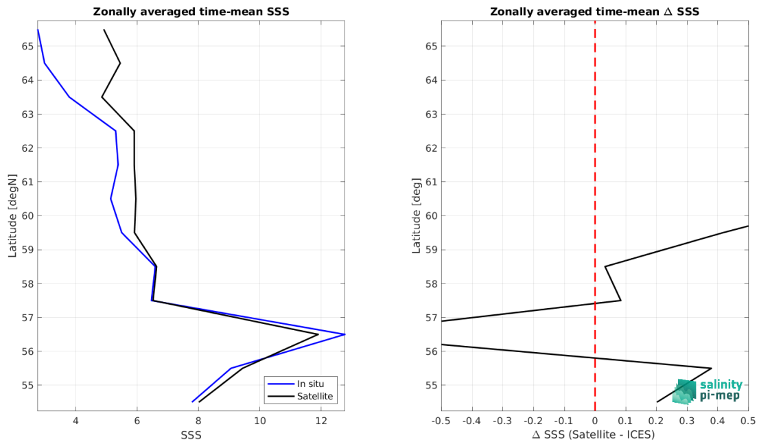
Figure 8: Left panel: Zonal mean SSS from SMOS SSS L3 v2 - 9-Days (BEC) satellite product (black) and from ICES (blue). Right panel: Zonal mean of \Delta SSS (Satellite - ICES) for all the collected Pi-MEP match-up pairs estimated over the full satellite product period.
