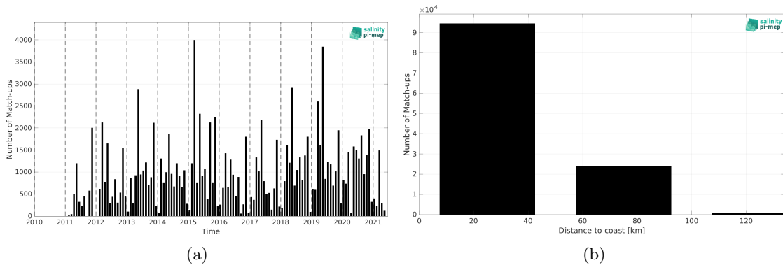
Figure 1: Number of match-ups between ICES and SMOS SSS L3 v2 - 9-Days (BEC) SSS as a function of time (a) and as function of the distance to coast (b) over the Baltic Sea Pi-MEP region and for the full satellite product period.
