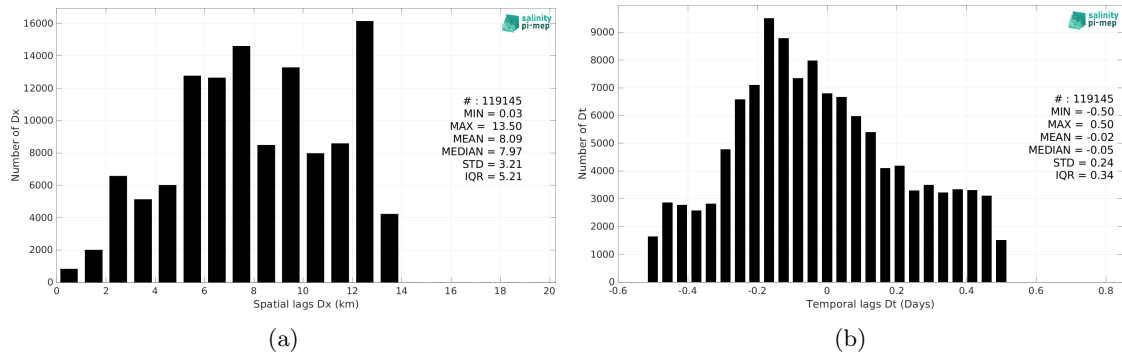
Figure 5: Histograms of the spatial (a) and temporal (b) lags between the location/time of the ICES measurement and the date of the corresponding SMOS SSS L3 v2 - 9-Days (BEC) SSS pixel.
