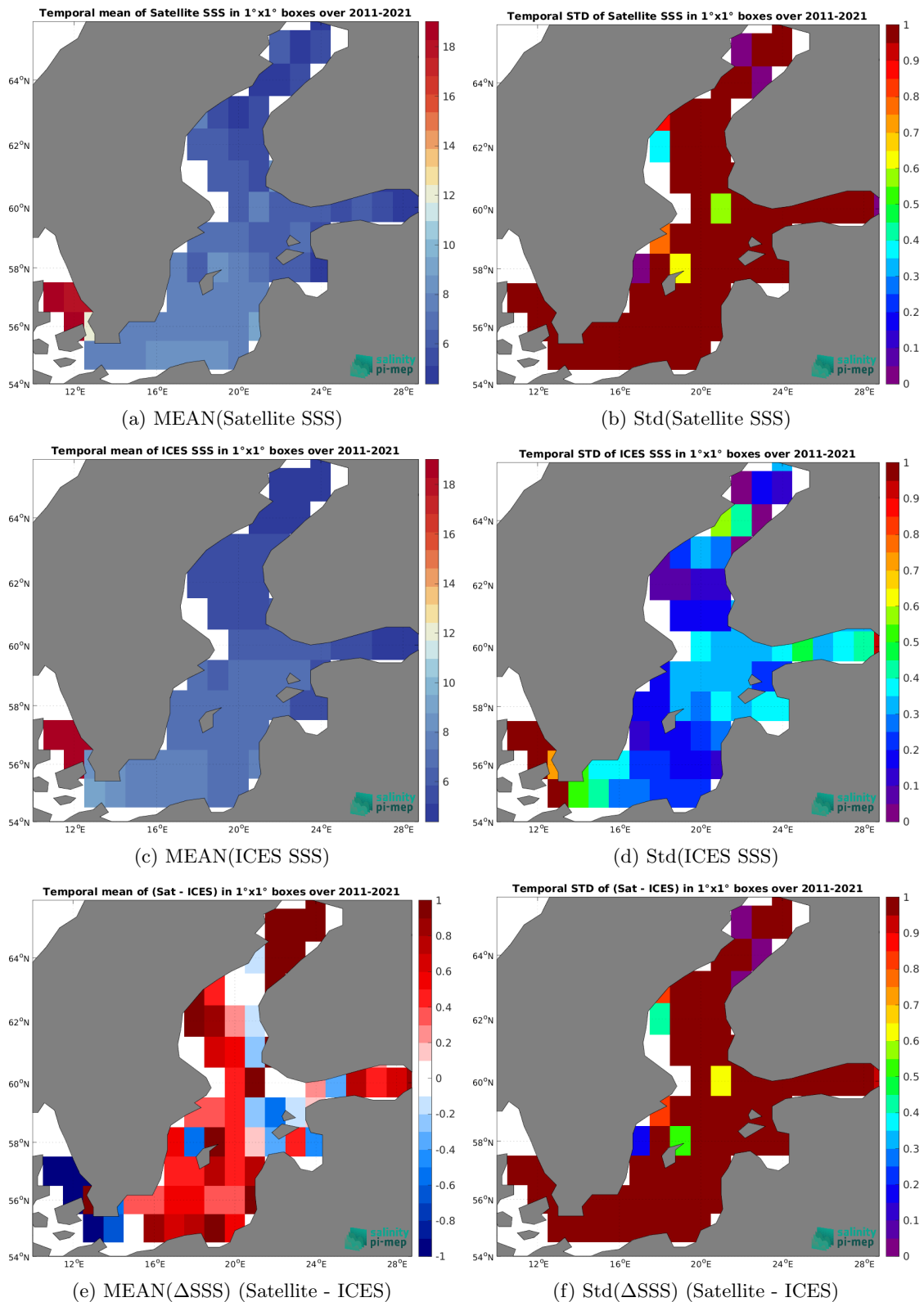
Figure 6: Temporal mean (left) and Std (right) of SSS from SMOS SSS L3 v2 - 9-Days (BEC) (top), ICES (middle), and of \Delta SSS (Satellite - ICES). Only match-up pairs are used to generate these maps.
