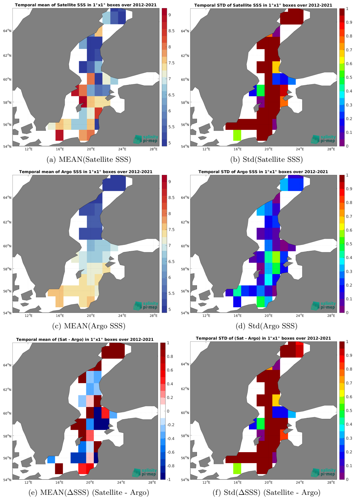
Figure 7: Temporal mean (left) and Std (right) of SSS from SMOS SSS L3 v2 - 9-Days (BEC) (top), Argo (middle), and of \Delta SSS (Satellite - Argo). Only match-up pairs are used to generate these maps.
