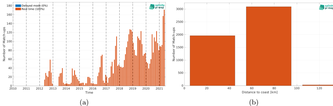
Figure 2: Number of match-ups between Argo and SMOS SSS L3 v2 - 9-Days (BEC) SSS as a function of time (a) and as function of the distance to coast (b) over the Baltic Sea Pi-MEP region and for the full satellite product period.
