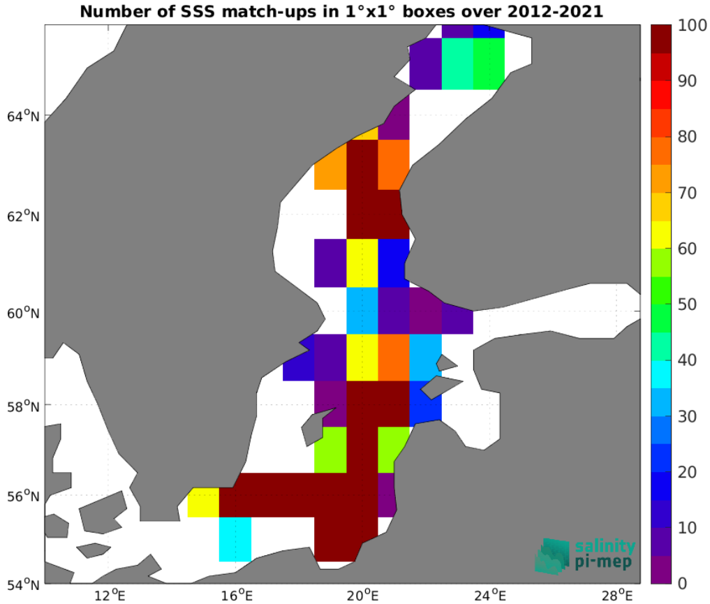
Figure 5: Number of SSS match-ups between Argo SSS and the SMOS SSS L3 v2 - 9-Days (BEC) SSS product for the Baltic Sea Pi-MEP region over 1^\circ \times 1^\circ boxes and for the full satellite product period.
