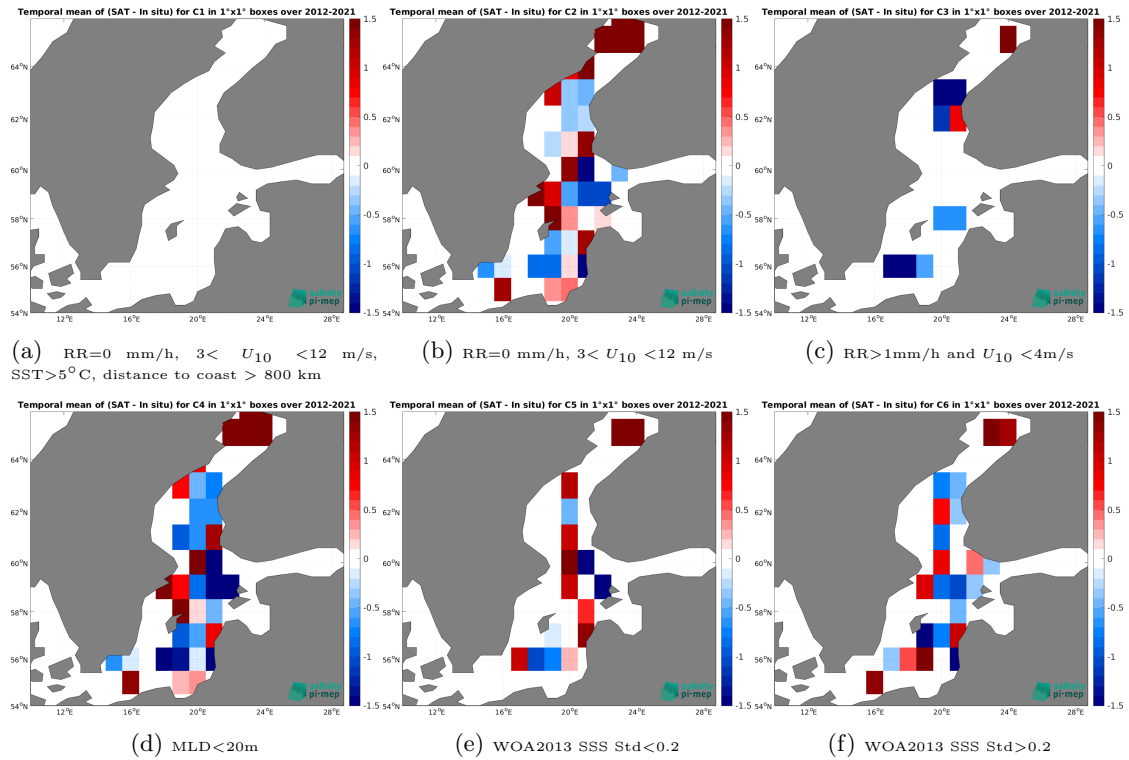
Figure 14: Temporal mean gridded over spatial boxes of size 1^\circ \times 1^\circ of \Delta SSS (SMOS SSS L3 v2 - 9-Days (BEC) - Argo) for 6 different subdatasets corresponding to:RR=0 mm/h, 3 < U_{10} < 12 m/s, SST>5°C, distance to coast > 800 km (a), RR=0 mm/h, 3 < U_{10} < 12 m/s (b), RR>1mm/h and U_{10} < 4 m/s (c),MLD<20m (d),WOA2013 SSS Std<0.2 (e),WOA2013 SSS Std>0.2 (f).
