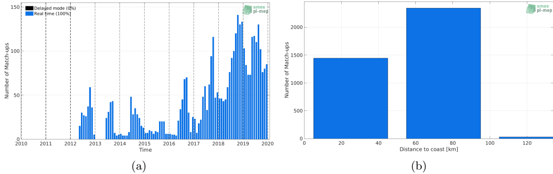
Figure 1: Number of match-ups between Argo and SMOS SSS L3 v2 - 9-Days (BEC) SSS as a function of time (a) and as function of the distance to coast (b) over the Baltic Sea Pi-MEP region and for the full satellite product period.
