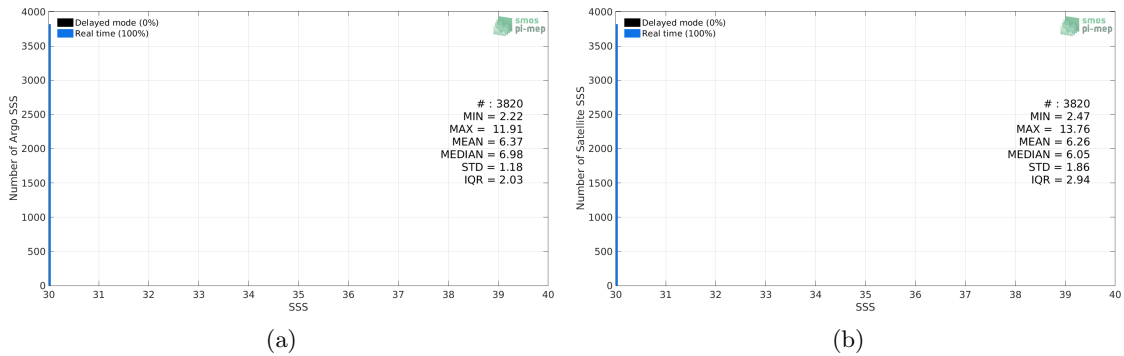
Figure 2: Histograms of SSS from Argo (a) and SMOS SSS L3 v2 - 9-Days (BEC) (b) considering all match-up pairs per bins of 0.1 over the Baltic Sea Pi-MEP region and for the full satellite product period.
