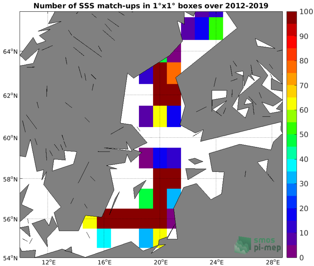
Figure 4: Number of SSS match-ups between Argo SSS and the SMOS SSS L3 v2 - 9-Days (BEC) SSS product for the Baltic Sea Pi-MEP region over 1°x1° boxes and for the full satellite product period.
