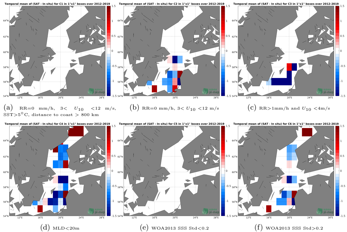
Figure 12: Temporal mean gridded over spatial boxes of size 1^{\circ}\times 1^{\circ} of \Delta\text{SSS} (SMOS SSS L3 v2 - 9-Days (BEC) - Argo) for 6 different subdatasets corresponding to:RR=0 mm/h, 3 < U_{10} < 12 m/s, SST >5^{\circ}\text{C} , distance to coast > 800 km (a), RR=0 mm/h, 3 < U_{10} < 12 m/s (b), RR >1 mm/h and U_{10} < 4 m/s (c),MLD <20 m (d),WOA2013 SSS Std <0.2 (e),WOA2013 SSS Std >0.2 (f).
