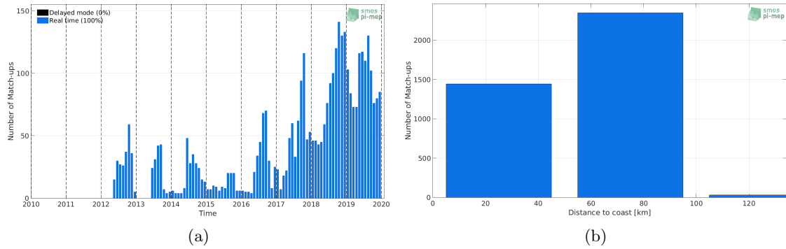
Figure 1: Number of match-ups between Argo and SMOS L3 v2 - 9-Days (BEC) SSS as a function of time (a) and as function of the distance to coast (b) over the Baltic Sea Pi-MEP region and for the full satellite product period.
