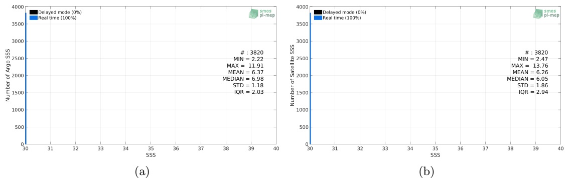
Figure 2: Histograms of SSS from Argo (a) and SMOS L3 v2 - 9-Days (BEC) (b) considering all match-up pairs per bins of 0.1 over the Baltic Sea Pi-MEP region and for the full satellite product period.
