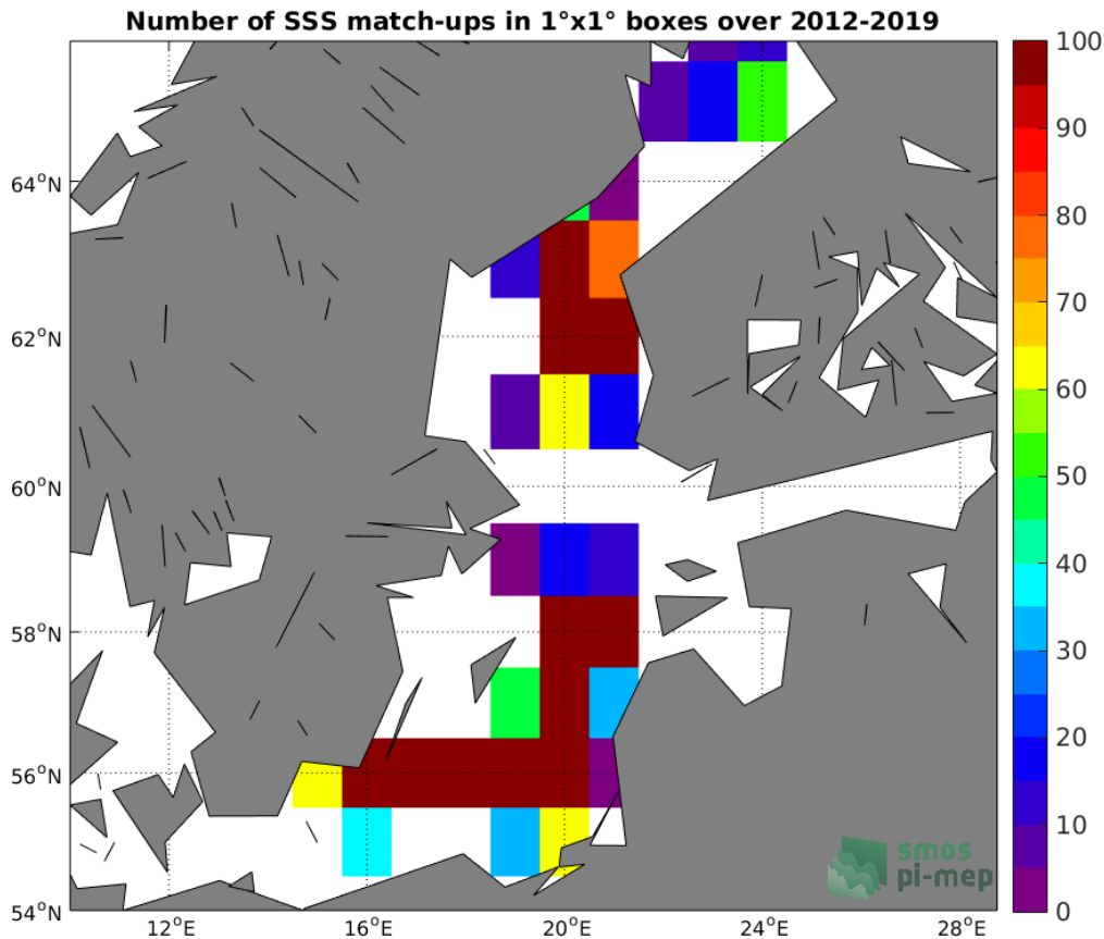
Figure 4: Number of SSS match-ups between Argo SSS and the SMOS L3 v2 - 9-Days (BEC) SSS product for the Baltic Sea Pi-MEP region over 1°x1° boxes and for the full satellite product period.
