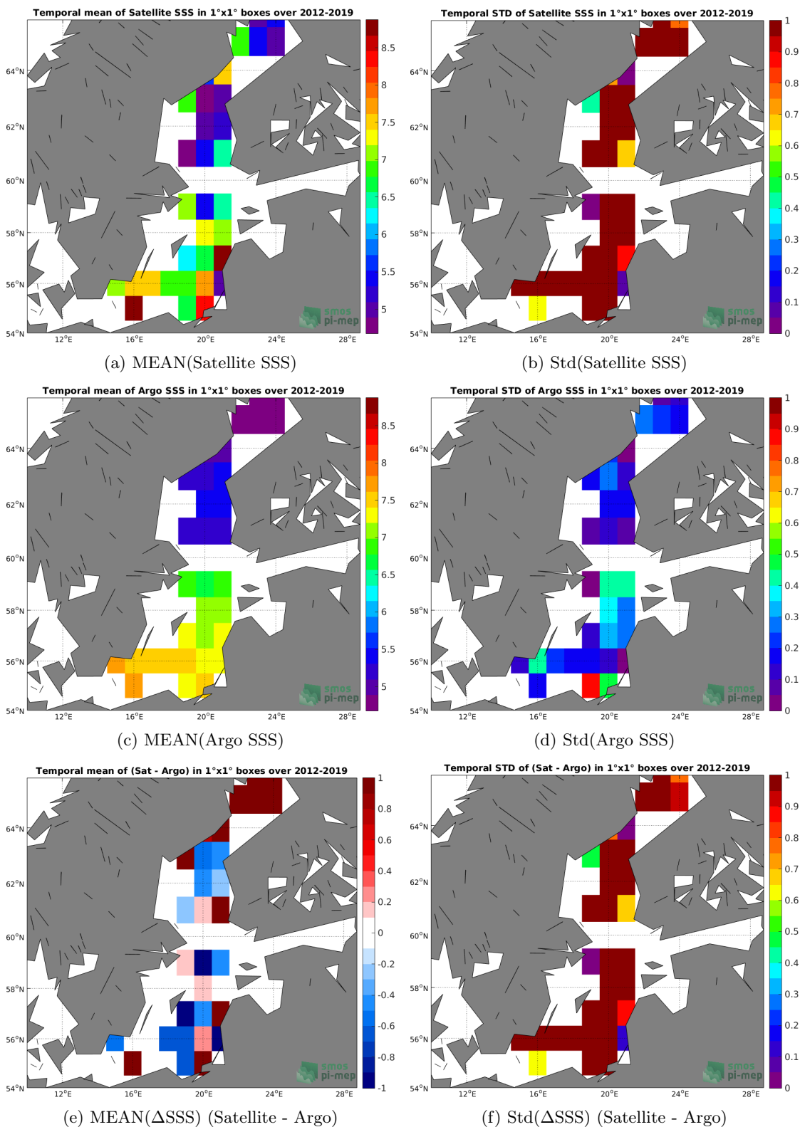
Figure 6: Temporal mean (left) and Std (right) of SSS from SMOS L3 v2 - 9-Days (BEC) (top), Argo (middle), and of \Delta SSS (Satellite - Argo). Only match-up pairs are used to generate these maps.
