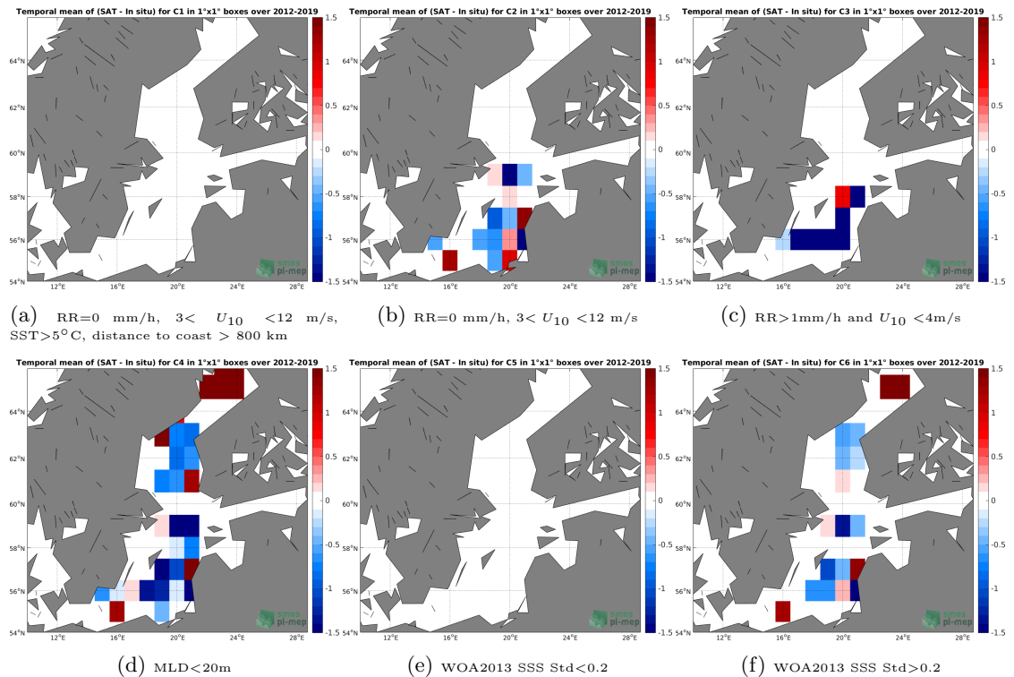
Figure 12: Temporal mean gridded over spatial boxes of size 1^{\circ}\times 1^{\circ} of \Delta\text{SSS} (SMOS L3 v2 - 9-Days (BEC) - Argo) for 6 different subdatasets corresponding to:RR=0 mm/h, 3 < U_{10} < 12 m/s, SST > 5^{\circ}\text{C} , distance to coast > 800 km (a), RR=0 mm/h, 3 < U_{10} < 12 m/s (b), RR > 1\text{mm/h} and U_{10} < 4\text{m/s} (c),MLD < 20\text{m} (d),WOA2013 SSS Std < 0.2 (e),WOA2013 SSS Std > 0.2 (f).
