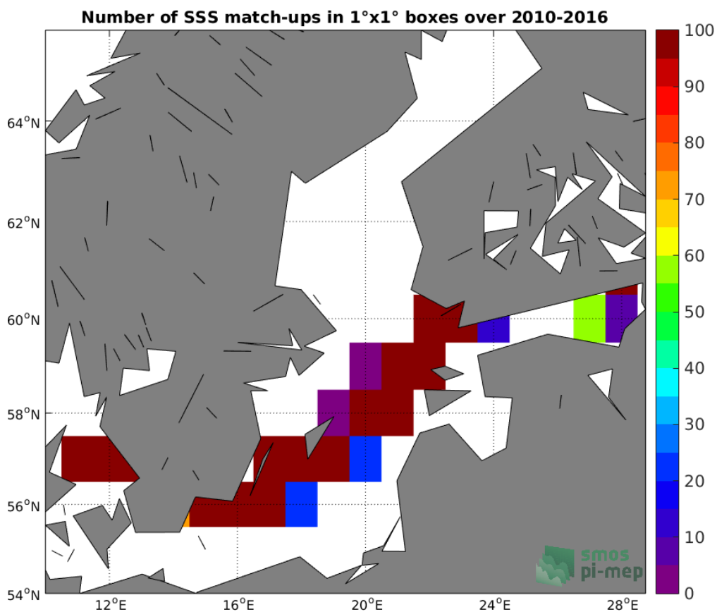
Figure 4: Number of SSS match-ups between TSG-LEGOS-DM SSS and the SMOS-L3-BEC-OA-V1-9DAYS-0.25DEG SSS product for the Baltic Sea Pi-MEP region over 1°x1° boxes and for the full satellite product period.
