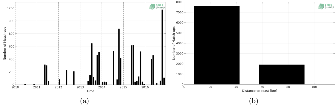
Figure 1: Number of match-ups between TSG-LEGOS-DM and SMOS-L3-BEC-OA-V1-9DAYS-0.25DEG SSS as a function of time (a) and as function of the distance to coast (b) over the Baltic Sea Pi-MEP region and for the full satellite product period.
