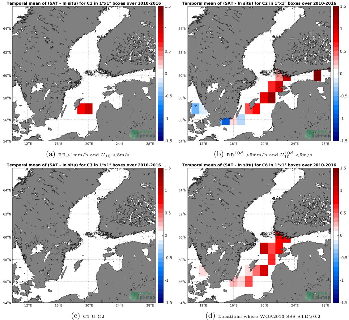
Figure 12: Temporal mean gridded over spatial boxes of size 1^\circ \times 1^\circ of \Delta SSS (SMOS-L3-BEC-OA-V1-9DAYS-0.25DEG - TSG-LEGOS-DM) for 4 different subdatasets corresponding to: RR > 1\text{mm/h} and U_{10} < 5\text{m/s} (a), RR^{10d} > 5\text{mm/h} and U_{10}^{10d} < 5\text{m/s} (b), C1 U C2 (c), Locations where WOA2013 SSS STD > 0.2 (d).
