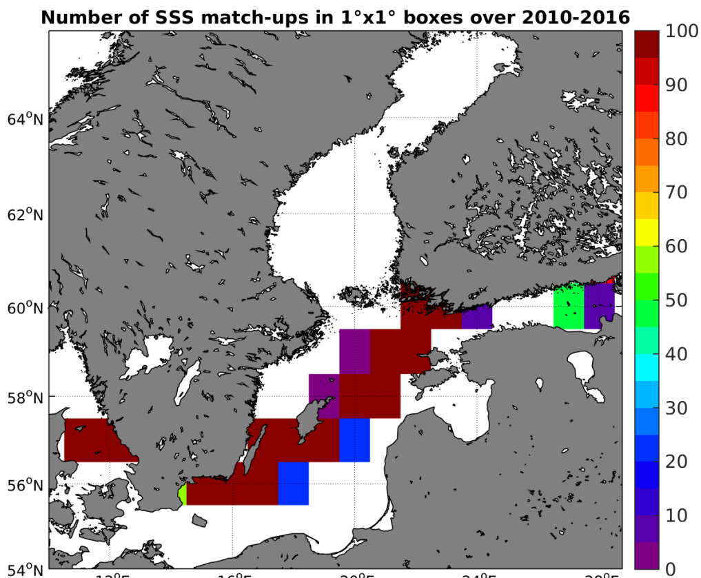
Figure 4: Number of SSS match-ups between TSG-LEGOS-DM SSS and the SMOS-L3-BEC-OA-V1-9DAYS-0.25DEG SSS product for the Baltic Sea Pi-MEP region over 1°x1° boxes and for the full satellite product period.
