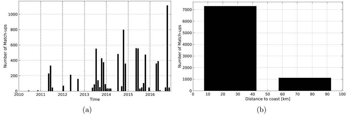
Figure 1: Number of match-ups between TSG-LEGOS-DM and SMOS-L3-BEC-OA-V1-9DAYS-0.25DEG SSS as a function of time (a) and as function of the distance to coast (b) over the Baltic Sea Pi-MEP region and for the full satellite product period.
