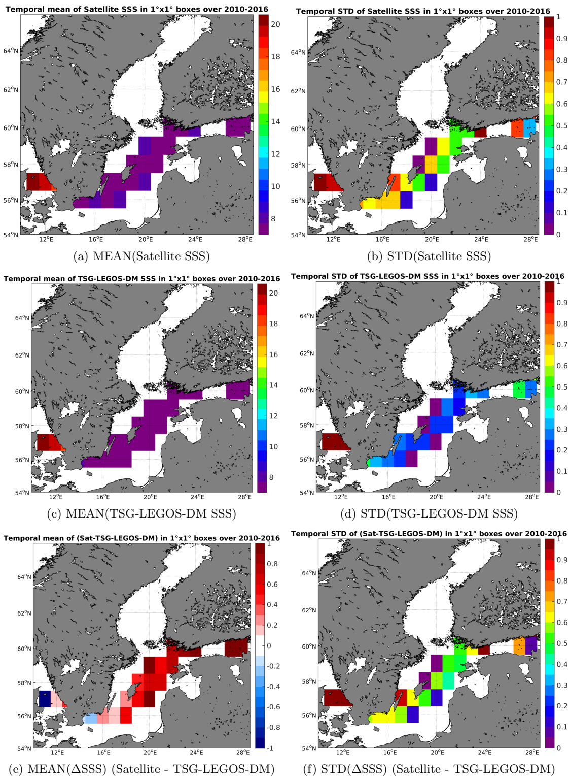
Figure 6: Temporal mean (left) and STD (right) of SSS from SMOS-L3-BEC-OA-V1-9DAYS-0.25DEG (top), TSG-LEGOS-DM (middle), and of \Delta SSS (Satellite - TSG-LEGOS-DM). Only match-up pairs are used to generate these maps.
