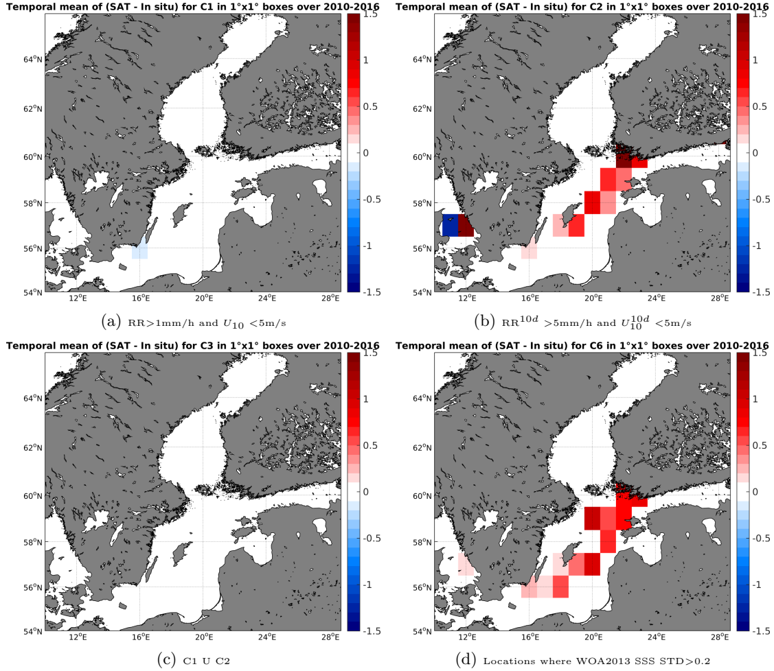
Figure 12: Temporal mean gridded over spatial boxes of size 1°x1° of \Delta SSS (SMOS-L3-BEC-OA-V1-9DAYS-0.25DEG - TSG-LEGOS-DM) for 4 different subdatasets corresponding to: RR > 1\text{mm/h} and U_{10} < 5\text{m/s} (a), RR^{10d} > 5\text{mm/h} and U_{10}^{10d} < 5\text{m/s} (b), C1 U C2 (c), Locations where WOA2013 SSS STD > 0.2 (d).
