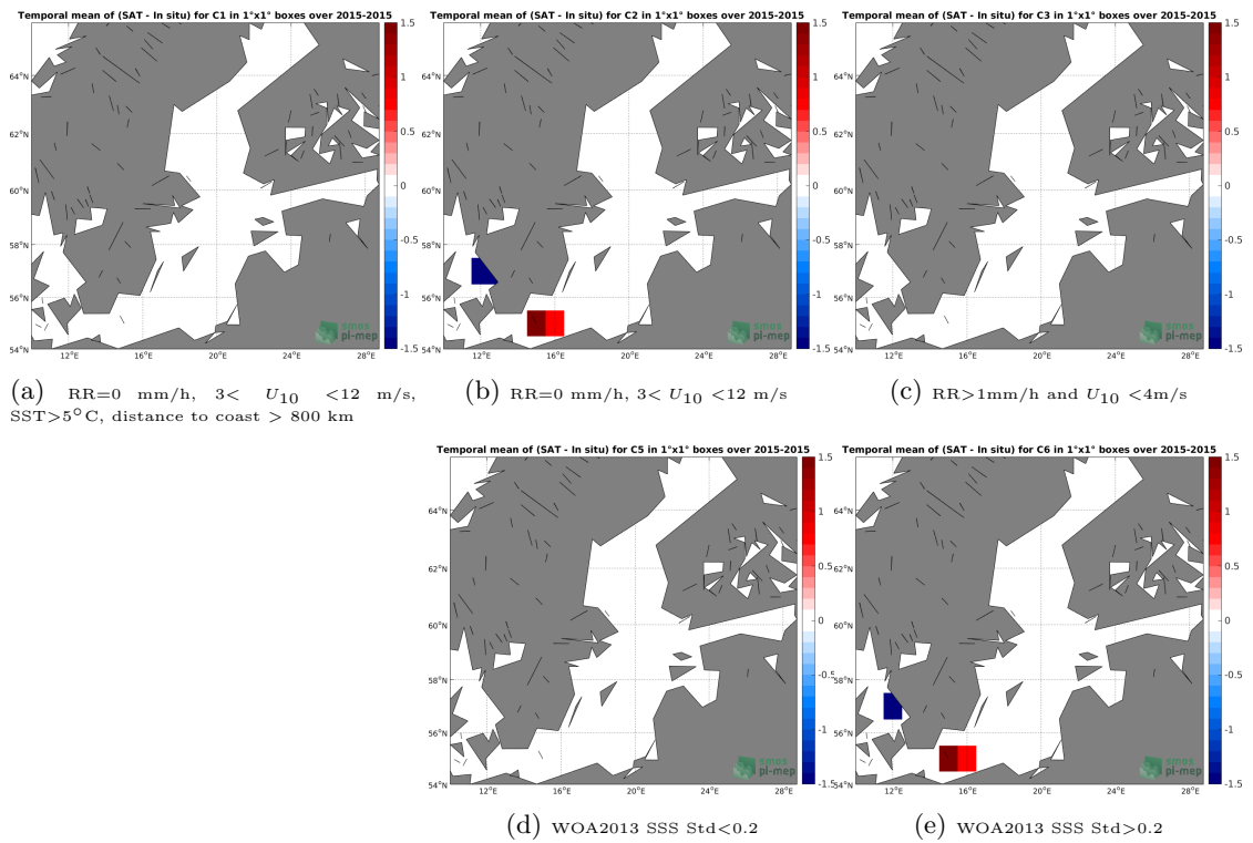
Figure 12: Temporal mean gridded over spatial boxes of size 1°x1° of \Delta SSS (SMOS-L3-BEC-OA-V1-9DAYS-0.25DEG - TSG-GOSUD-Research-vessel) for 5 different subdatasets corresponding to:RR=0 mm/h, 3 < U_{10} < 12 m/s, SST>5°C, distance to coast > 800 km (a), RR=0 mm/h, 3 < U_{10} < 12 m/s (b), RR>1mm/h and U_{10} < 4 m/s (c), WOA2013 SSS Std<0.2 (d), WOA2013 SSS Std>0.2 (e).
