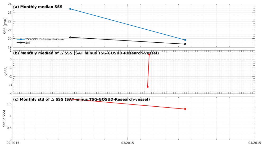
Figure 7: Time series of the monthly median SSS (top), median of \Delta SSS (Satellite - TSG-GOSUD-Research-vessel) and Std of \Delta SSS (Satellite - TSG-GOSUD-Research-vessel) over the Baltic Sea Pi-MEP region considering all match-ups collected by the Pi-MEP.
