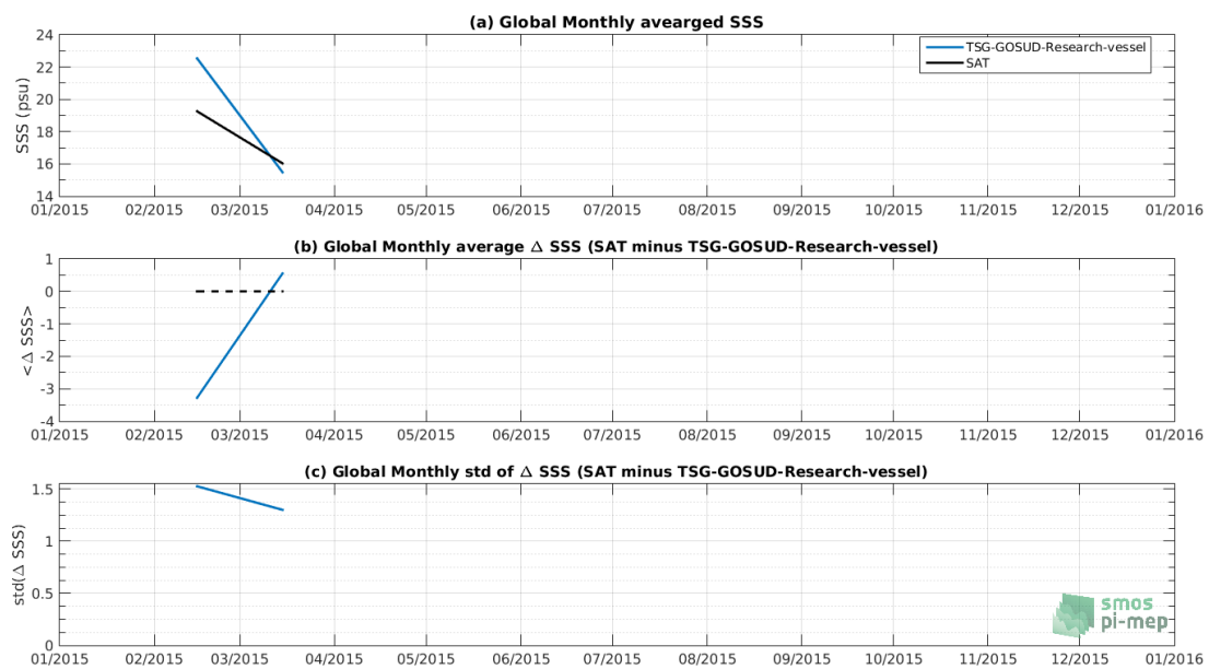
Figure 7: Time series of the monthly averaged mean SSS (top), mean \Delta SSS (Satellite - TSG-GOSUD-Research-vessel) and STD of \Delta SSS (Satellite - TSG-GOSUD-Research-vessel) over the Baltic Sea Pi-MEP region considering all match-ups collected by the Pi-MEP platform.
