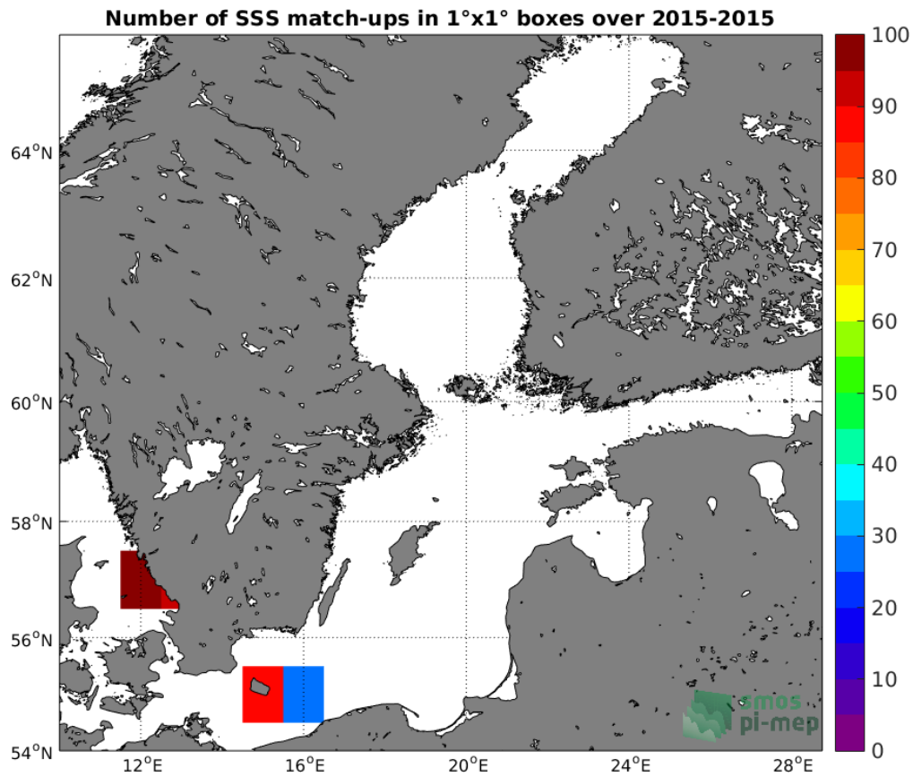
Figure 4: Number of SSS match-ups between TSG-GOSUD-Research-vessel SSS and the SMOS-L3-BEC-OA-V1-9DAYS-0.25DEG SSS product for the Baltic Sea Pi-MEP region over 1°x1° boxes and for the full satellite product period.
