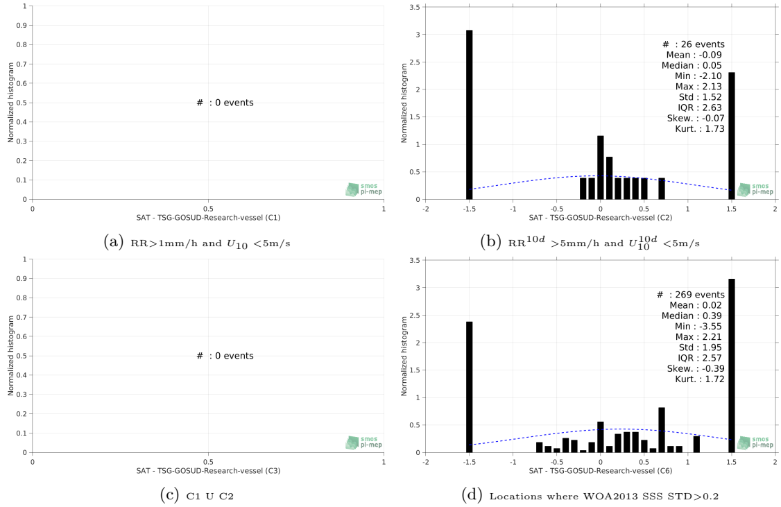
Figure 13: Normalized histogram of \Delta\text{SSS} (SMOS-L3-BEC-OA-V1-9DAYS-0.25DEG - TSG-GOSUD-Research-vessel) for 6 different subdatasets corresponding to: RR > 1\text{mm/h} and U_{10} < 5\text{m/s} (a), RR^{10d} > 5\text{mm/h} and U_{10}^{10d} < 5\text{m/s} (b), C1 \cup C2 (c), Locations where WOA2013 SSS STD > 0.2 (d).
