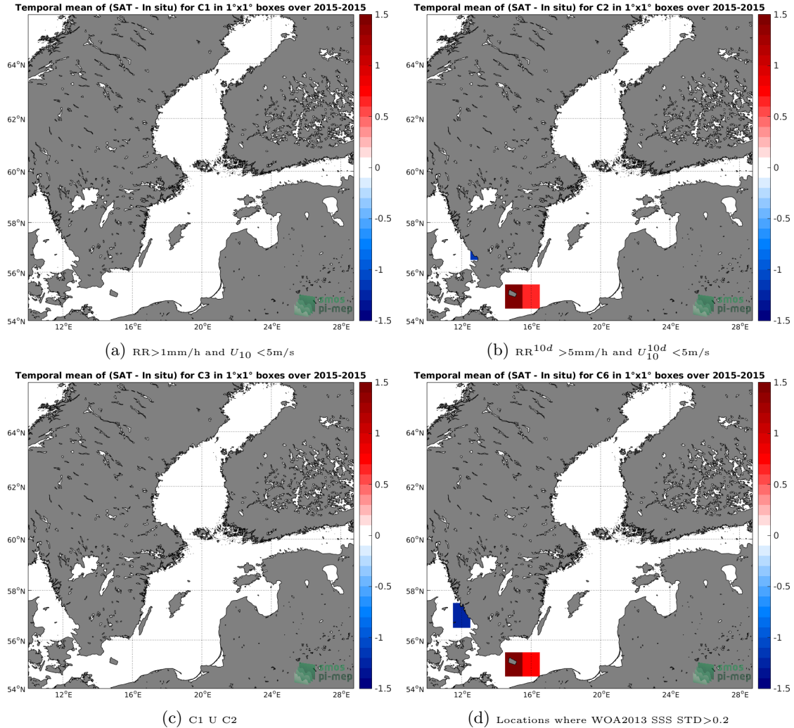
Figure 12: Temporal mean gridded over spatial boxes of size 1^\circ \times 1^\circ of \Delta SSS (SMOS-L3-BEC-OA-V1-9DAYS-0.25DEG - TSG-GOSUD-Research-vessel) for 4 different subdatasets corresponding to: RR > 1\text{mm/h} and U_{10} < 5\text{m/s} (a), RR^{10d} > 5\text{mm/h} and U_{10}^{10d} < 5\text{m/s} (b), C1 U C2 (c), Locations where WOA2013 SSS STD > 0.2 (d).
