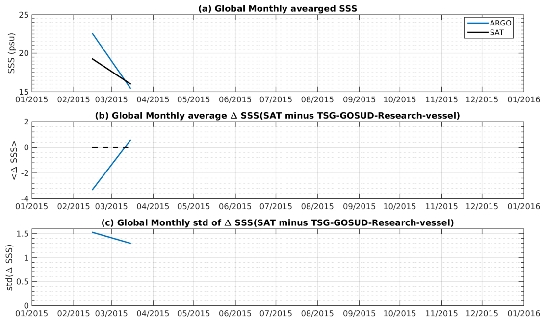
Figure 7: Time series of the monthly averaged mean SSS (top), mean \Delta SSS (Satellite - TSG-GOSUD-Research-vessel) and STD of \Delta SSS (Satellite - TSG-GOSUD-Research-vessel) over the Baltic Sea Pi-MEP region considering all match-ups collected by the Pi-MEP platform.
