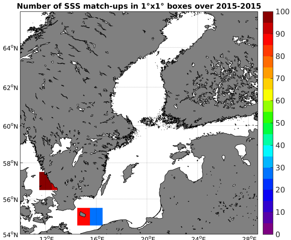
Figure 4: Number of SSS match-ups between TSG-GOSUD-Research-vessel SSS and the SMOS-L3-BEC-OA-V1-9DAYS-0.25DEG SSS product for the Baltic Sea Pi-MEP region over 1°x1° boxes and for the full satellite product period.
