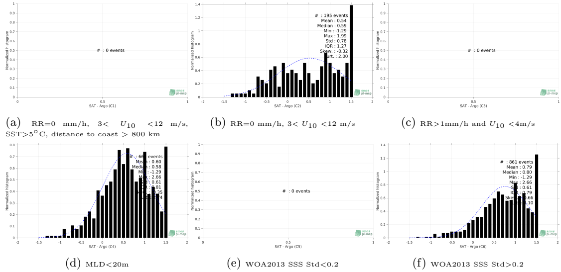
Figure 13: Normalized histogram of \Delta\text{SSS} (SMOS-L3-BEC-OA-V1-9DAYS-0.25DEG - Argo) for 6 different subdatasets corresponding to: RR=0 mm/h, 3 < U_{10} < 12 m/s, SST>5°C, distance to coast > 800 km (a), RR=0 mm/h, 3 < U_{10} < 12 m/s (b), RR>1mm/h and U_{10} < 4 m/s (c), MLD<20m (d), WOA2013 SSS Std<0.2 (e), WOA2013 SSS Std>0.2 (f).
