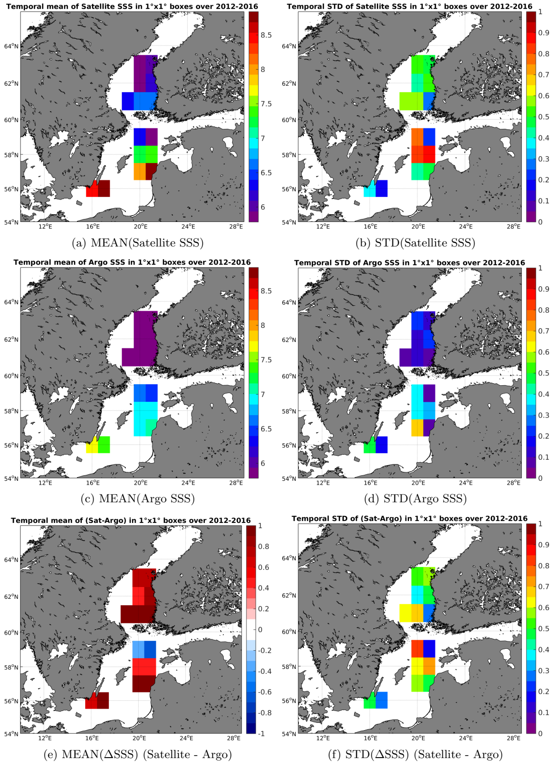
Figure 6: Temporal mean (left) and STD (right) of SSS from SMOS-L3-BEC-OA-V1-9DAYS-0.25DEG (top), Argo (middle), and of \Delta SSS (Satellite - Argo). Only match-up pairs are used to generate these maps.
