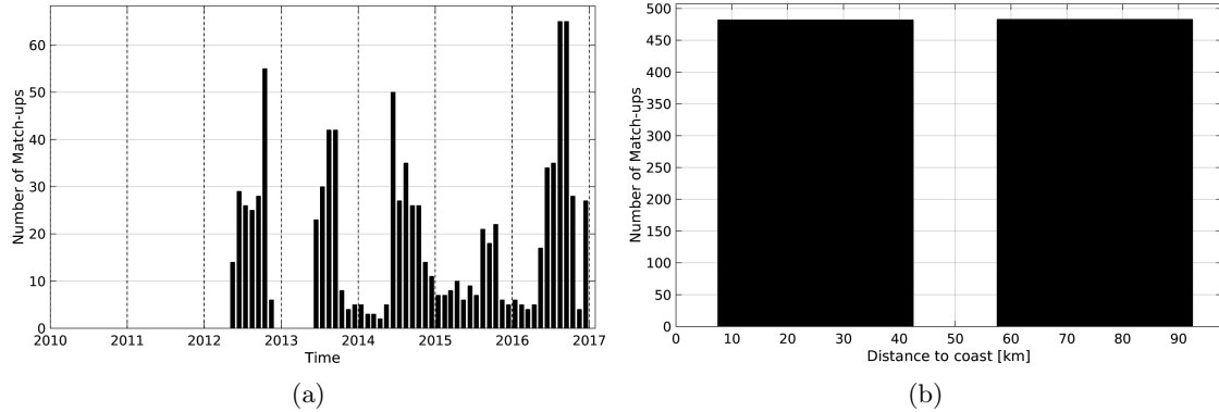
Figure 1: Number of match-ups between Argo and SMOS-L3-BEC-OA-V1-9DAYS-0.25DEG SSS as a function of time (a) and as function of the distance to coast (b) over the Baltic Sea Pi-MEP region and for the full satellite product period.
