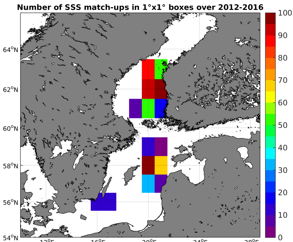
Figure 4: Number of SSS match-ups between Argo SSS and the SMOS-L3-BEC-OA-V1-9DAYS-0.25DEG SSS product for the Baltic Sea Pi-MEP region over 1°x1° boxes and for the full satellite product period.
