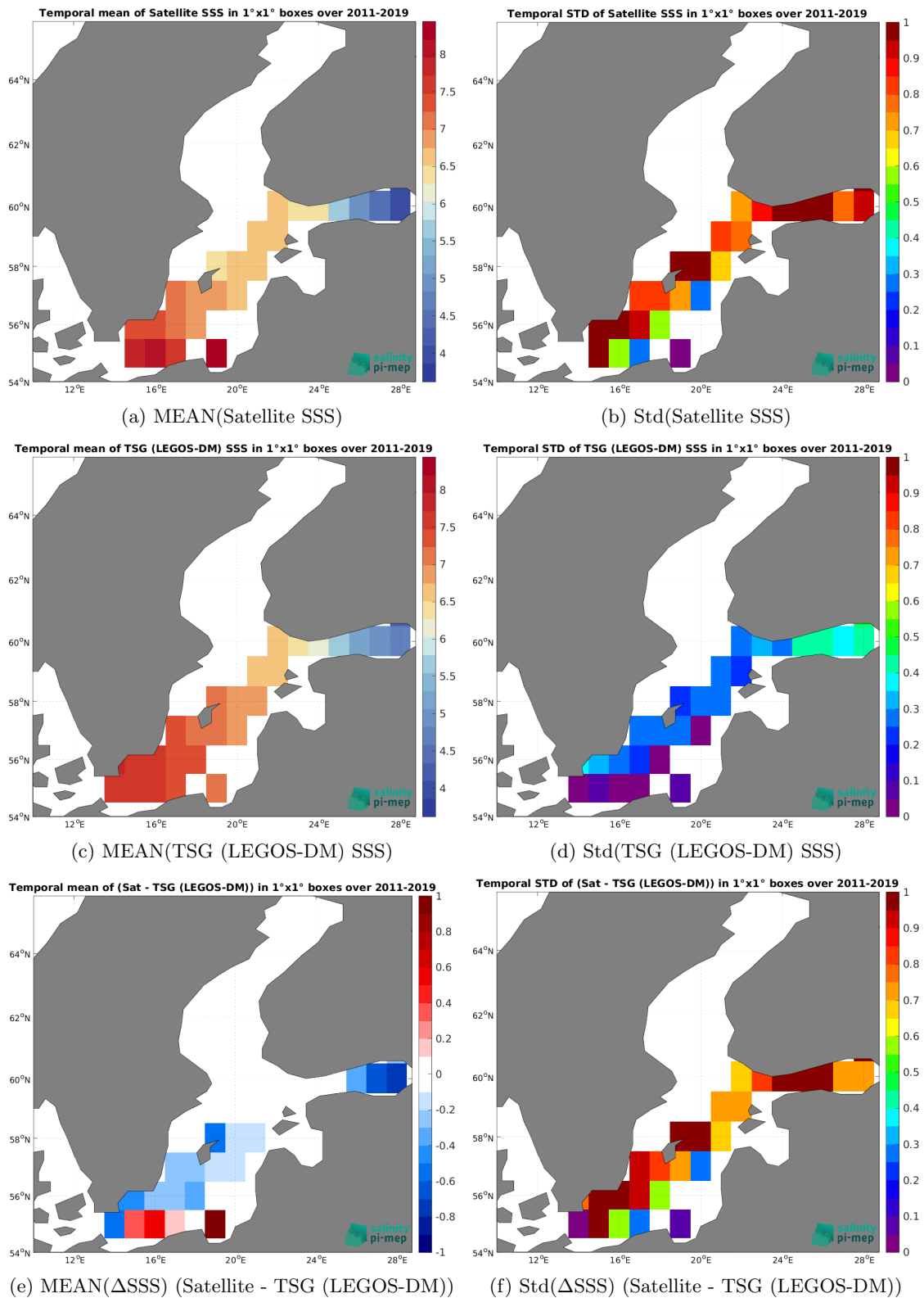
Figure 7: Temporal mean (left) and Std (right) of SSS from SMOS SSS L3 Baltic v1 - 9 Days (BEC) (top), TSG (LEGOS-DM) (middle), and \Delta SSS (Satellite - TSG (LEGOS-DM)). Only match-up pairs are used to generate these maps.
