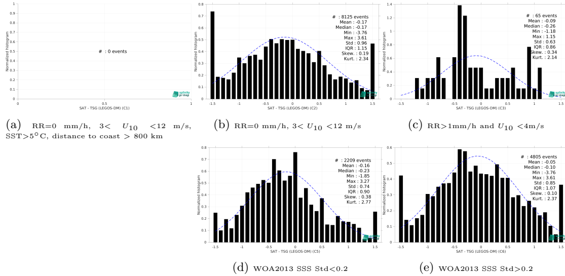
Figure 15: Normalized histogram of \Delta SSS (SMOS SSS L3 Baltic v1 - 9 Days (BEC) - TSG (LEGOS-DM)) for 5 different subdatasets corresponding to: RR=0 mm/h, 3 < U_{10} < 12 m/s, SST > 5°C, distance to coast > 800 km (a), RR=0 mm/h, 3 < U_{10} < 12 m/s (b), RR > 1mm/h and U_{10} < 4 m/s (c), WOA2013 SSS Std < 0.2 (d), WOA2013 SSS Std > 0.2 (e).
