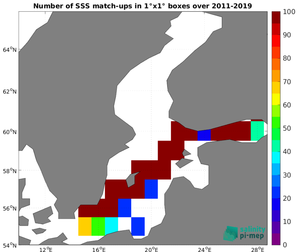
Figure 5: Number of SSS match-ups between TSG (LEGOS-DM) SSS and the SMOS SSS L3 Baltic v1 - 9 Days (BEC) SSS product for the Baltic Sea Pi-MEP region over 1°x1° boxes and for the full satellite product period.
