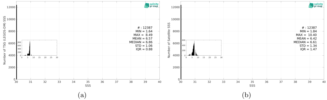
Figure 3: Histograms of SSS from TSG (LEGOS-DM) (a) and SMOS SSS L3 Baltic v1 - 9 Days (BEC) (b) considering all match-up pairs per bins of 0.1 over the Baltic Sea Pi-MEP region and for the full satellite product period.
