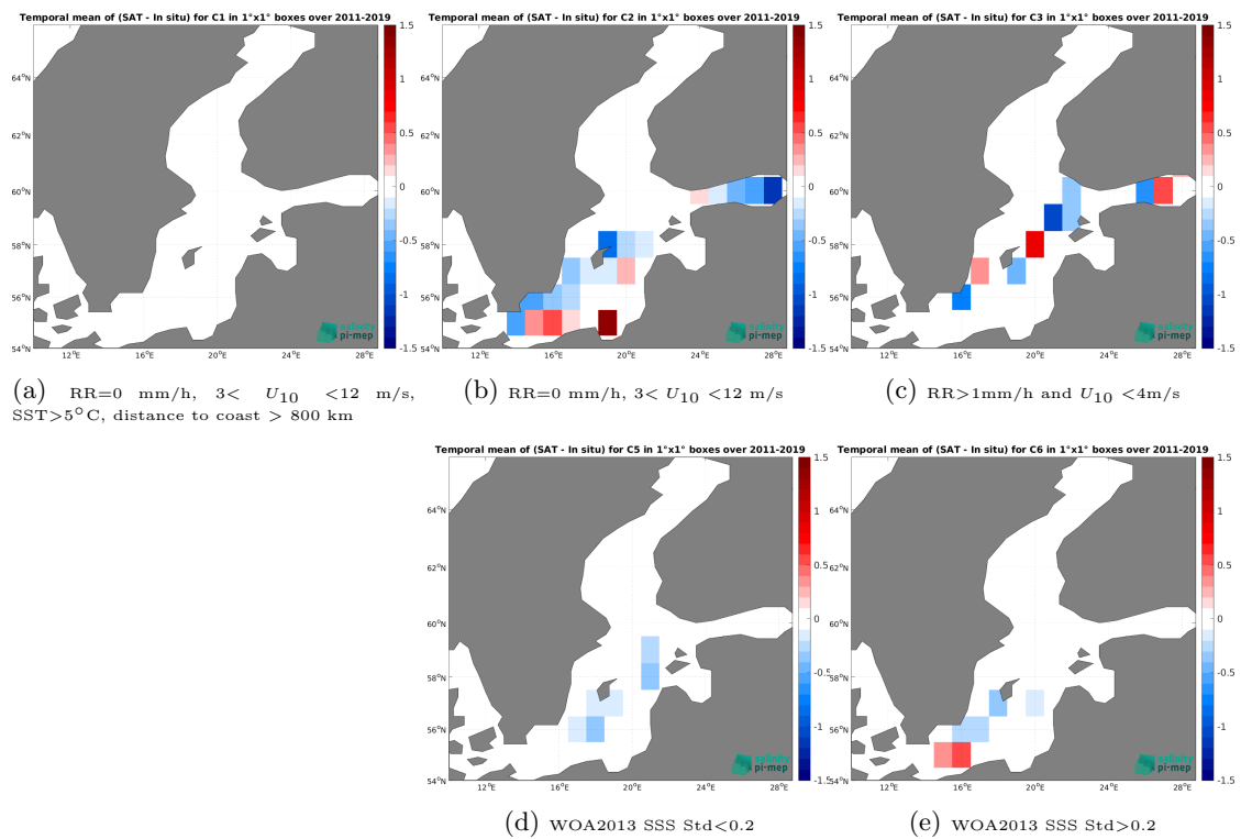
Figure 14: Temporal mean gridded over spatial boxes of size 1^\circ \times 1^\circ of \Delta SSS (SMOS SSS L3 Baltic v1 - 9 Days (BEC) - TSG (LEGOS-DM)) for 5 different subdatasets corresponding to:RR=0 mm/h, 3 < U_{10} < 12 m/s, SST >5^\circ C, distance to coast > 800 km (a), RR=0 mm/h, 3 < U_{10} < 12 m/s (b), RR >1 mm/h and U_{10} < 4 m/s (c), WOA2013 SSS Std <0.2 (d), WOA2013 SSS Std >0.2 (e).
