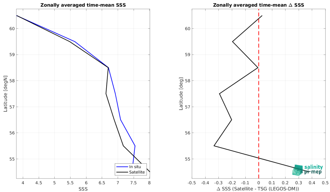
Figure 9: Left panel: Zonal mean SSS from SMOS SSS L3 Baltic v1 - 9 Days (BEC) satellite product (black) and from TSG (LEGOS-DM) (blue). Right panel: Zonal mean of \Delta SSS (Satellite - TSG (LEGOS-DM)) for all the collected Pi-MEP match-up pairs estimated over the full satellite product period.
