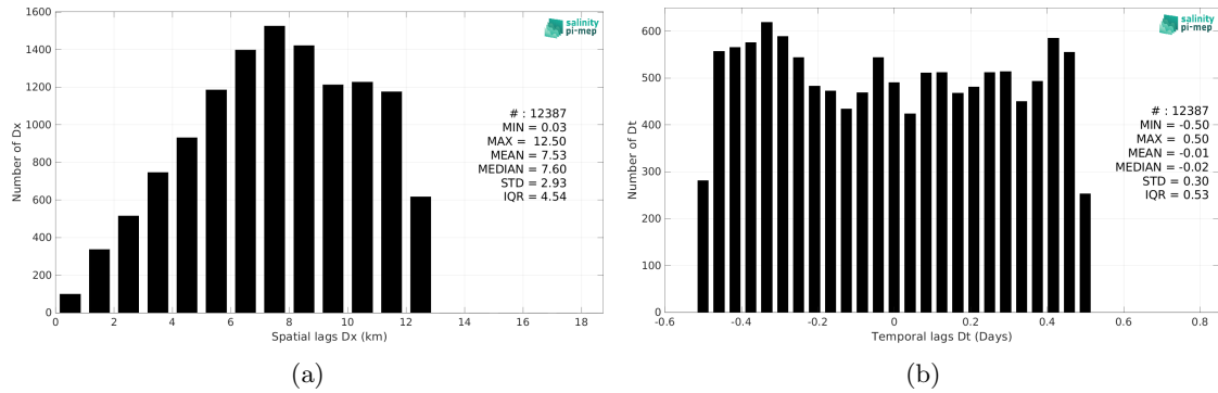
Figure 6: Histograms of the spatial (a) and temporal (b) lags between the location/time of the TSG (LEGOS-DM) measurement and the date of the corresponding SMOS SSS L3 Baltic v1 - 9 Days (BEC) SSS pixel.
