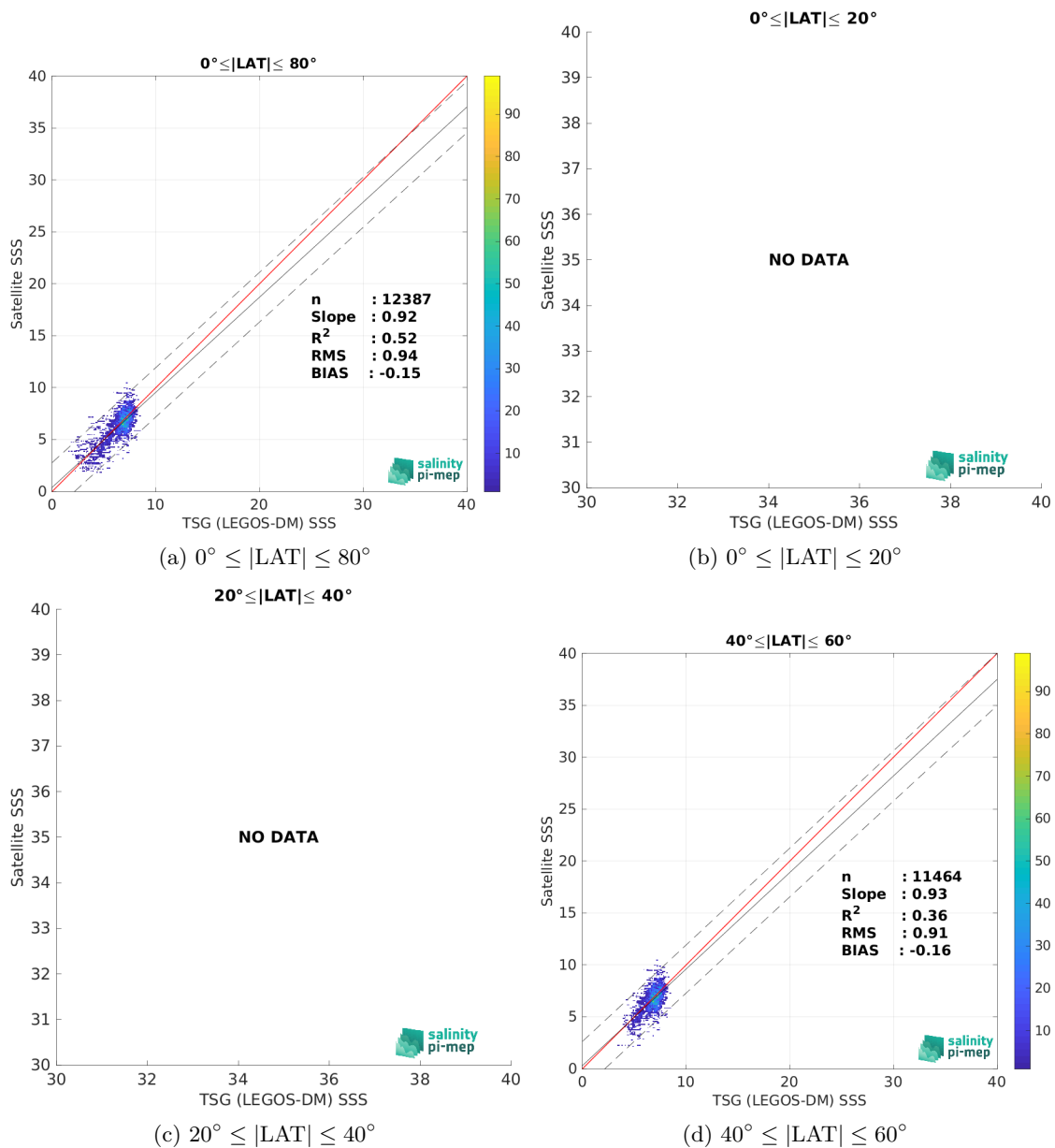
Figure 10: Contour maps of the concentration of SMOS SSS L3 Baltic v1 - 9 Days (BEC) SSS (y-axis) versus TSG (LEGOS-DM) SSS (x-axis) at match-up pairs for different latitude bands. For each plot, the red line shows x=y . The black thin and dashed lines indicate a linear fit through the data cloud and the \pm 95\% confidence levels, respectively. The number match-up pairs n , the slope and R^2 coefficient of the linear fit, the root mean square (RMS) and the mean bias between satellite and in situ data are indicated for each latitude band in each plots.
