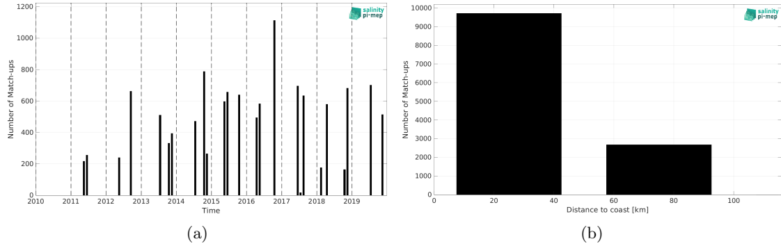
Figure 2: Number of match-ups between TSG (LEGOS-DM) and SMOS SSS L3 Baltic v1 - 9 Days (BEC) SSS as a function of time (a) and as function of the distance to coast (b) over the Baltic Sea Pi-MEP region and for the full satellite product period.
