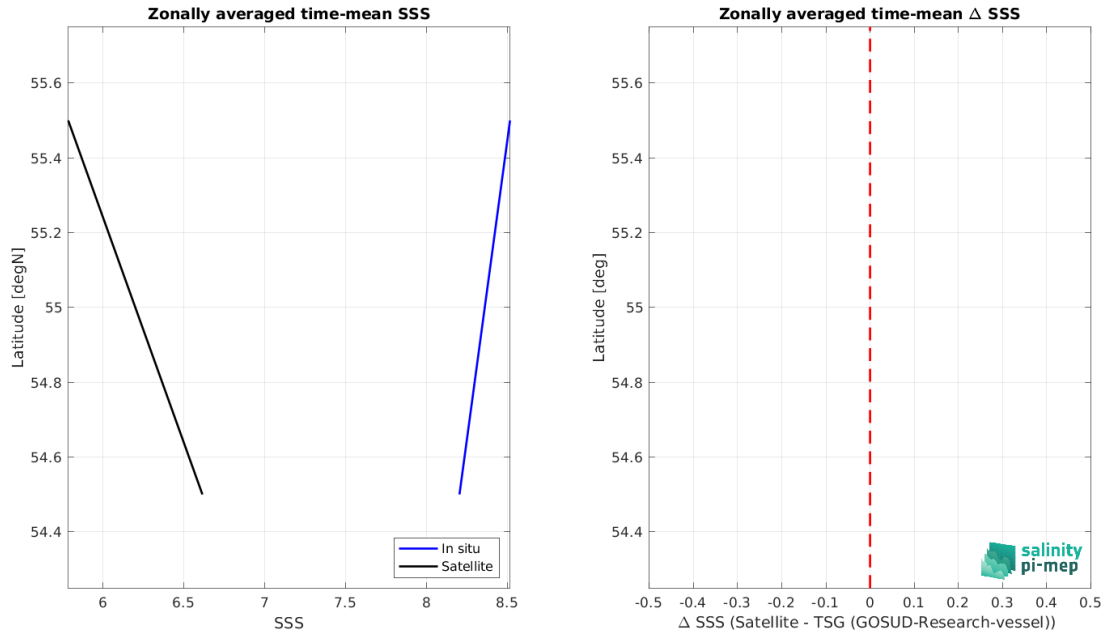
Figure 9: Left panel: Zonal mean SSS from SMOS SSS L3 Baltic v1 - 9 Days (BEC) satellite product (black) and from TSG (GOSUD-Research-vessel) (blue). Right panel: Zonal mean of \Delta SSS (Satellite - TSG (GOSUD-Research-vessel)) for all the collected Pi-MEP match-up pairs estimated over the full satellite product period.
