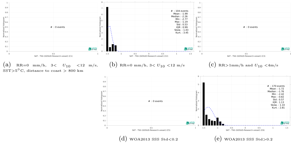
Figure 15: Normalized histogram of \Delta SSS (SMOS SSS L3 Baltic v1 - 9 Days (BEC) - TSG (GOSUD-Research-vessel)) for 5 different subdatasets corresponding to: RR=0 mm/h, 3 < U_{10} < 12 m/s, SST > 5°C, distance to coast > 800 km (a), RR=0 mm/h, 3 < U_{10} < 12 m/s (b), RR > 1mm/h and U_{10} < 4 m/s (c), WOA2013 SSS Std < 0.2 (d), WOA2013 SSS Std > 0.2 (e).
