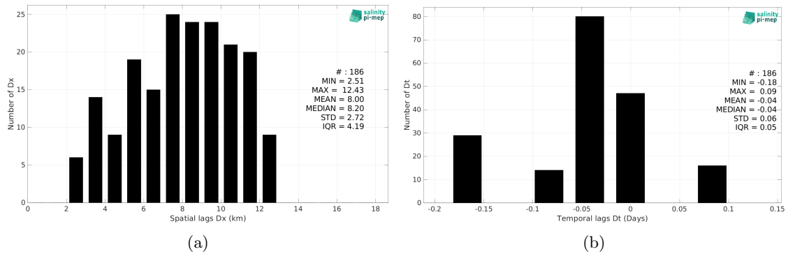
Figure 6: Histograms of the spatial (a) and temporal (b) lags between the location/time of the TSG (GOSUD-Research-vessel) measurement and the date of the corresponding SMOS SSS L3 Baltic v1 - 9 Days (BEC) SSS pixel.
