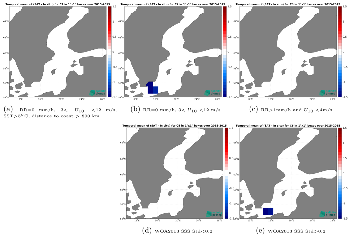
Figure 14: Temporal mean gridded over spatial boxes of size 1^\circ \times 1^\circ of \Delta\text{SSS} (SMOS SSS L3 Baltic v1 - 9 Days (BEC) - TSG (GOSUD-Research-vessel)) for 5 different subdatasets corresponding to:RR=0 mm/h, 3 < U_{10} < 12 m/s, SST>5°C, distance to coast > 800 km (a), RR=0 mm/h, 3 < U_{10} < 12 m/s (b), RR>1mm/h and U_{10} < 4 m/s (c), WOA2013 SSS Std<0.2 (d), WOA2013 SSS Std>0.2 (e).
