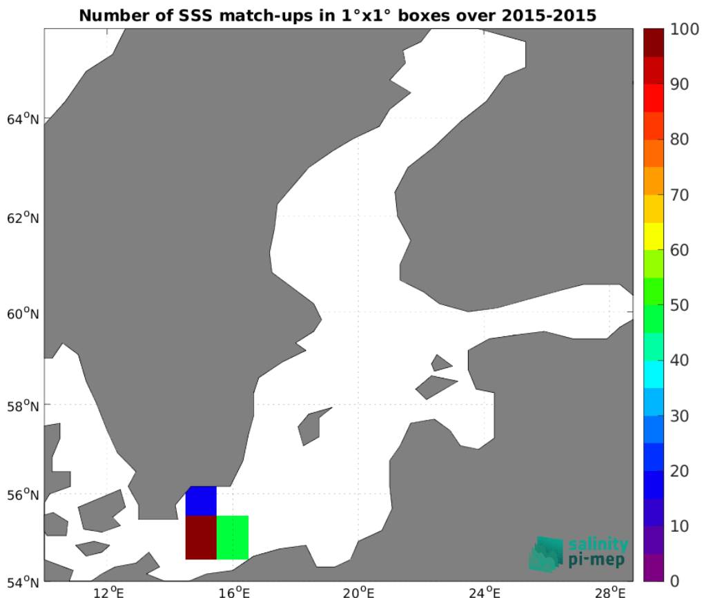
Figure 5: Number of SSS match-ups between TSG (GOSUD-Research-vessel) SSS and the SMOS SSS L3 Baltic v1 - 9 Days (BEC) SSS product for the Baltic Sea Pi-MEP region over 1°x1° boxes and for the full satellite product period.
