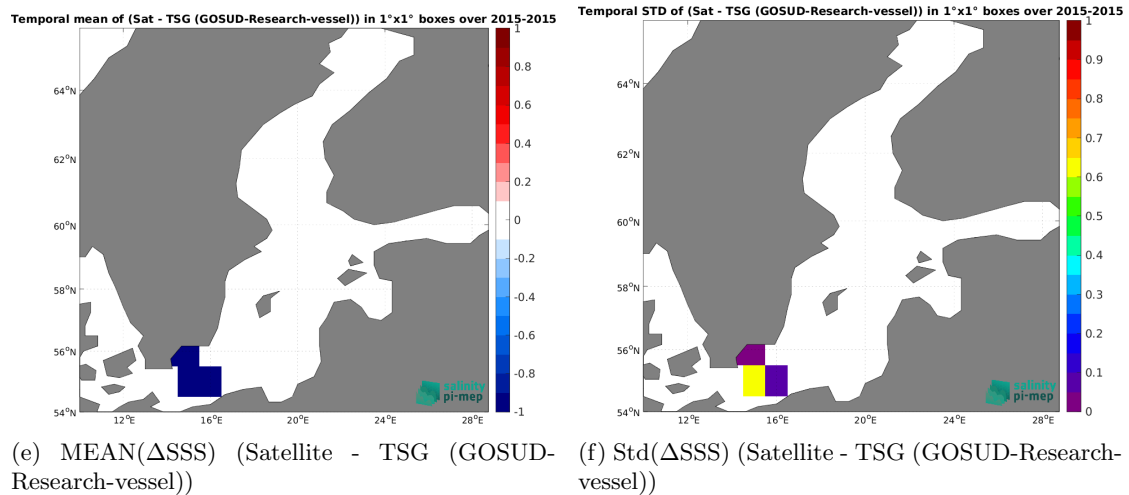
Figure 7: Temporal mean (left) and Std (right) of SSS from SMOS SSS L3 Baltic v1 - 9 Days (BEC) (top), TSG (GOSUD-Research-vessel) (middle), and of \Delta SSS (Satellite - TSG (GOSUD-Research-vessel)). Only match-up pairs are used to generate these maps.
