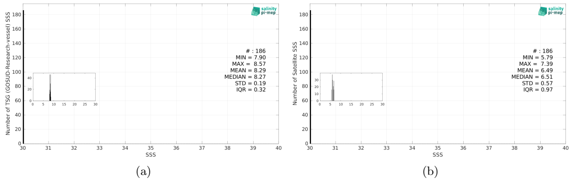
Figure 3: Histograms of SSS from TSG (GOSUD-Research-vessel) (a) and SMOS SSS L3 Baltic v1 - 9 Days (BEC) (b) considering all match-up pairs per bins of 0.1 over the Baltic Sea Pi-MEP region and for the full satellite product period.
