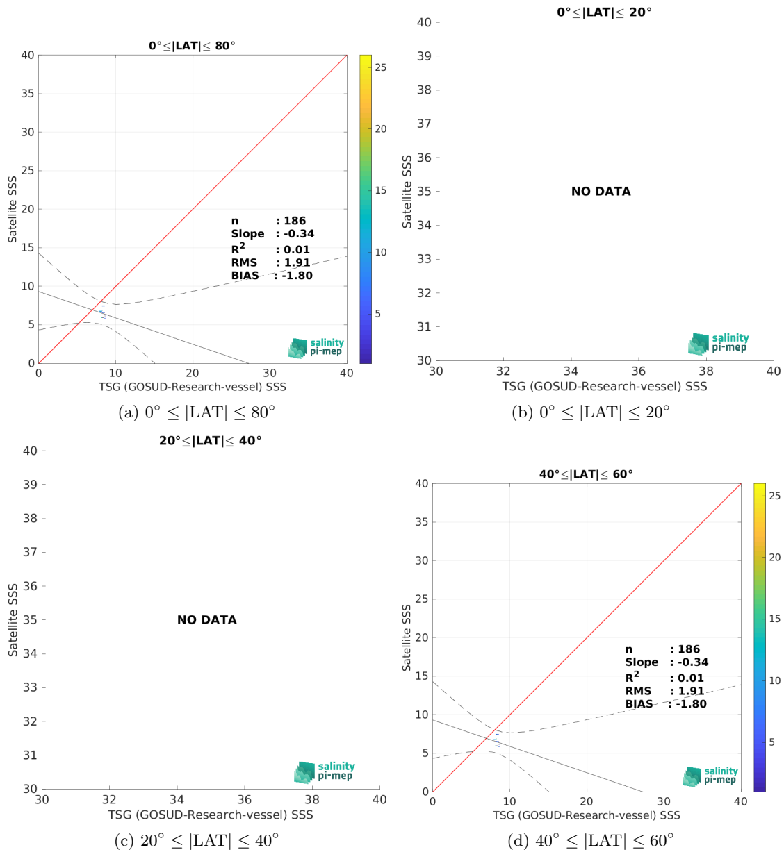
Figure 10: Contour maps of the concentration of SMOS SSS L3 Baltic v1 - 9 Days (BEC) SSS (y-axis) versus TSG (GOSUD-Research-vessel) SSS (x-axis) at match-up pairs for different latitude bands. For each plot, the red line shows x=y . The black thin and dashed lines indicate a linear fit through the data cloud and the \pm 95\% confidence levels, respectively. The number match-up pairs n , the slope and R^2 coefficient of the linear fit, the root mean square (RMS) and the mean bias between satellite and in situ data are indicated for each latitude band in each plot.
