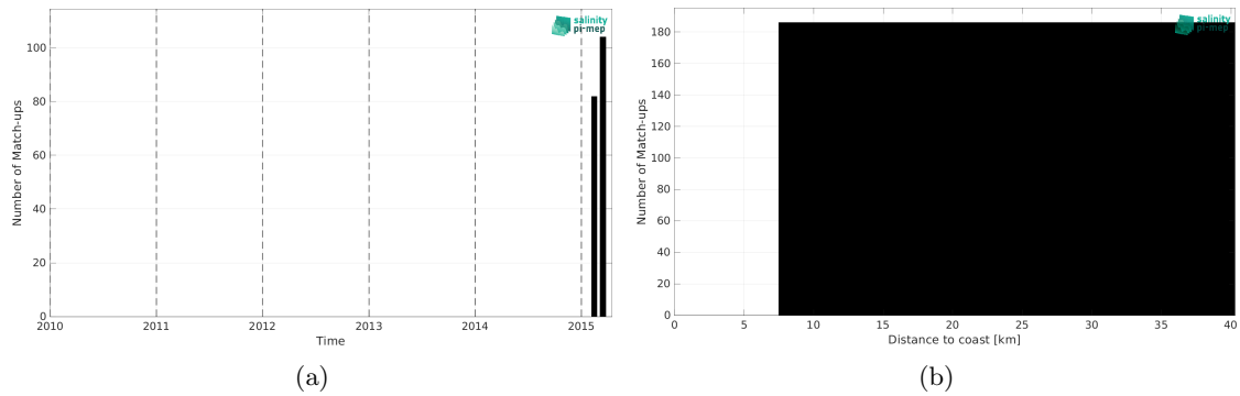
Figure 2: Number of match-ups between TSG (GOSUD-Research-vessel) and SMOS SSS L3 Baltic v1 - 9 Days (BEC) SSS as a function of time (a) and as function of the distance to coast (b) over the Baltic Sea Pi-MEP region and for the full satellite product period.
