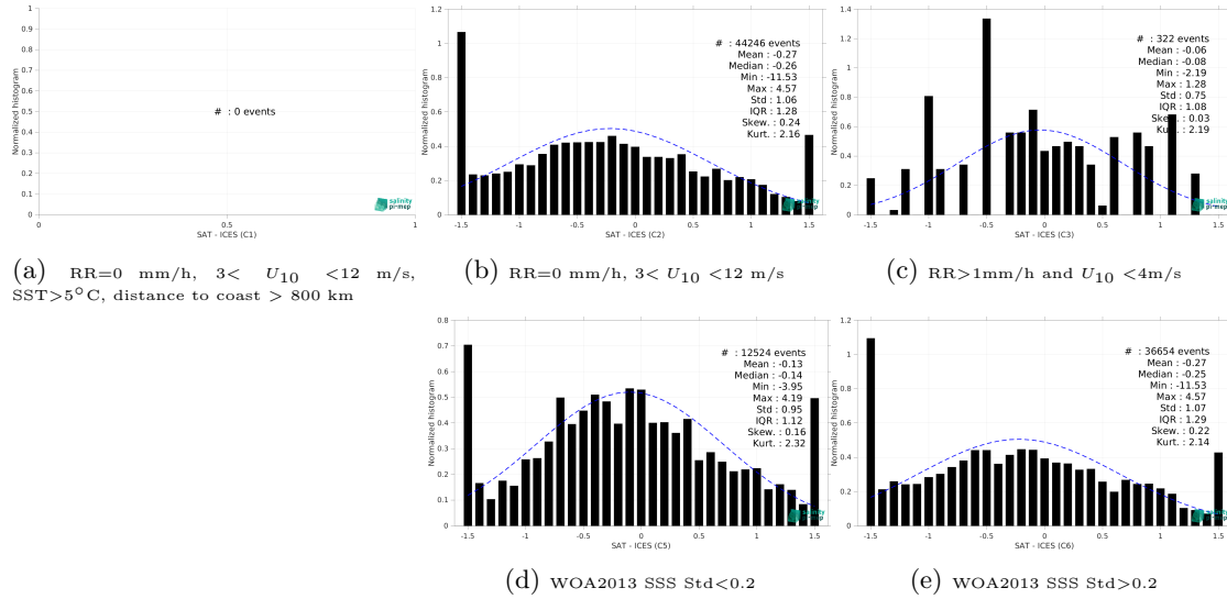
Figure 15: Normalized histogram of \Delta SSS (SMOS SSS L3 Baltic v1 - 9 Days (BEC) - ICES) for 5 different subdatasets corresponding to: RR=0 mm/h, 3 < U_{10} < 12 m/s, SST > 5°C, distance to coast > 800 km (a), RR=0 mm/h, 3 < U_{10} < 12 m/s (b), RR > 1mm/h and U_{10} < 4 m/s (c), WOA2013 SSS Std < 0.2 (d), WOA2013 SSS Std > 0.2 (e).
