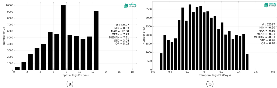
Figure 6: Histograms of the spatial (a) and temporal (b) lags between the location/time of the ICES measurement and the date of the corresponding SMOS SSS L3 Baltic v1 - 9 Days (BEC) SSS pixel.
