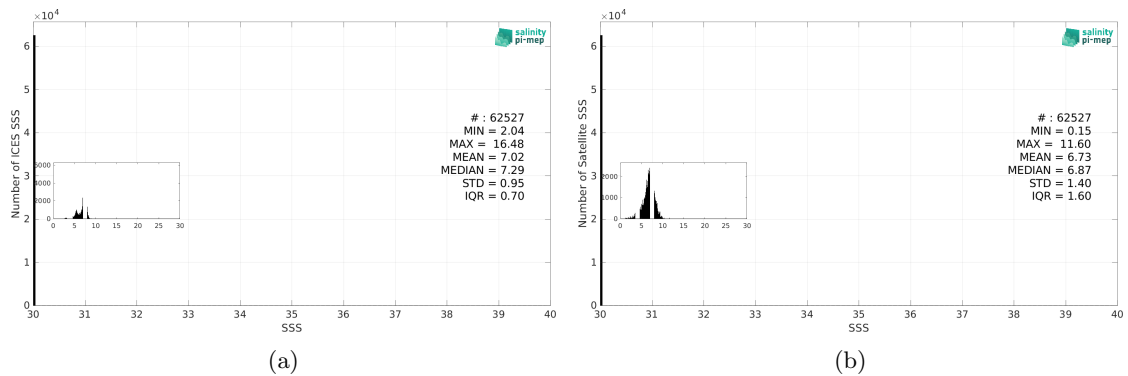
Figure 3: Histograms of SSS from ICES (a) and SMOS SSS L3 Baltic v1 - 9 Days (BEC) (b) considering all match-up pairs per bins of 0.1 over the Baltic Sea Pi-MEP region and for the full satellite product period.
