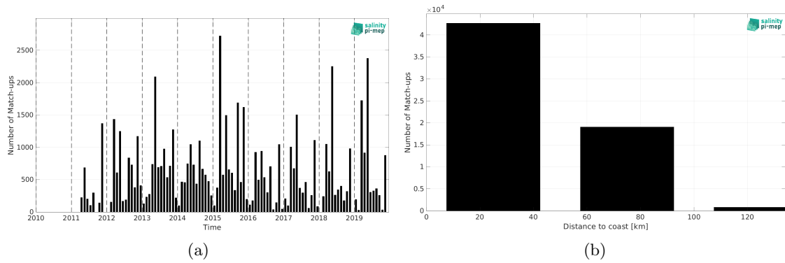
Figure 2: Number of match-ups between ICES and SMOS SSS L3 Baltic v1 - 9 Days (BEC) SSS as a function of time (a) and as function of the distance to coast (b) over the Baltic Sea Pi-MEP region and for the full satellite product period.
