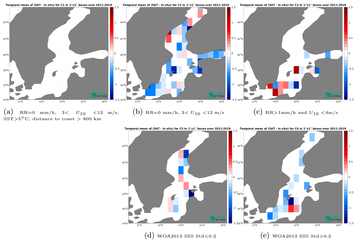
Figure 14: Temporal mean gridded over spatial boxes of size 1^\circ \times 1^\circ of \Delta SSS (SMOS SSS L3 Baltic v1 - 9 Days (BEC) - ICES) for 5 different subdatasets corresponding to:RR=0 mm/h, 3 < U_{10} < 12 m/s, SST >5^\circ\text{C} , distance to coast > 800 km (a), RR=0 mm/h, 3 < U_{10} < 12 m/s (b), RR >1 mm/h and U_{10} < 4 m/s (c), WOA2013 SSS Std <0.2 (d), WOA2013 SSS Std >0.2 (e).
