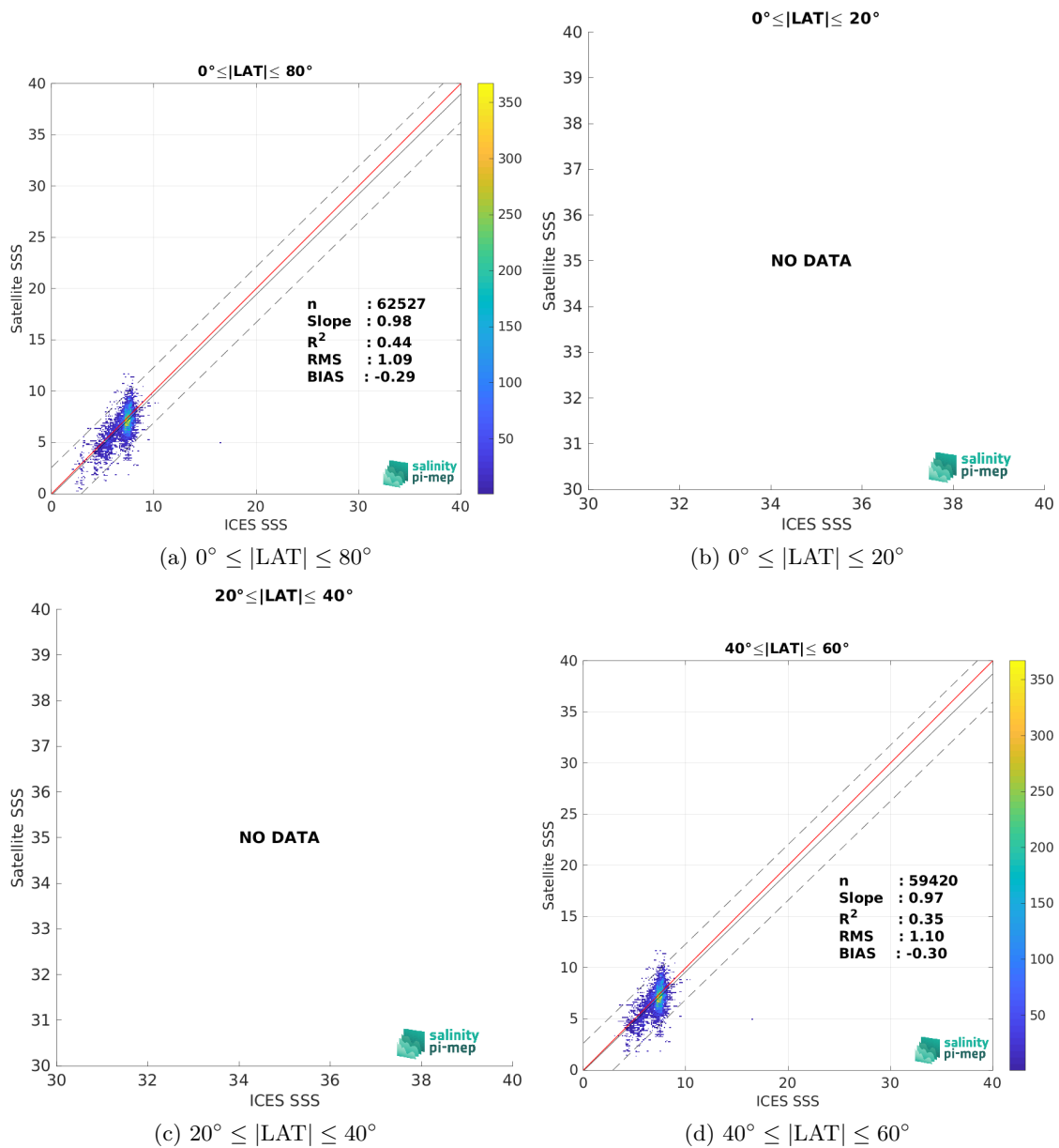
Figure 10: Contour maps of the concentration of SMOS SSS L3 Baltic v1 - 9 Days (BEC) SSS (y-axis) versus ICES SSS (x-axis) at match-up pairs for different latitude bands. For each plot, the red line shows x=y . The black thin and dashed lines indicate a linear fit through the data cloud and the \pm 95\% confidence levels, respectively. The number match-up pairs n , the slope and R^2 coefficient of the linear fit, the root mean square (RMS) and the mean bias between satellite and in situ data are indicated for each latitude band in each plots.
