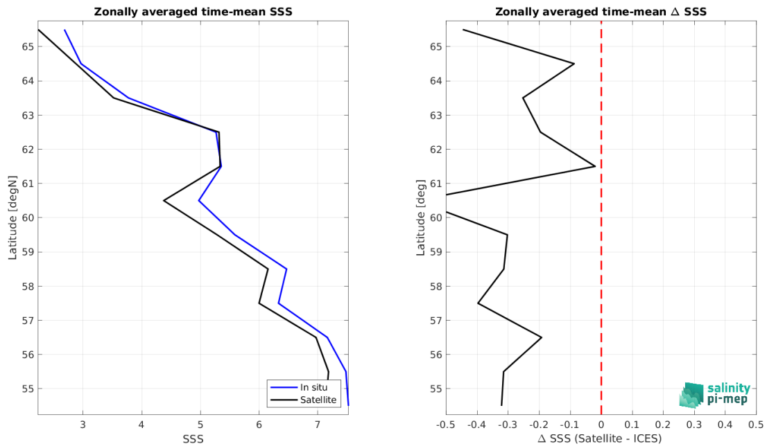
Figure 9: Left panel: Zonal mean SSS from SMOS SSS L3 Baltic v1 - 9 Days (BEC) satellite product (black) and from ICES (blue). Right panel: Zonal mean of \Delta SSS (Satellite - ICES) for all the collected Pi-MEP match-up pairs estimated over the full satellite product period.
