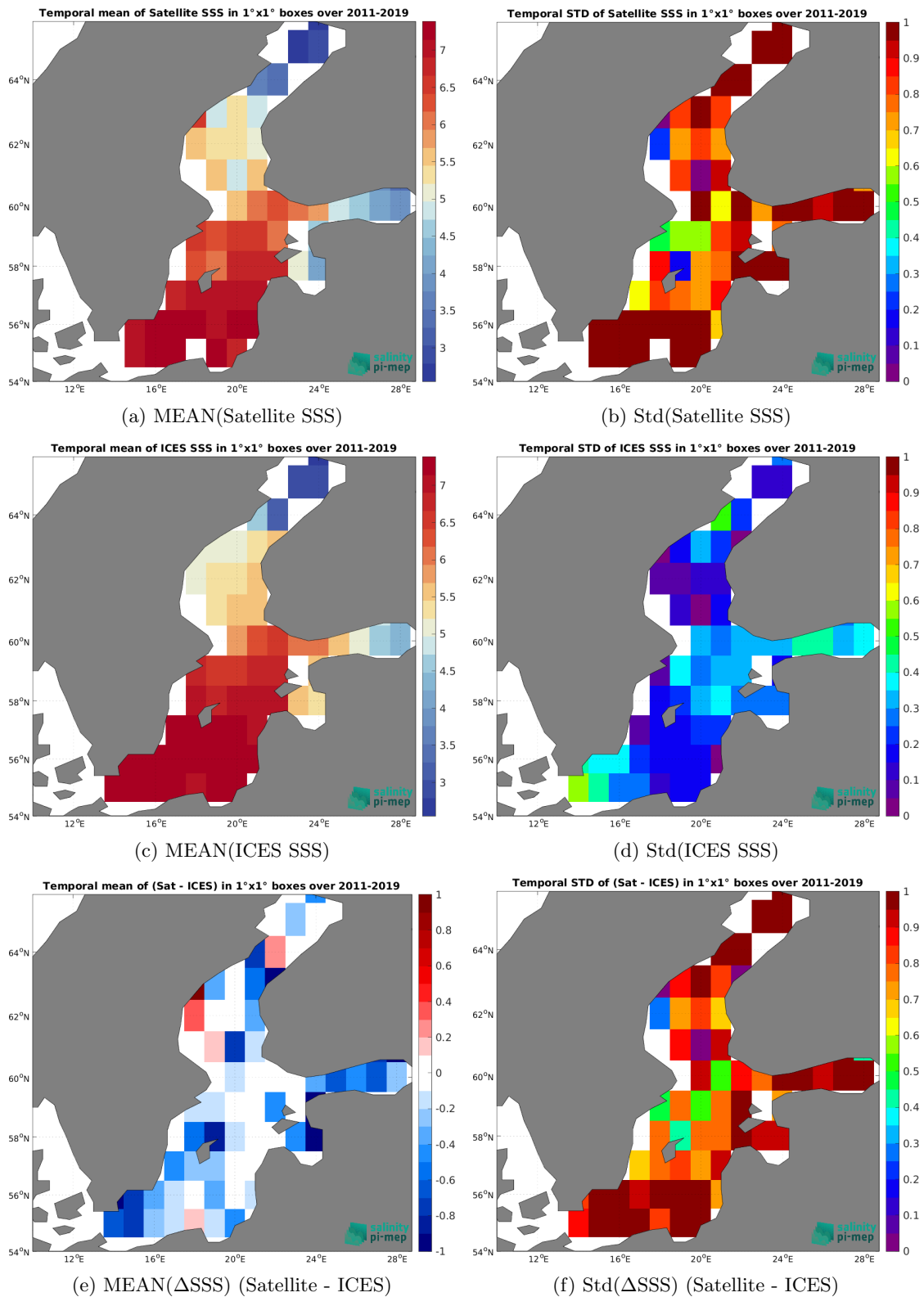
Figure 7: Temporal mean (left) and Std (right) of SSS from SMOS SSS L3 Baltic v1 - 9 Days (BEC) (top), ICES (middle), and of \Delta SSS (Satellite - ICES). Only match-up pairs are used to generate these maps.
