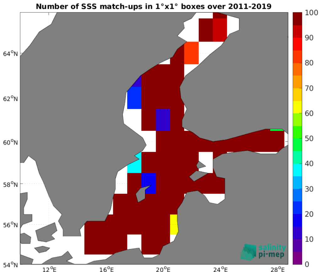
Figure 5: Number of SSS match-ups between ICES SSS and the SMOS SSS L3 Baltic v1 - 9 Days (BEC) SSS product for the Baltic Sea Pi-MEP region over 1°x1° boxes and for the full satellite product period.
