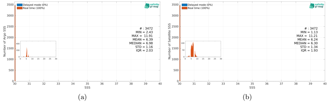
Figure 3: Histograms of SSS from Argo (a) and SMOS SSS L3 Baltic v1 - 9 Days (BEC) (b) considering all match-up pairs per bins of 0.1 over the Baltic Sea Pi-MEP region and for the full satellite product period.
