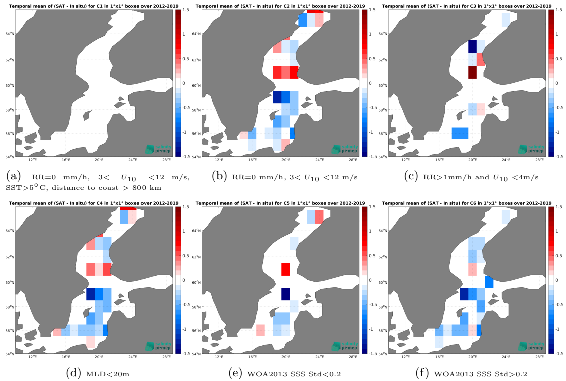
Figure 14: Temporal mean gridded over spatial boxes of size 1^\circ \times 1^\circ of \Delta SSS (SMOS SSS L3 Baltic v1 - 9 Days (BEC) - Argo) for 6 different subdatasets corresponding to:RR=0 mm/h, 3 < U_{10} < 12 m/s, SST>5°C, distance to coast > 800 km (a), RR=0 mm/h, 3 < U_{10} < 12 m/s (b), RR>1mm/h and U_{10} < 4 m/s (c),MLD<20m (d),WOA2013 SSS Std<0.2 (e),WOA2013 SSS Std>0.2 (f).
