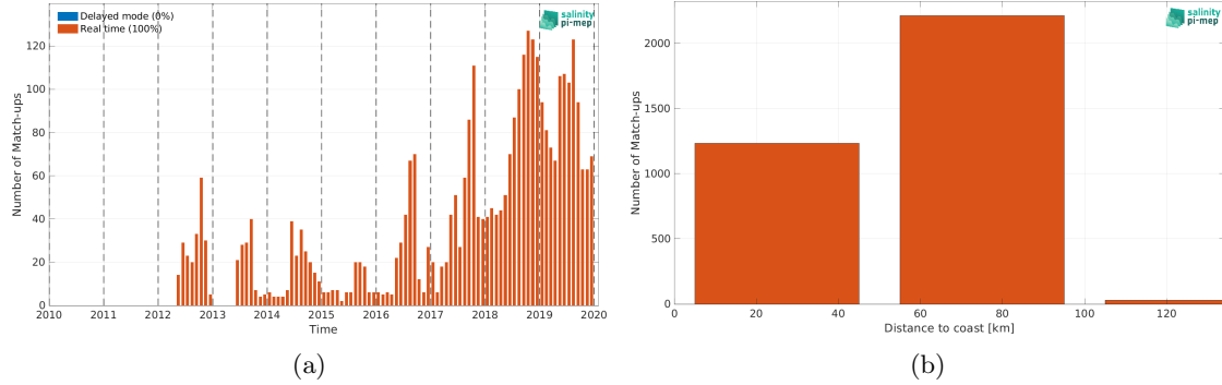
Figure 2: Number of match-ups between Argo and SMOS SSS L3 Baltic v1 - 9 Days (BEC) SSS as a function of time (a) and as function of the distance to coast (b) over the Baltic Sea Pi-MEP region and for the full satellite product period.
