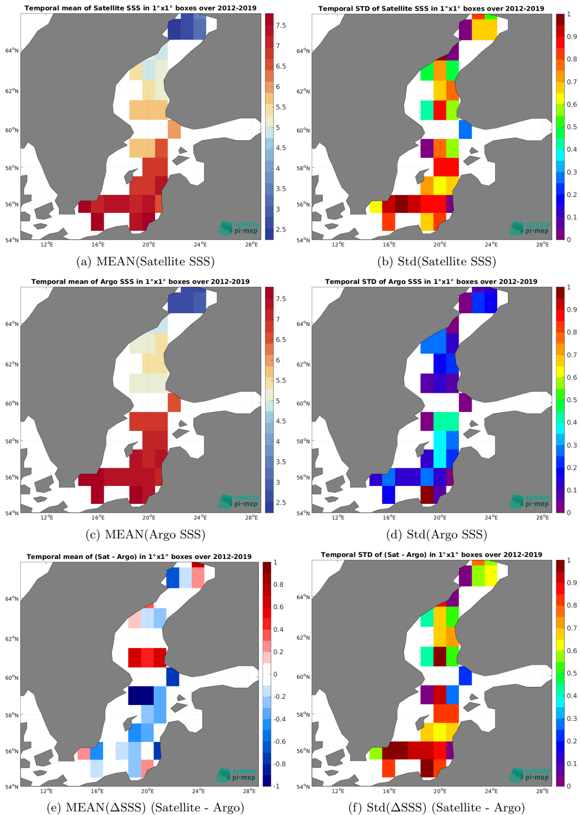
Figure 7: Temporal mean (left) and Std (right) of SSS from SMOS SSS L3 Baltic v1 - 9 Days (BEC) (top), Argo (middle), and of \Delta SSS (Satellite - Argo). Only match-up pairs are used to generate these maps.
