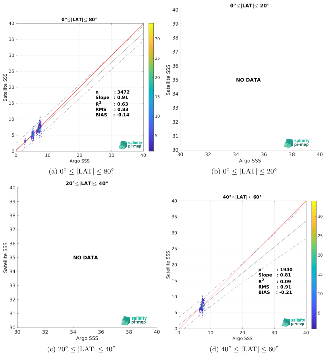
Figure 10: Contour maps of the concentration of SMOS SSS L3 Baltic v1 - 9 Days (BEC) SSS (y-axis) versus Argo SSS (x-axis) at match-up pairs for different latitude bands. For each plot, the red line shows x=y . The black thin and dashed lines indicate a linear fit through the data cloud and the \pm 95\% confidence levels, respectively. The number match-up pairs n , the slope and R^2 coefficient of the linear fit, the root mean square (RMS) and the mean bias between satellite and in situ data are indicated for each latitude band in each plots.
