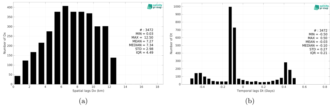
Figure 6: Histograms of the spatial (a) and temporal (b) lags between the location/time of the Argo measurement and the date of the corresponding SMOS SSS L3 Baltic v1 - 9 Days (BEC) SSS pixel.
