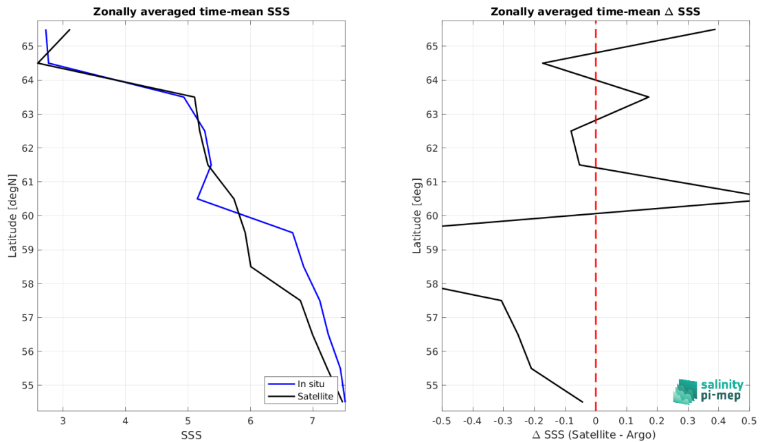
Figure 9: Left panel: Zonal mean SSS from SMOS SSS L3 Baltic v1 - 9 Days (BEC) satellite product (black) and from Argo (blue). Right panel: Zonal mean of \Delta SSS (Satellite - Argo) for all the collected Pi-MEP match-up pairs estimated over the full satellite product period.
