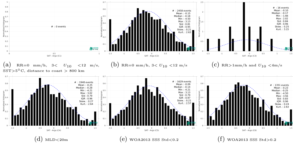
Figure 15: Normalized histogram of \Delta SSS (SMOS SSS L3 Baltic v1 - 9 Days (BEC) - Argo) for 6 different subdatasets corresponding to: RR=0 mm/h, 3 < U_{10} < 12 m/s, SST>5°C, distance to coast > 800 km (a), RR=0 mm/h, 3 < U_{10} < 12 m/s (b), RR>1mm/h and U_{10} < 4 m/s (c), MLD<20m (d), WOA2013 SSS Std<0.2 (e), WOA2013 SSS Std>0.2 (f).
