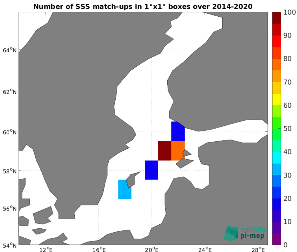
Figure 4: Number of SSS match-ups between TSG (LEGOS-DM) SSS and the SMOS SSS L2 v700 (ESA) SSS product for the Baltic Sea Pi-MEP region over 1^{\circ} \times 1^{\circ} boxes and for the full satellite product period.
