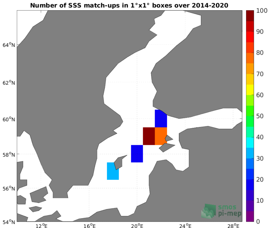
Figure 4: Number of SSS match-ups between TSG (LEGOS-DM) SSS and the SMOS SSS L2 v700 (ESA) SSS product for the Baltic Sea Pi-MEP region over 1°×1° boxes and for the full satellite product period.
