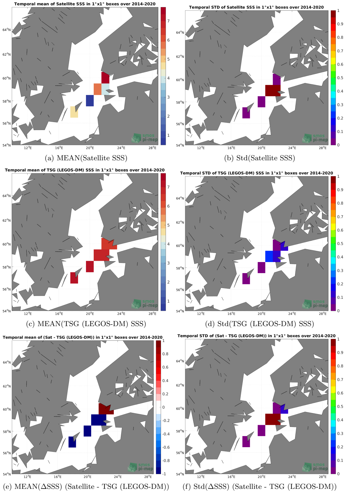
Figure 6: Temporal mean (left) and Std (right) of SSS from SMOS SSS L2 v700 (ESA) (top), TSG (LEGOS-DM) (middle), and of \Delta SSS (Satellite - TSG (LEGOS-DM)). Only match-up pairs are used to generate these maps.
