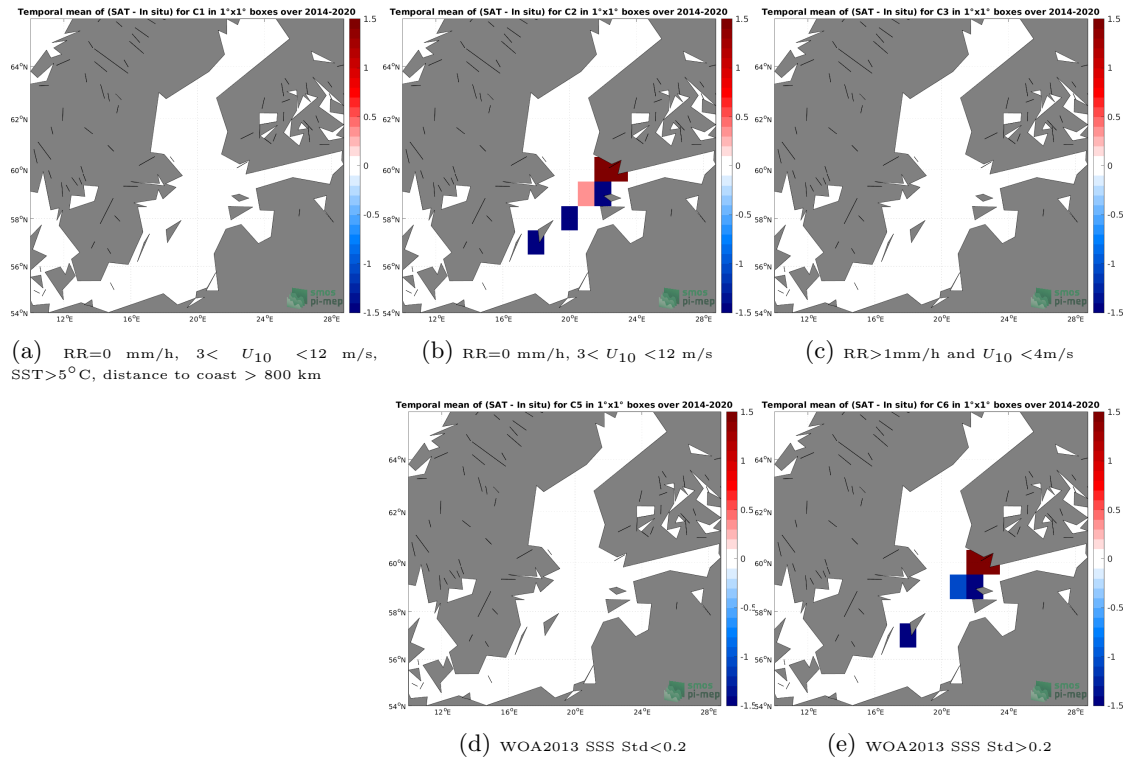
Figure 12: Temporal mean gridded over spatial boxes of size 1^{\circ}\times 1^{\circ} of \Delta\text{SSS} (SMOS SSS L2 v700 (ESA) - TSG (LEGOS-DM)) for 5 different subdatasets corresponding to: \text{RR}=0 mm/h, 3 < U_{10} < 12 m/s, \text{SST} > 5^{\circ}\text{C} , distance to coast > 800 km (a), \text{RR}=0 mm/h, 3 < U_{10} < 12 m/s (b), \text{RR} > 1\text{mm/h} and U_{10} < 4\text{m/s} (c), WOA2013 SSS Std < 0.2 (d), WOA2013 SSS Std > 0.2 (e).
