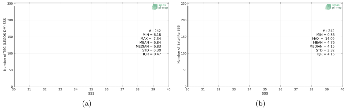
Figure 2: Histograms of SSS from TSG (LEGOS-DM) (a) and SMOS SSS L2 v700 (ESA) (b) considering all match-up pairs per bins of 0.1 over the Baltic Sea Pi-MEP region and for the full satellite product period.
