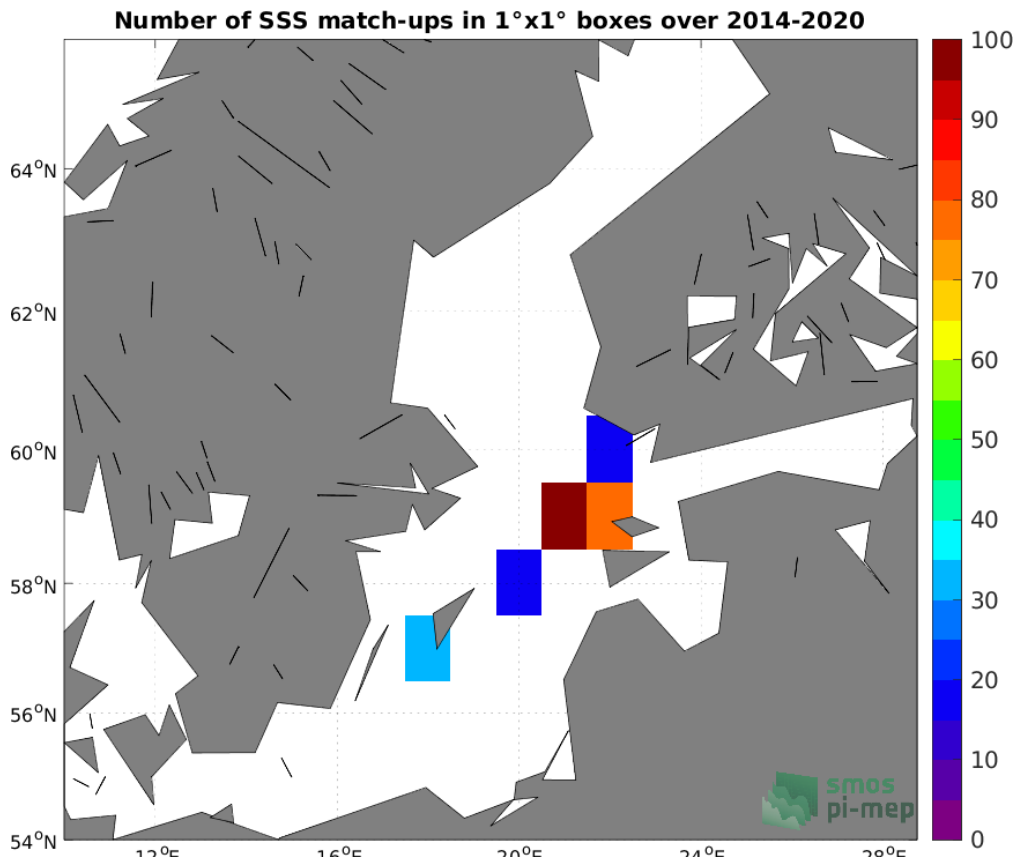
Figure 4: Number of SSS match-ups between TSG (LEGOS-DM) SSS and the SMOS SSS L2 v700 (ESA) SSS product for the Baltic Sea Pi-MEP region over 1°x1° boxes and for the full satellite product period.
