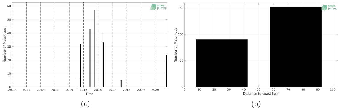
Figure 1: Number of match-ups between TSG (LEGOS-DM) and SMOS SSS L2 v700 (ESA) SSS as a function of time (a) and as function of the distance to coast (b) over the Baltic Sea Pi-MEP region and for the full satellite product period.
