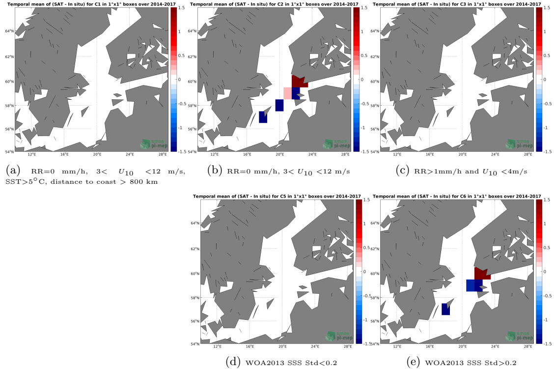
Figure 12: Temporal mean gridded over spatial boxes of size 1^{\circ}\times 1^{\circ} of \Delta\text{SSS} (SMOS SSS L2 v700 (ESA) - TSG (LEGOS-DM)) for 5 different subdatasets corresponding to:RR=0 mm/h, 3 < U_{10} < 12 m/s, SST >5^{\circ}\text{C} , distance to coast > 800 km (a), RR=0 mm/h, 3 < U_{10} < 12 m/s (b), RR >1 mm/h and U_{10} < 4 m/s (c), WOA2013 SSS Std <0.2 (d), WOA2013 SSS Std >0.2 (e).
