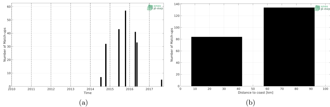
Figure 1: Number of match-ups between TSG (LEGOS-DM) and SMOS SSS L2 v700 (ESA) SSS as a function of time (a) and as function of the distance to coast (b) over the Baltic Sea Pi-MEP region and for the full satellite product period.
