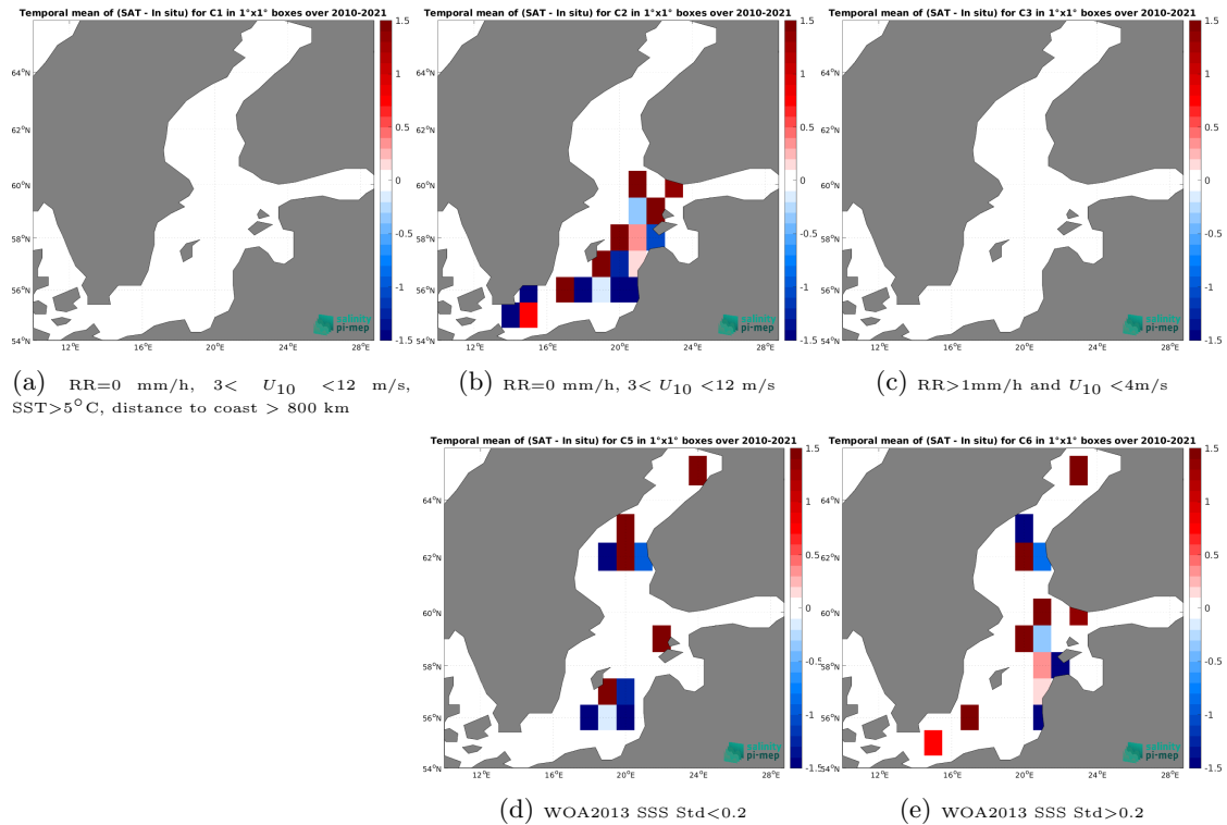
Figure 12: Temporal mean gridded over spatial boxes of size 1^{\circ}\times 1^{\circ} of \Delta\text{SSS} (SMOS SSS L2 v700 (ESA) - ICES) for 5 different subdatasets corresponding to:RR=0 mm/h, 3 < U_{10} < 12 m/s, SST > 5^{\circ}\text{C} , distance to coast > 800 km (a), RR=0 mm/h, 3 < U_{10} < 12 m/s (b), RR > 1 mm/h and U_{10} < 4 m/s (c), WOA2013 SSS Std < 0.2 (d), WOA2013 SSS Std > 0.2 (e).
