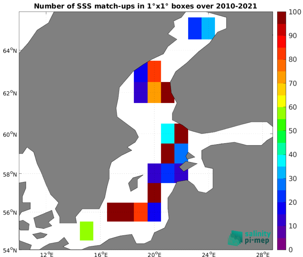
Figure 4: Number of SSS match-ups between ICES SSS and the SMOS SSS L2 v700 (ESA) SSS product for the Baltic Sea Pi-MEP region over 1°x1° boxes and for the full satellite product period.
