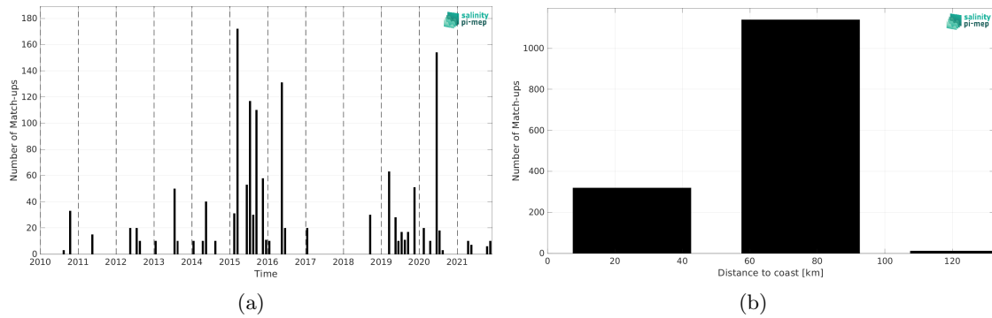
Figure 1: Number of match-ups between ICES and SMOS SSS L2 v700 (ESA) SSS as a function of time (a) and as function of the distance to coast (b) over the Baltic Sea Pi-MEP region and for the full satellite product period.
