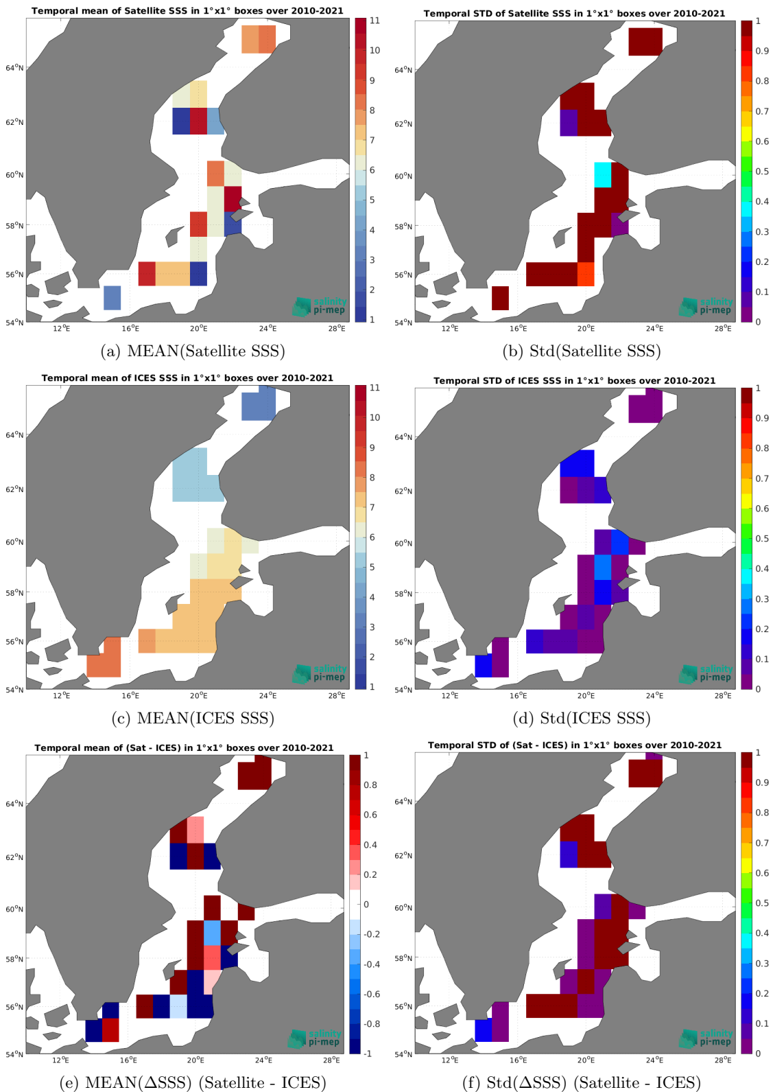
Figure 6: Temporal mean (left) and Std (right) of SSS from SMOS SSS L2 v700 (ESA) (top), ICES (middle), and of \Delta SSS (Satellite - ICES) (bottom). Only match-up pairs are used to generate these maps.
