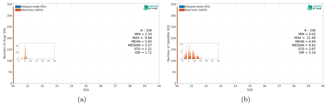
Figure 3: Histograms of SSS from Argo (a) and SMOS SSS L2 v700 (ESA) (b) considering all match-up pairs per bins of 0.1 over the Baltic Sea Pi-MEP region and for the full satellite product period.
