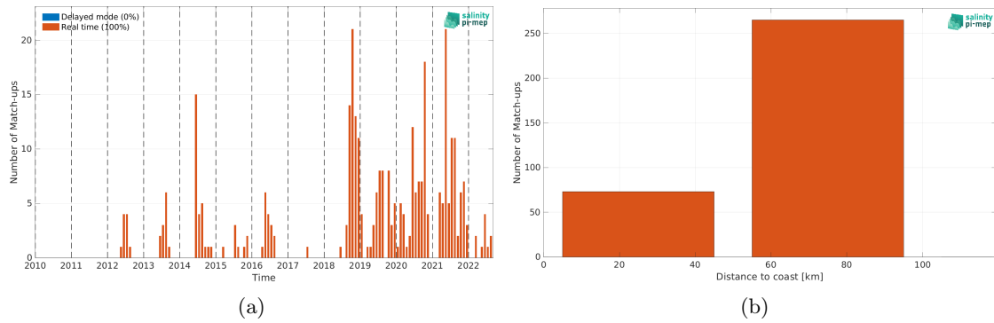
Figure 2: Number of match-ups between Argo and SMOS SSS L2 v700 (ESA) SSS as a function of time (a) and as function of the distance to coast (b) over the Baltic Sea Pi-MEP region and for the full satellite product period.
