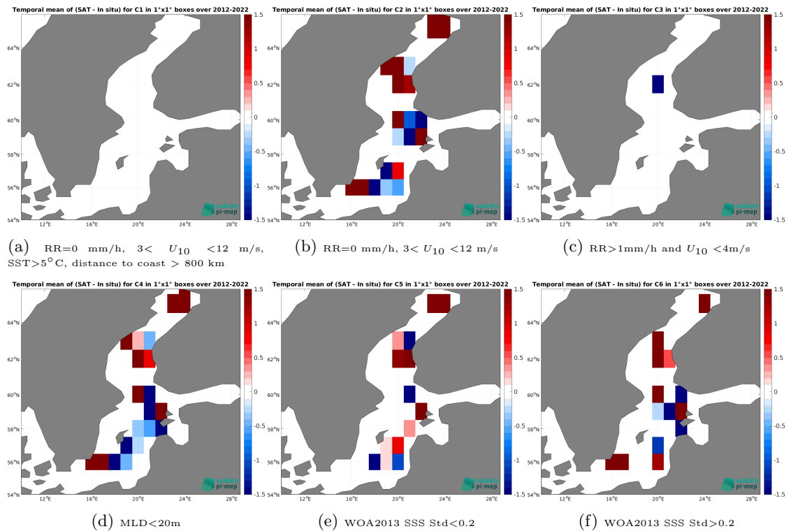
Figure 14: Temporal mean gridded over spatial boxes of size 1^\circ \times 1^\circ of \Delta SSS (SMOS SSS L2 v700 (ESA) - Argo) for 6 different subdatasets corresponding to:RR=0 mm/h, 3 < U_{10} < 12 m/s, SST > 5°C, distance to coast > 800 km (a), RR=0 mm/h, 3 < U_{10} < 12 m/s (b), RR > 1mm/h and U_{10} < 4 m/s (c),MLD < 20m (d),WOA2013 SSS Std < 0.2 (e),WOA2013 SSS Std > 0.2 (f).
