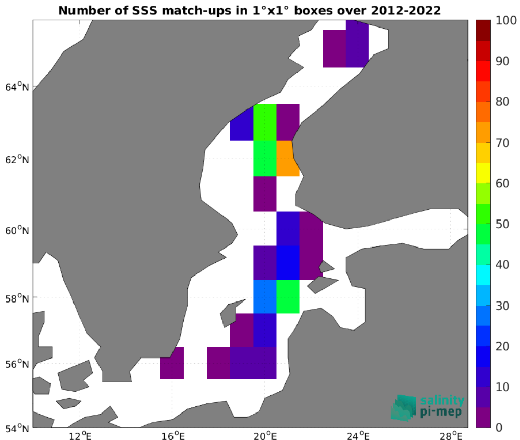
Figure 5: Number of SSS match-ups between Argo SSS and the SMOS SSS L2 v700 (ESA) SSS product for the Baltic Sea Pi-MEP region over 1^\circ \times 1^\circ boxes and for the full satellite product period.
