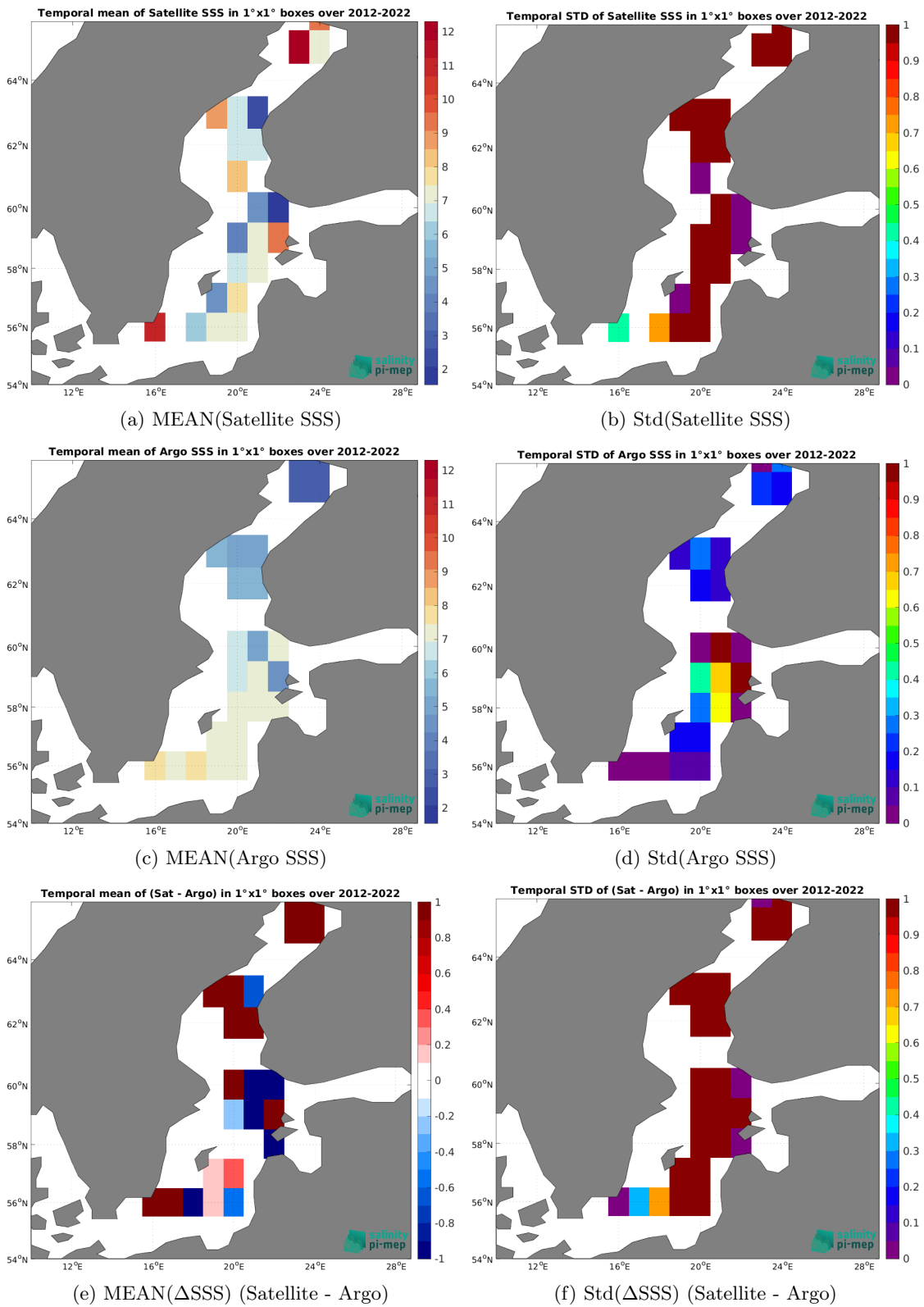
Figure 7: Temporal mean (left) and Std (right) of SSS from SMOS SSS L2 v700 (ESA) (top), Argo (middle), and of \Delta SSS (Satellite - Argo) (bottom). Only match-up pairs are used to generate these maps.
