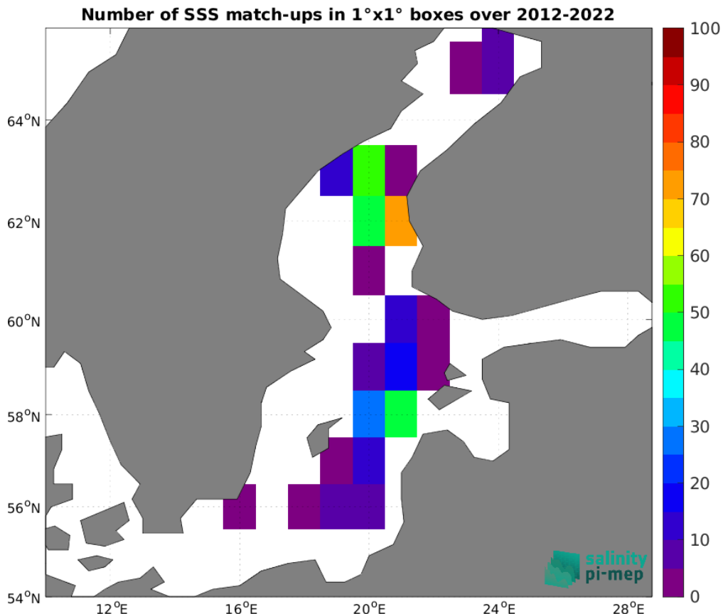
Figure 4: Number of SSS match-ups between Argo SSS and the SMOS SSS L2 v700 (ESA) SSS product for the Baltic Sea Pi-MEP region over 1^\circ \times 1^\circ boxes and for the full satellite product period.
