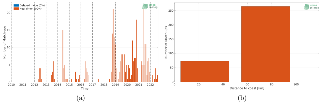
Figure 1: Number of match-ups between Argo and SMOS SSS L2 v700 (ESA) SSS as a function of time (a) and as function of the distance to coast (b) over the Baltic Sea Pi-MEP region and for the full satellite product period.
