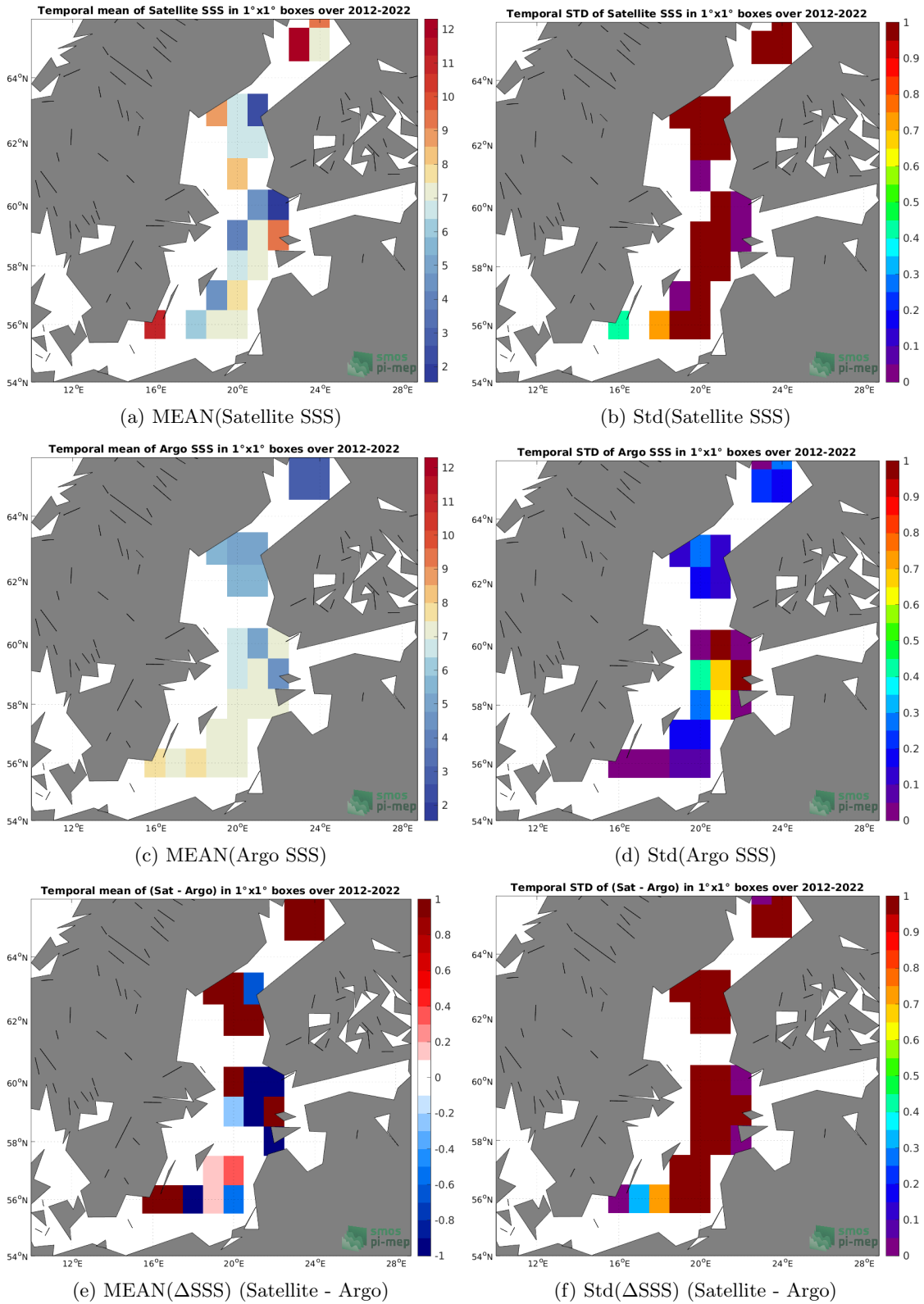
Figure 6: Temporal mean (left) and Std (right) of SSS from SMOS SSS L2 v700 (ESA) (top), Argo (middle), and of \Delta SSS (Satellite - Argo) (bottom). Only match-up pairs are used to generate these maps.
