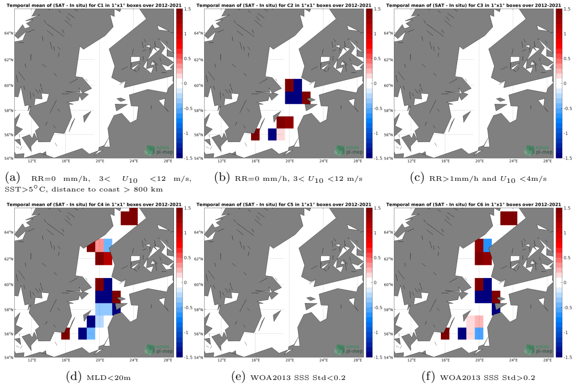
Figure 12: Temporal mean gridded over spatial boxes of size 1^{\circ}\times 1^{\circ} of \Delta\text{SSS} (SMOS SSS L2 v700 (ESA) - Argo) for 6 different subdatasets corresponding to:RR=0 mm/h, 3 < U_{10} < 12 m/s, SST >5^{\circ}\text{C} , distance to coast > 800 km (a), RR=0 mm/h, 3 < U_{10} < 12 m/s (b), RR >1\text{mm/h} and U_{10} < 4\text{m/s} (c),MLD <20\text{m} (d),WOA2013 SSS Std <0.2 (e),WOA2013 SSS Std >0.2 (f).
