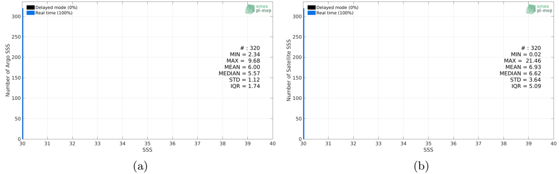
Figure 2: Histograms of SSS from Argo (a) and SMOS SSS L2 v700 (ESA) (b) considering all match-up pairs per bins of 0.1 over the Baltic Sea Pi-MEP region and for the full satellite product period.
