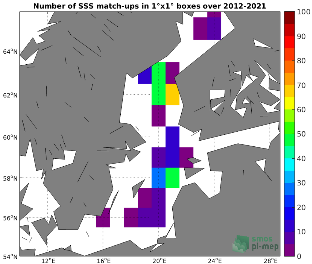
Figure 4: Number of SSS match-ups between Argo SSS and the SMOS SSS L2 v700 (ESA) SSS product for the Baltic Sea Pi-MEP region over 1°x1° boxes and for the full satellite product period.
