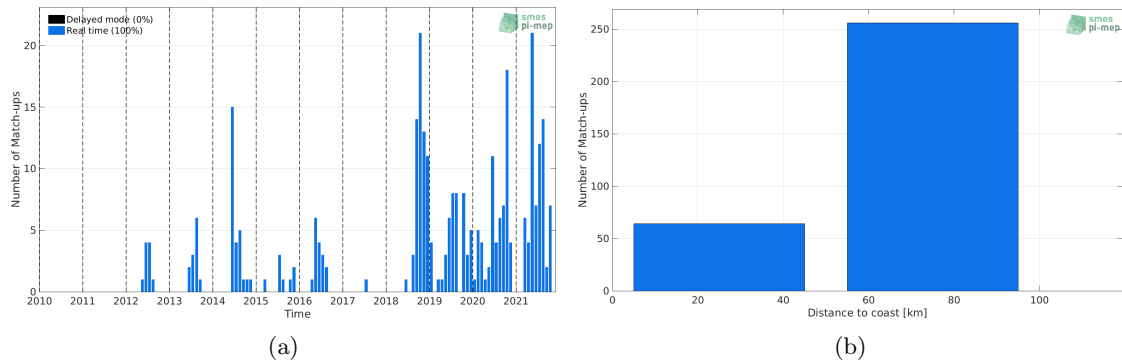
Figure 1: Number of match-ups between Argo and SMOS SSS L2 v700 (ESA) SSS as a function of time (a) and as function of the distance to coast (b) over the Baltic Sea Pi-MEP region and for the full satellite product period.
