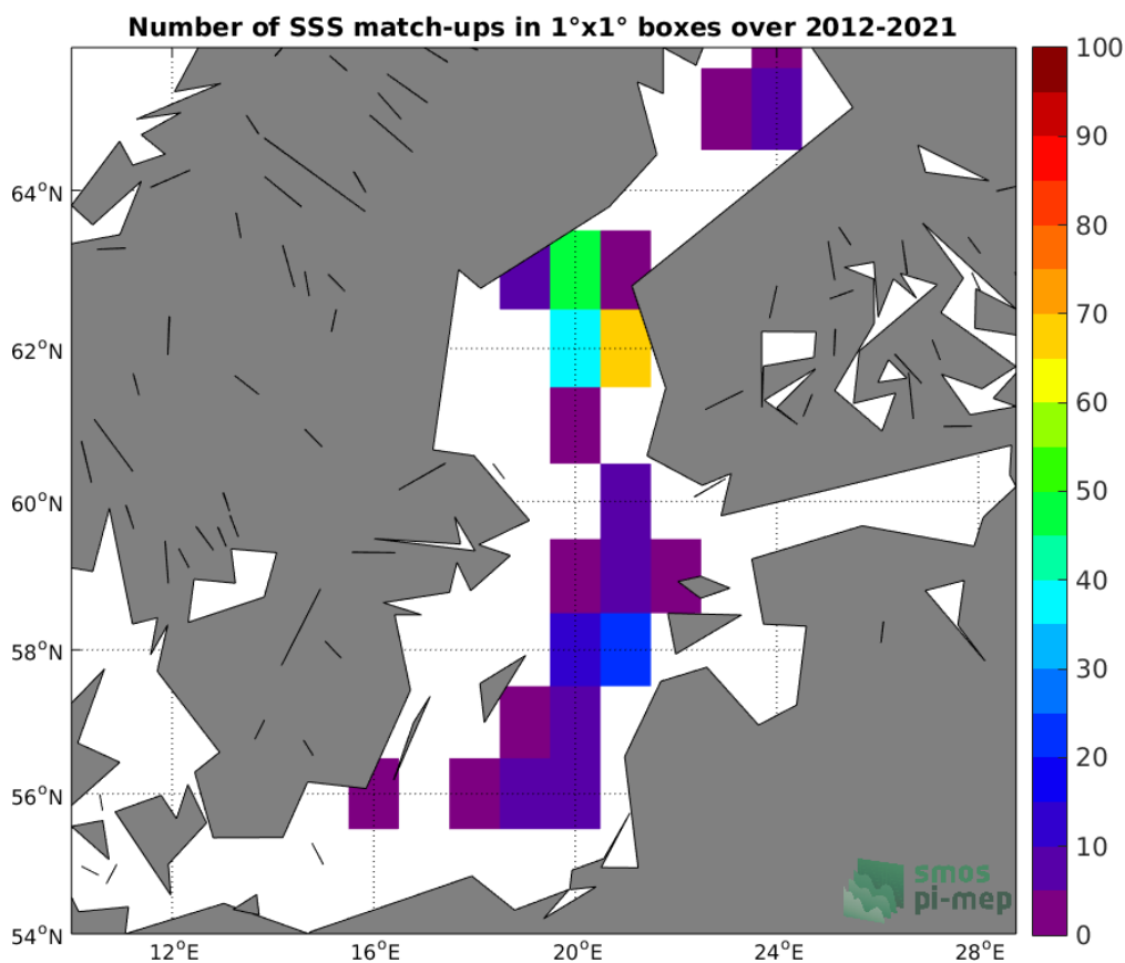
Figure 4: Number of SSS match-ups between Argo SSS and the SMOS SSS L2 v700 (ESA) SSS product for the Baltic Sea Pi-MEP region over 1^{\circ} \times 1^{\circ} boxes and for the full satellite product period.
