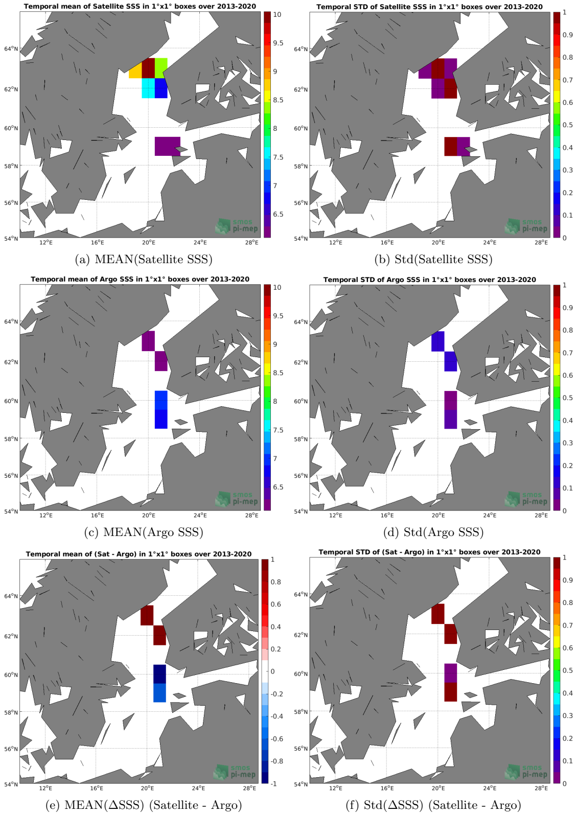
Figure 6: Temporal mean (left) and Std (right) of SSS from SMOS SSS L2 v662 (ESA) (top), Argo (middle), and of \Delta SSS (Satellite - Argo) (bottom). Only match-up pairs are used to generate these maps.
