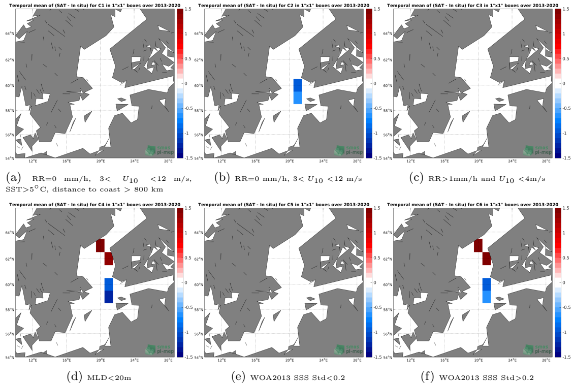
Figure 12: Temporal mean gridded over spatial boxes of size 1^{\circ}\times 1^{\circ} of \Delta\text{SSS} (SMOS SSS L2 v662 (ESA) - Argo) for 6 different subdatasets corresponding to:RR=0 mm/h, 3 < U_{10} < 12 m/s, SST > 5^{\circ}\text{C} , distance to coast > 800 km (a), RR=0 mm/h, 3 < U_{10} < 12 m/s (b), RR > 1\text{mm/h} and U_{10} < 4\text{m/s} (c),MLD < 20\text{m} (d),WOA2013 SSS Std < 0.2 (e),WOA2013 SSS Std > 0.2 (f).
