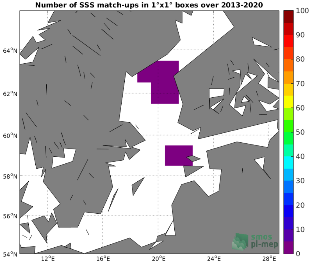
Figure 4: Number of SSS match-ups between Argo SSS and the SMOS SSS L2 v662 (ESA) SSS product for the Baltic Sea Pi-MEP region over 1°x1° boxes and for the full satellite product period.
