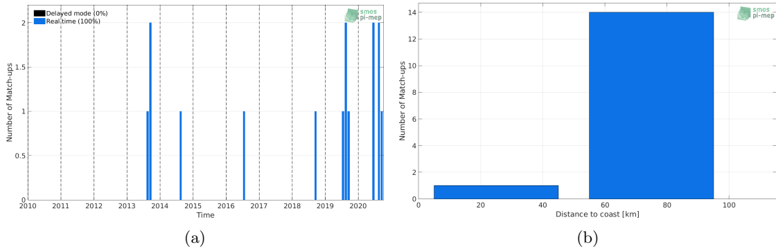
Figure 1: Number of match-ups between Argo and SMOS SSS L2 v662 (ESA) SSS as a function of time (a) and as function of the distance to coast (b) over the Baltic Sea Pi-MEP region and for the full satellite product period.
