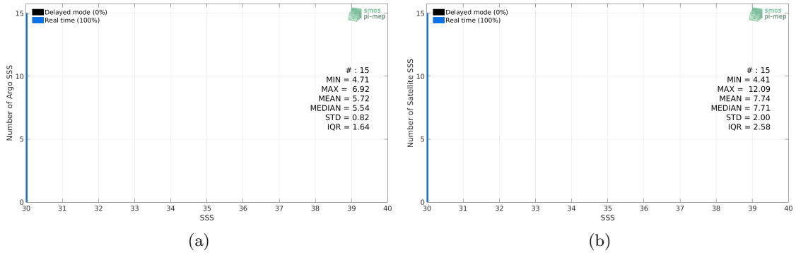
Figure 2: Histograms of SSS from Argo (a) and SMOS SSS L2 v662 (ESA) (b) considering all match-up pairs per bins of 0.1 over the Baltic Sea Pi-MEP region and for the full satellite product period.
