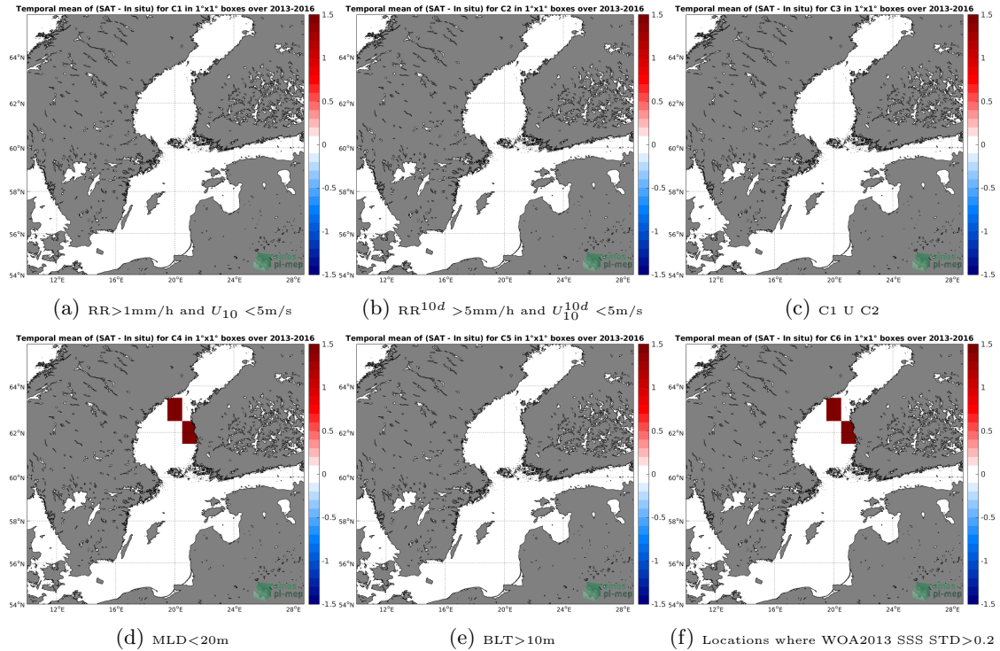
Figure 12: Temporal mean gridded over spatial boxes of size 1^\circ \times 1^\circ of \Delta\text{SSS} (SMOS-L2-DPGS-v662 - Argo) for 6 different subdatasets corresponding to: RR > 1\text{mm/h} and U_{10} < 5\text{m/s} (a), RR^{10d} > 5\text{mm/h} and U_{10}^{10d} < 5\text{m/s} (b), C1 U C2 (c), MLD < 20\text{m} (d), BLT > 10\text{m} (e), Locations where WOA2013 SSS STD > 0.2 (f).
