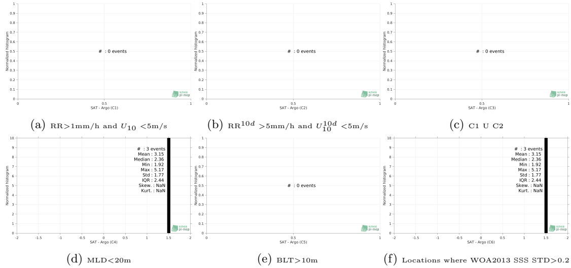
Figure 13: Normalized histogram of \Delta SSS (SMOS-L2-DPGS-v662 - Argo) for 6 different sub-datasets corresponding to: RR>1mm/h and U_{10} < 5 m/s (a), RR^{10d} > 5 mm/h and U_{10}^{10d} < 5 m/s (b), C1 U C2 (c),MLD<20m (d),BLT>10m (e),Locations where WOA2013 SSS STD>0.2 (f).
