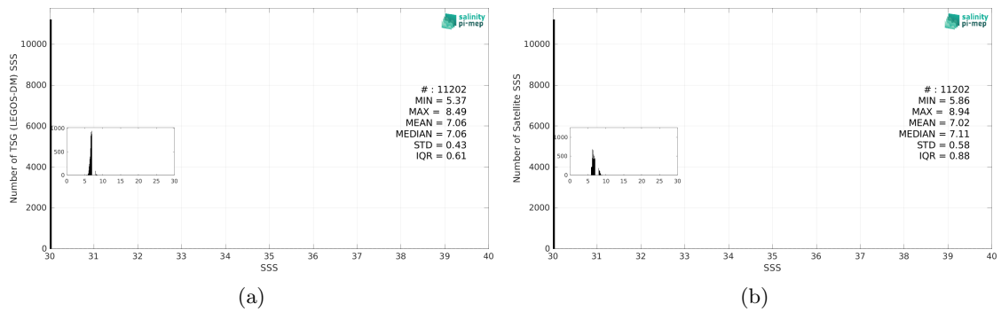
Figure 3: Histograms of SSS from TSG (LEGOS-DM) (a) and SMAP SSS L4 OI v3 - Monthly (ESR) (b) considering all match-up pairs per bins of 0.1 over the Baltic Sea Pi-MEP region and for the full satellite product period.
