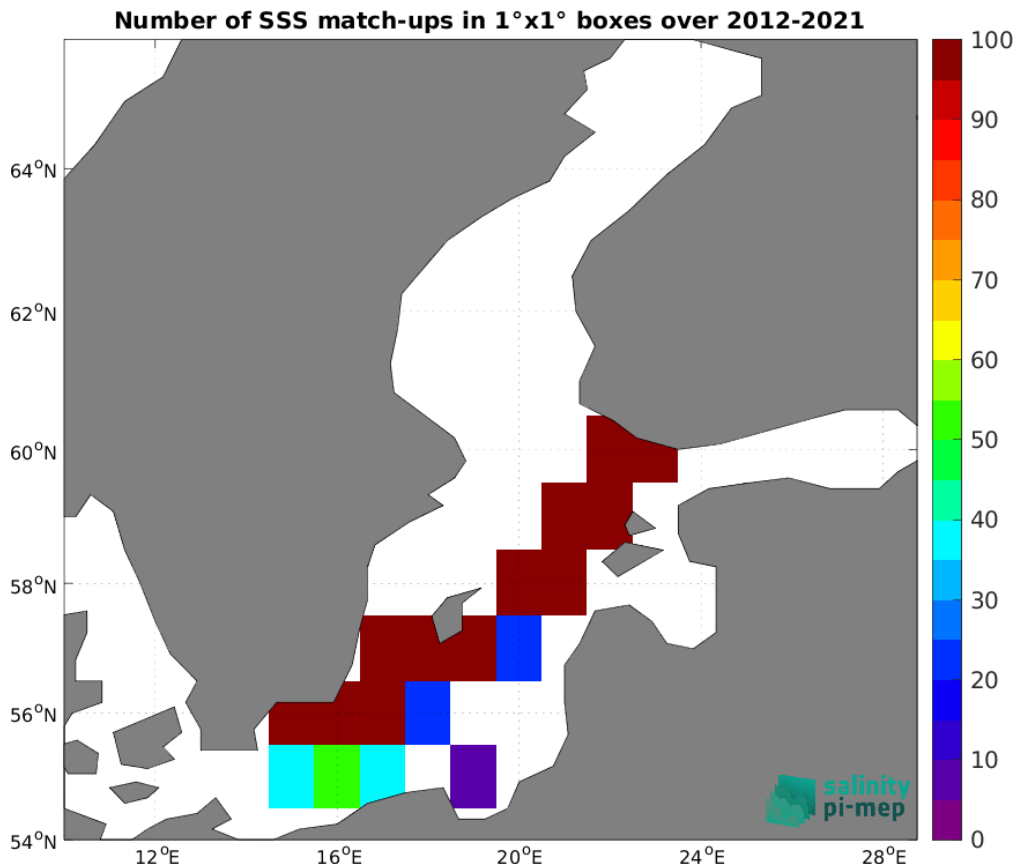
Figure 5: Number of SSS match-ups between TSG (LEGOS-DM) SSS and the SMAP SSS L4 OI v3 - Monthly (ESR) SSS product for the Baltic Sea Pi-MEP region over 1^\circ \times 1^\circ boxes and for the full satellite product period.
