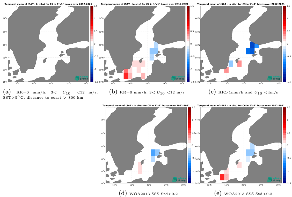
Figure 14: Temporal mean gridded over spatial boxes of size 1^\circ \times 1^\circ of \Delta\text{SSS} (SMAP SSS L4 OI v3 - Monthly (ESR) - TSG (LEGOS-DM)) for 5 different subdatasets corresponding to:RR=0 mm/h, 3 < U_{10} < 12 m/s, SST >5^\circ\text{C} , distance to coast > 800 km (a), RR=0 mm/h, 3 < U_{10} < 12 m/s (b), RR >1 mm/h and U_{10} < 4 m/s (c), WOA2013 SSS Std <0.2 (d), WOA2013 SSS Std >0.2 (e).
