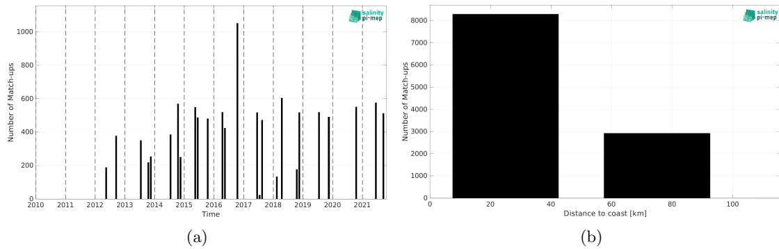
Figure 2: Number of match-ups between TSG (LEGOS-DM) and SMAP SSS L4 OI v3 - Monthly (ESR) SSS as a function of time (a) and as function of the distance to coast (b) over the Baltic Sea Pi-MEP region and for the full satellite product period.
