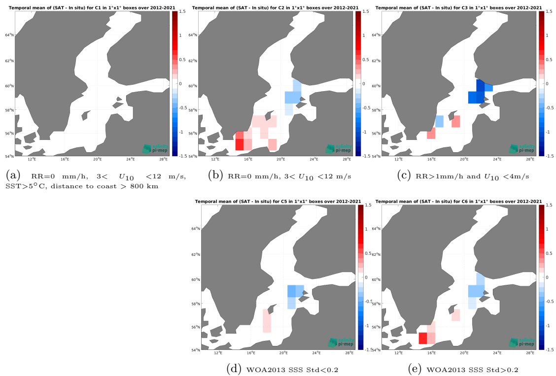
Figure 14: Temporal mean gridded over spatial boxes of size 1^\circ \times 1^\circ of \Delta SSS (SMAP SSS L4 OI v3 - Monthly (ESR) - TSG (LEGOS-DM)) for 5 different subdatasets corresponding to:RR=0 mm/h, 3 < U_{10} < 12 m/s, SST >5^\circ\text{C} , distance to coast > 800 km (a), RR=0 mm/h, 3 < U_{10} < 12 m/s (b), RR >1 mm/h and U_{10} < 4 m/s (c), WOA2013 SSS Std <0.2 (d), WOA2013 SSS Std >0.2 (e).
