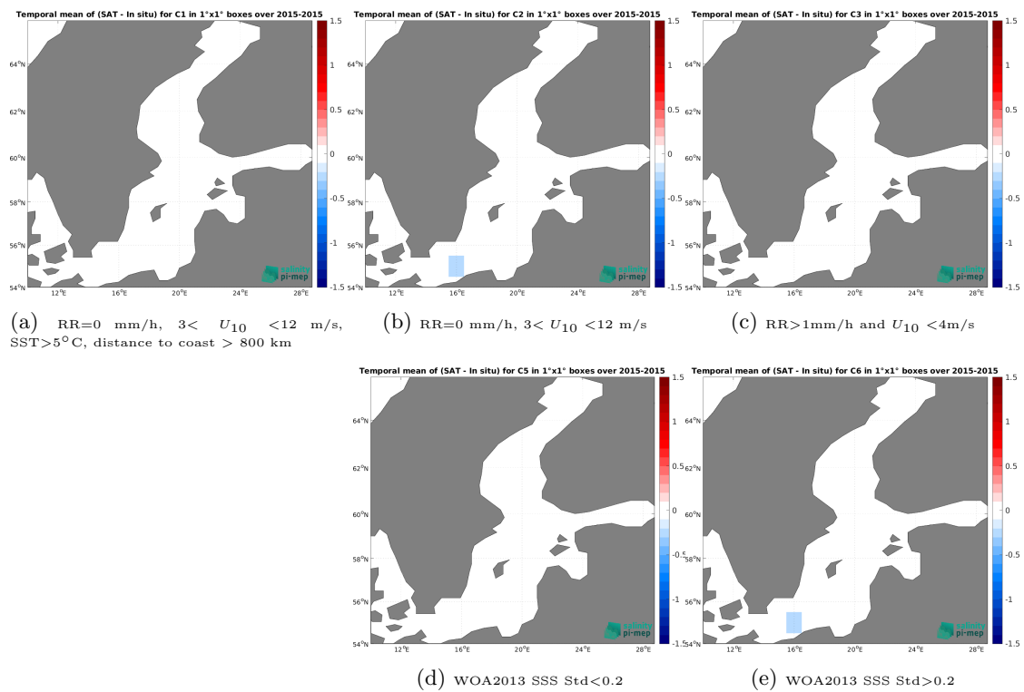
Figure 14: Temporal mean gridded over spatial boxes of size 1^\circ \times 1^\circ of \Delta SSS (SMAP SSS L4 OI v3 - Monthly (ESR) - TSG (GOSUD-Research-vessel)) for 5 different subdatasets corresponding to:RR=0 mm/h, 3 < U_{10} < 12 m/s, SST >5^\circ C, distance to coast > 800 km (a), RR=0 mm/h, 3 < U_{10} < 12 m/s (b), RR >1 mm/h and U_{10} < 4 m/s (c), WOA2013 SSS Std <0.2 (d), WOA2013 SSS Std >0.2 (e).
