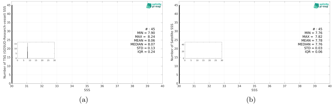
Figure 3: Histograms of SSS from TSG (GOSUD-Research-vessel) (a) and SMAP SSS L4 OI v3 - Monthly (ESR) (b) considering all match-up pairs per bins of 0.1 over the Baltic Sea Pi-MEP region and for the full satellite product period.
