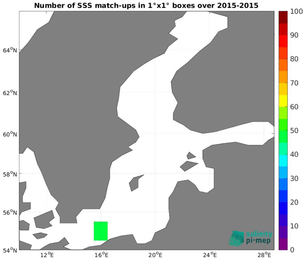
Figure 5: Number of SSS match-ups between TSG (GOSUD-Research-vessel) SSS and the SMAP SSS L4 OI v3 - Monthly (ESR) SSS product for the Baltic Sea Pi-MEP region over 1^\circ \times 1^\circ boxes and for the full satellite product period.
