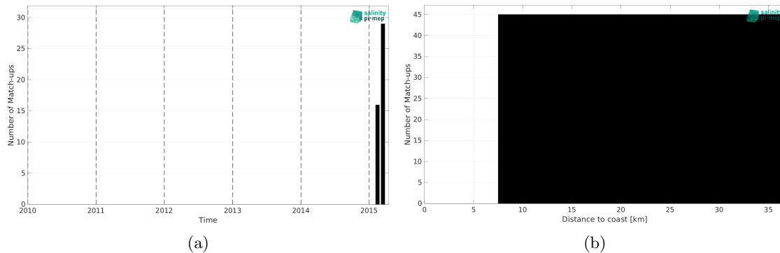
Figure 2: Number of match-ups between TSG (GOSUD-Research-vessel) and SMAP SSS L4 OI v3 - Monthly (ESR) SSS as a function of time (a) and as function of the distance to coast (b) over the Baltic Sea Pi-MEP region and for the full satellite product period.
