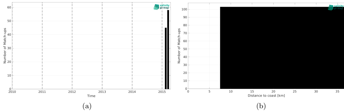
Figure 2: Number of match-ups between TSG (GOSUD-Research-vessel) and SMAP SSS L4 OI v3 - Monthly (ESR) SSS as a function of time (a) and as function of the distance to coast (b) over the Baltic Sea Pi-MEP region and for the full satellite product period.
