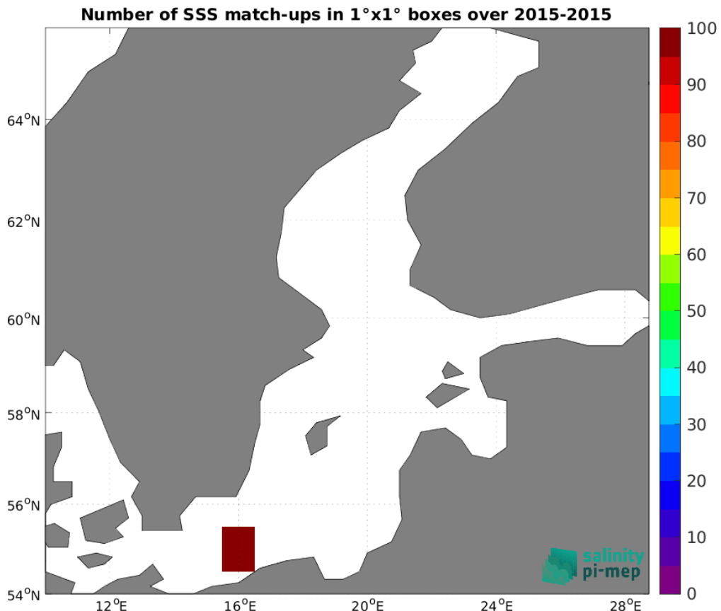
Figure 5: Number of SSS match-ups between TSG (GOSUD-Research-vessel) SSS and the SMAP SSS L4 OI v3 - Monthly (ESR) SSS product for the Baltic Sea Pi-MEP region over 1°×1° boxes and for the full satellite product period.
