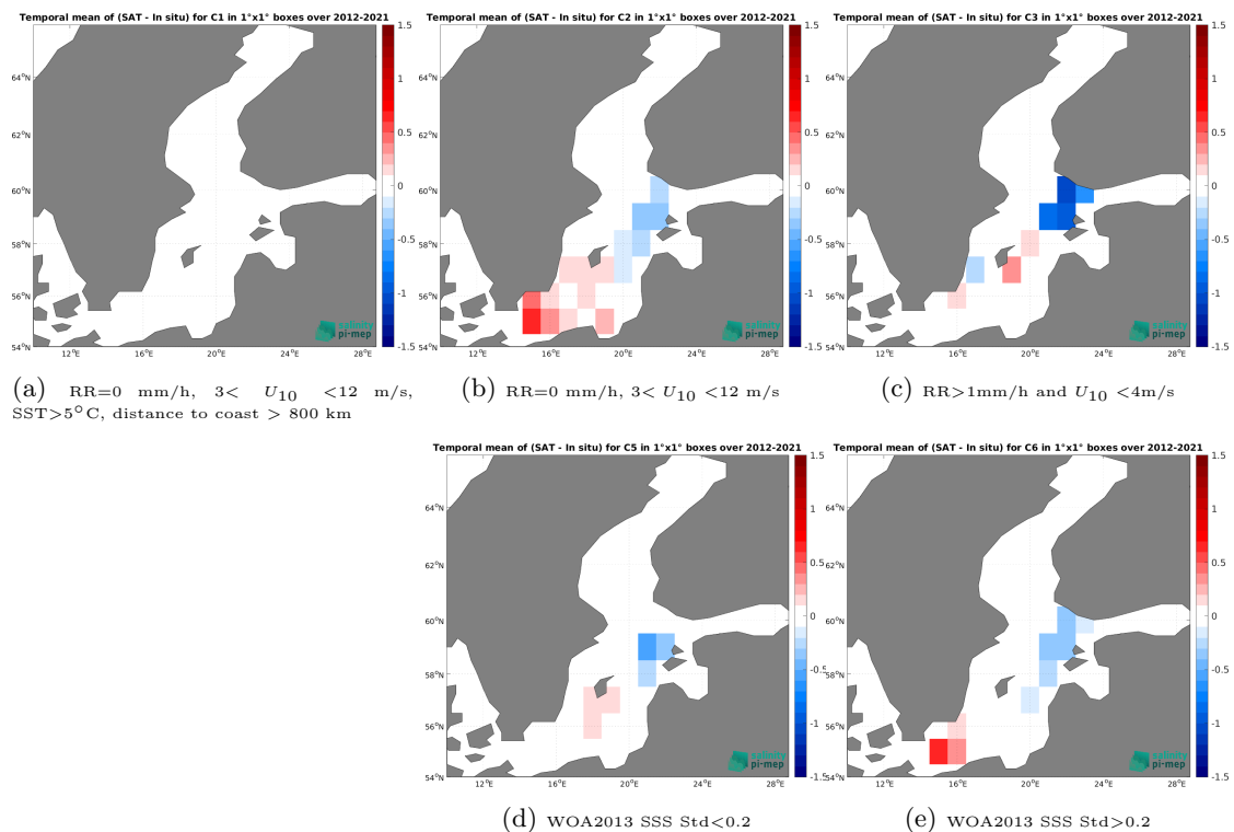
Figure 14: Temporal mean gridded over spatial boxes of size 1^\circ \times 1^\circ of \Delta\text{SSS} (SMAP SSS L4 OI v3 - Daily (ESR) - TSG (LEGOS-DM)) for 5 different subdatasets corresponding to:RR=0 mm/h, 3 < U_{10} < 12 m/s, SST>5°C, distance to coast > 800 km (a), RR=0 mm/h, 3 < U_{10} < 12 m/s (b), RR>1mm/h and U_{10} < 4 m/s (c), WOA2013 SSS Std<0.2 (d), WOA2013 SSS Std>0.2 (e).
