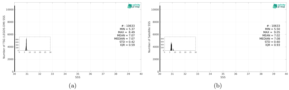
Figure 3: Histograms of SSS from TSG (LEGOS-DM) (a) and SMAP SSS L4 OI v3 - Daily (ESR) (b) considering all match-up pairs per bins of 0.1 over the Baltic Sea Pi-MEP region and for the full satellite product period.
