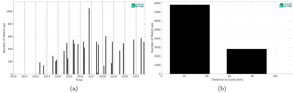
Figure 2: Number of match-ups between TSG (LEGOS-DM) and SMAP SSS L4 OI v3 - Daily (ESR) SSS as a function of time (a) and as function of the distance to coast (b) over the Baltic Sea Pi-MEP region and for the full satellite product period.
