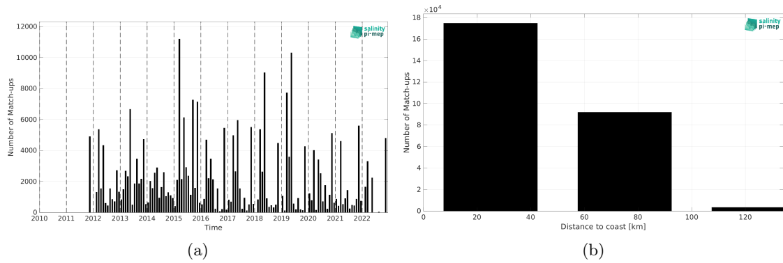
Figure 2: Number of match-ups between ICES and SMAP SSS L4 OI v3 - Daily (ESR) SSS as a function of time (a) and as function of the distance to coast (b) over the Baltic Sea Pi-MEP region and for the full satellite product period.
