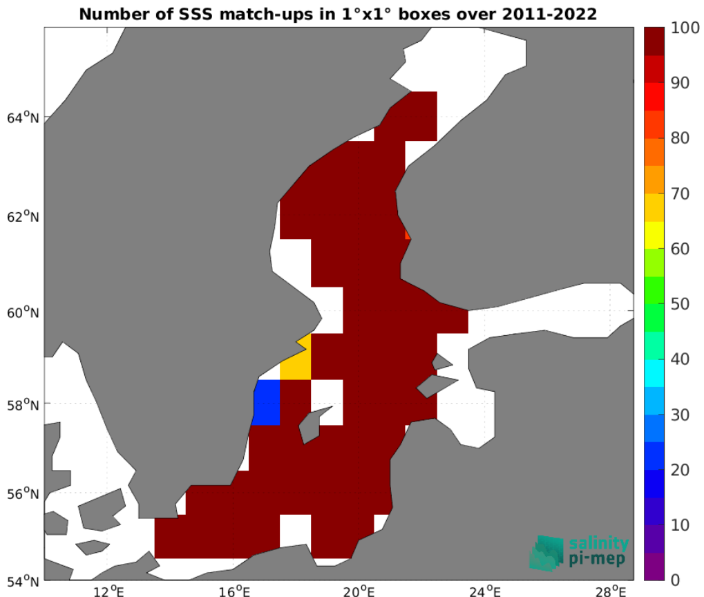
Figure 5: Number of SSS match-ups between ICES SSS and the SMAP SSS L4 OI v3 - Daily (ESR) SSS product for the Baltic Sea Pi-MEP region over 1^\circ \times 1^\circ boxes and for the full satellite product period.
