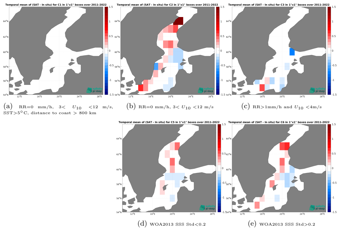
Figure 14: Temporal mean gridded over spatial boxes of size 1^\circ \times 1^\circ of \Delta SSS (SMAP SSS L4 OI v3 - Daily (ESR) - ICES) for 5 different subdatasets corresponding to:RR=0 mm/h, 3 < U_{10} < 12 m/s, SST >5^\circ\text{C} , distance to coast > 800 km (a), RR=0 mm/h, 3 < U_{10} < 12 m/s (b), RR >1 mm/h and U_{10} < 4 m/s (c), WOA2013 SSS Std <0.2 (d), WOA2013 SSS Std >0.2 (e).
