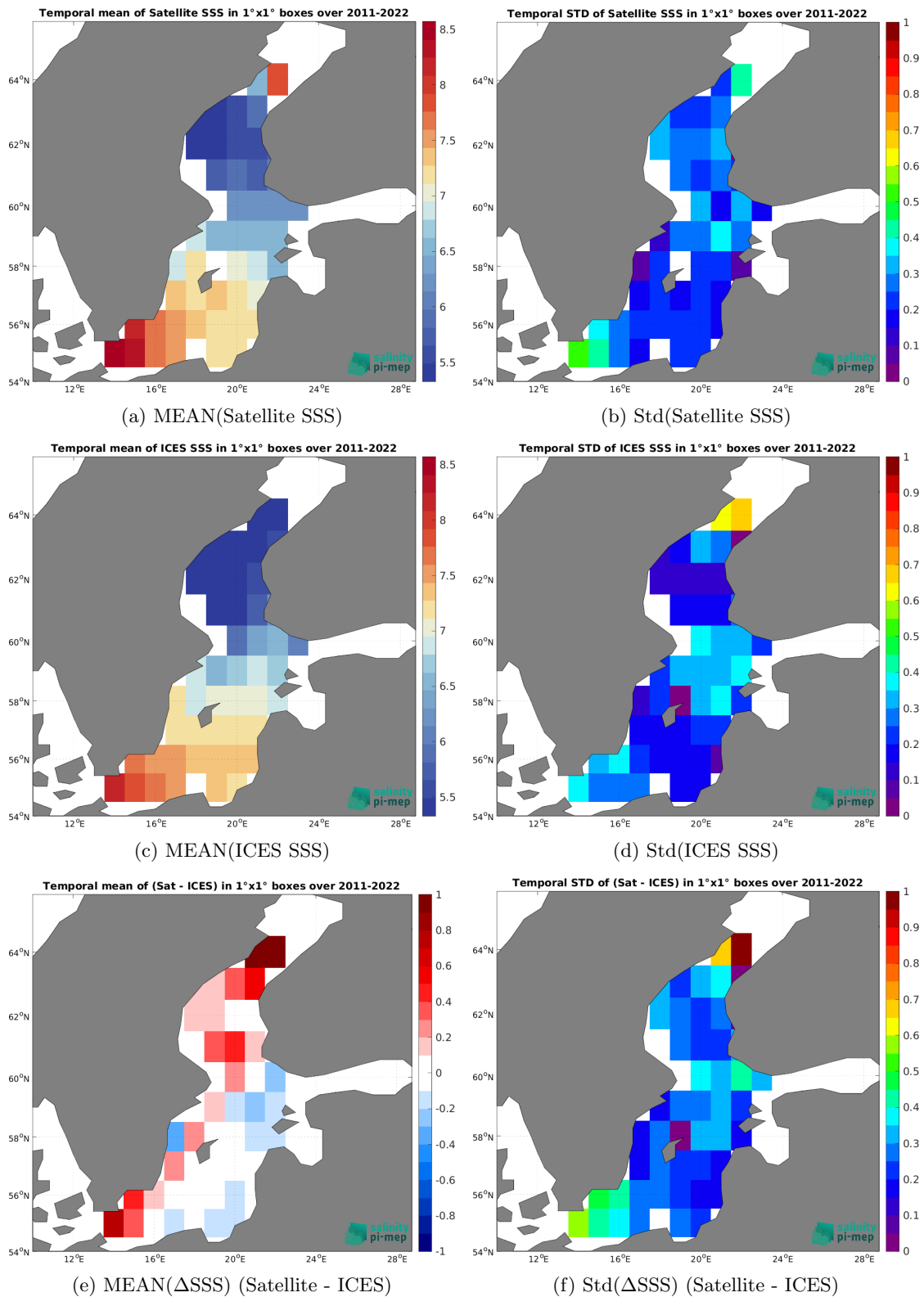
Figure 7: Temporal mean (left) and Std (right) of SSS from SMAP SSS L4 OI v3 - Daily (ESR) (top), ICES (middle), and of \Delta SSS (Satellite - ICES). Only match-up pairs are used to generate these maps.
