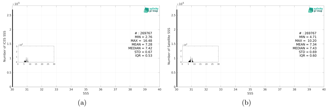
Figure 3: Histograms of SSS from ICES (a) and SMAP SSS L4 OI v3 - Daily (ESR) (b) considering all match-up pairs per bins of 0.1 over the Baltic Sea Pi-MEP region and for the full satellite product period.
