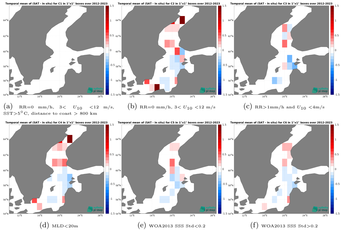
Figure 14: Temporal mean gridded over spatial boxes of size 1^\circ \times 1^\circ of \Delta\text{SSS} (SMAP SSS L4 OI v3 - Daily (ESR) - Argo) for 6 different subdatasets corresponding to:RR=0 mm/h, 3 < U_{10} < 12 m/s, SST>5°C, distance to coast > 800 km (a), RR=0 mm/h, 3 < U_{10} < 12 m/s (b), RR>1mm/h and U_{10} < 4 m/s (c),MLD<20m (d),WOA2013 SSS Std<0.2 (e),WOA2013 SSS Std>0.2 (f).
