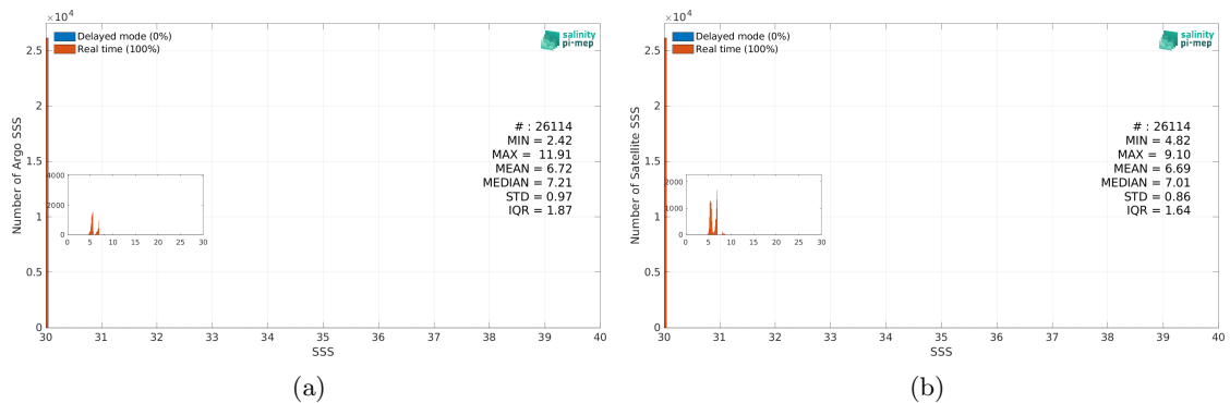
Figure 3: Histograms of SSS from Argo (a) and SMAP SSS L4 OI v3 - Daily (ESR) (b) considering all match-up pairs per bins of 0.1 over the Baltic Sea Pi-MEP region and for the full satellite product period.
