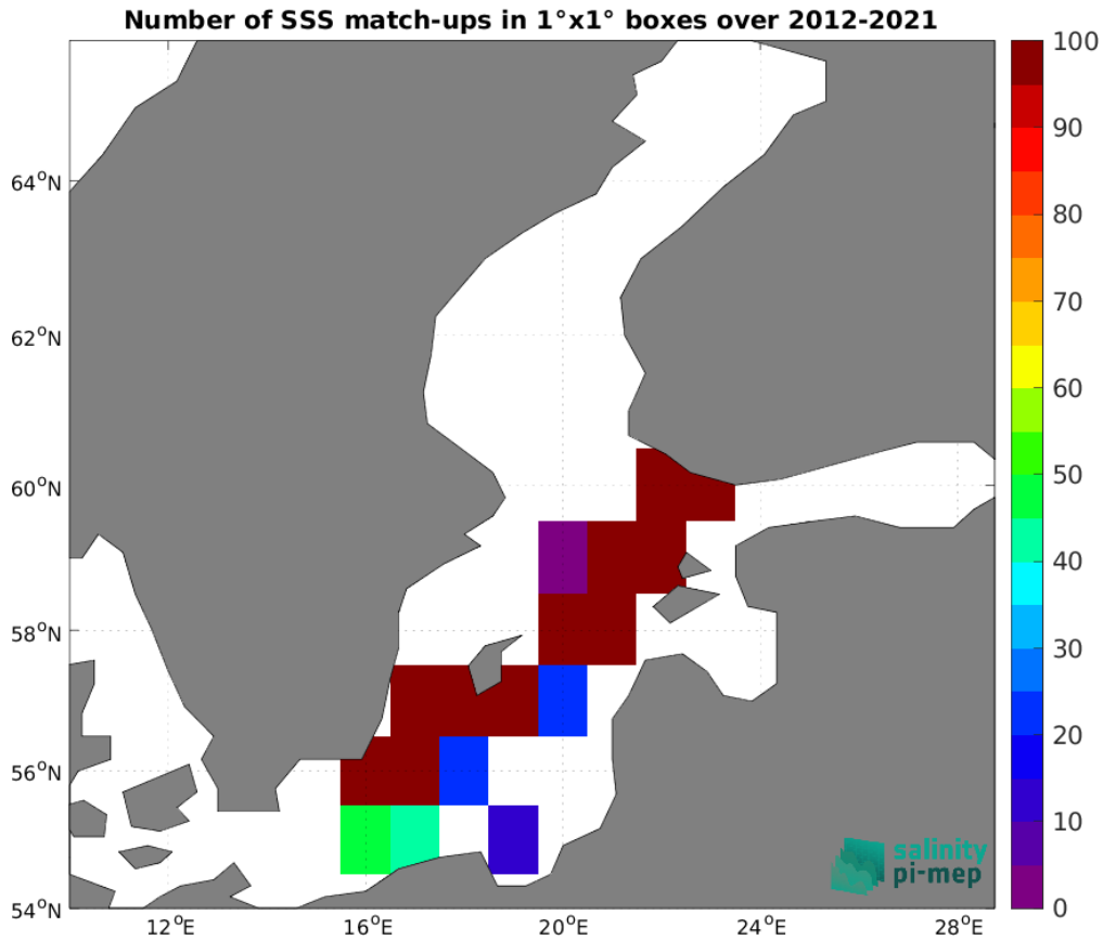
Figure 4: Number of SSS match-ups between TSG (LEGOS-DM) SSS and the SMAP SSS L4 OI v2 - 7 Days (ESR) SSS product for the Baltic Sea Pi-MEP region over 1^\circ \times 1^\circ boxes and for the full satellite product period.
