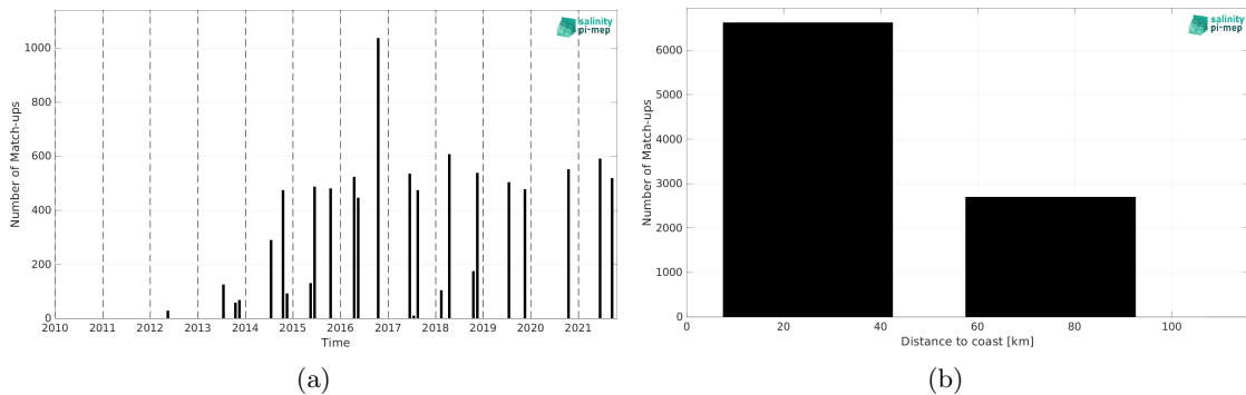
Figure 1: Number of match-ups between TSG (LEGOS-DM) and SMAP SSS L4 OI v2 - 7 Days (ESR) SSS as a function of time (a) and as function of the distance to coast (b) over the Baltic Sea Pi-MEP region and for the full satellite product period.
