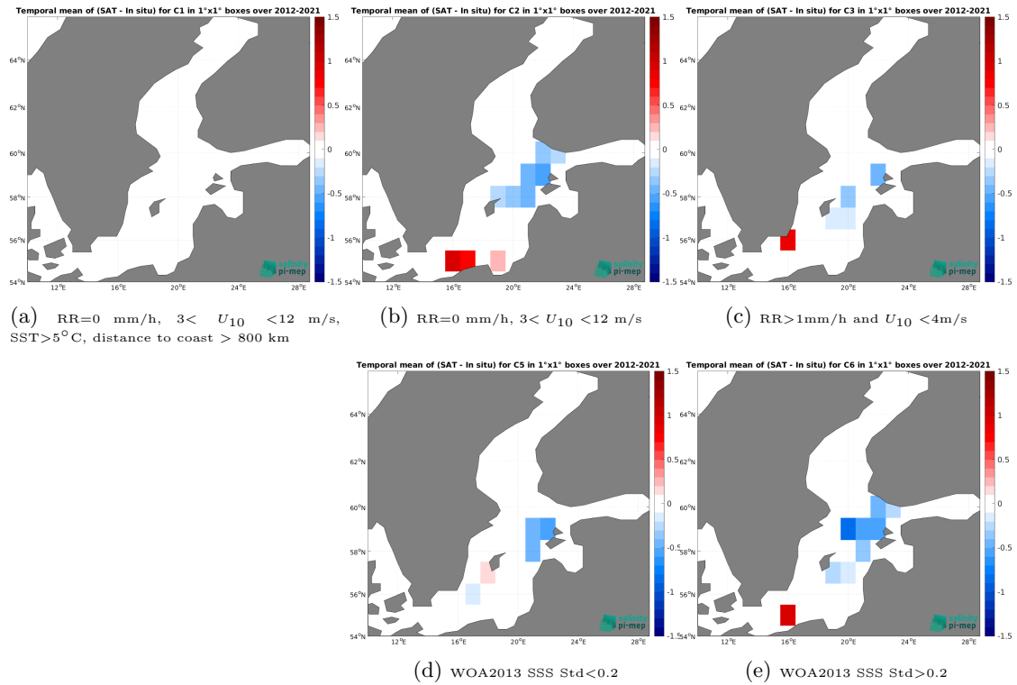
Figure 12: Temporal mean gridded over spatial boxes of size 1^{\circ}\times 1^{\circ} of \Delta\text{SSS} (SMAP SSS L4 OI v2 - 7 Days (ESR) - TSG (LEGOS-DM)) for 5 different subdatasets corresponding to: \text{RR}=0 mm/h, 3 < U_{10} < 12 m/s, \text{SST} > 5^{\circ}\text{C} , distance to coast > 800 km (a), \text{RR}=0 mm/h, 3 < U_{10} < 12 m/s (b), \text{RR} > 1\text{mm/h} and U_{10} < 4\text{m/s} (c), WOA2013 SSS Std < 0.2 (d), WOA2013 SSS Std > 0.2 (e).
