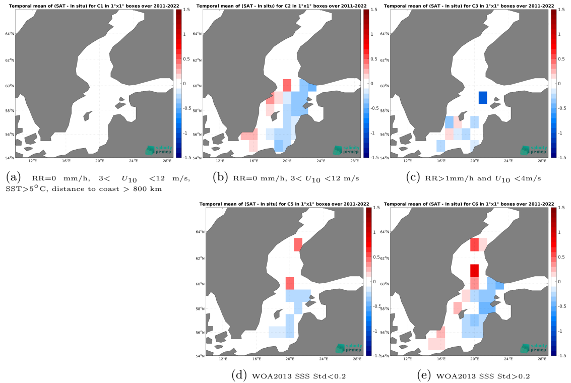
Figure 12: Temporal mean gridded over spatial boxes of size 1^{\circ}\times 1^{\circ} of \Delta\text{SSS} (SMAP SSS L4 OI v2 - 7 Days (ESR) - ICES) for 5 different subdatasets corresponding to:RR=0 mm/h, 3 < U_{10} < 12 m/s, SST >5^{\circ}\text{C} , distance to coast > 800 km (a), RR=0 mm/h, 3 < U_{10} < 12 m/s (b), RR >1 mm/h and U_{10} < 4 m/s (c), WOA2013 SSS Std <0.2 (d), WOA2013 SSS Std >0.2 (e).
