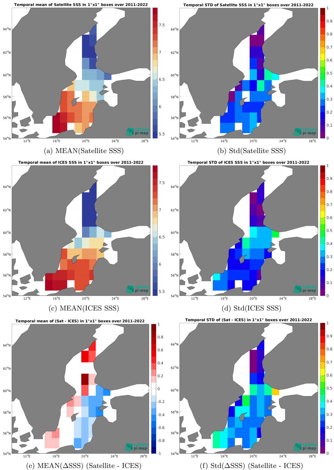
Figure 6: Temporal mean (left) and Std (right) of SSS from SMAP SSS L4 OI v2 - 7 Days (ESR) (top), ICES (middle), and of \Delta SSS (Satellite - ICES). Only match-up pairs are used to generate these maps.
