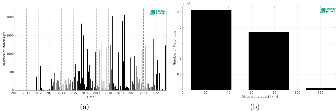
Figure 1: Number of match-ups between ICES and SMAP SSS L4 OI v2 - 7 Days (ESR) SSS as a function of time (a) and as function of the distance to coast (b) over the Baltic Sea Pi-MEP region and for the full satellite product period.
