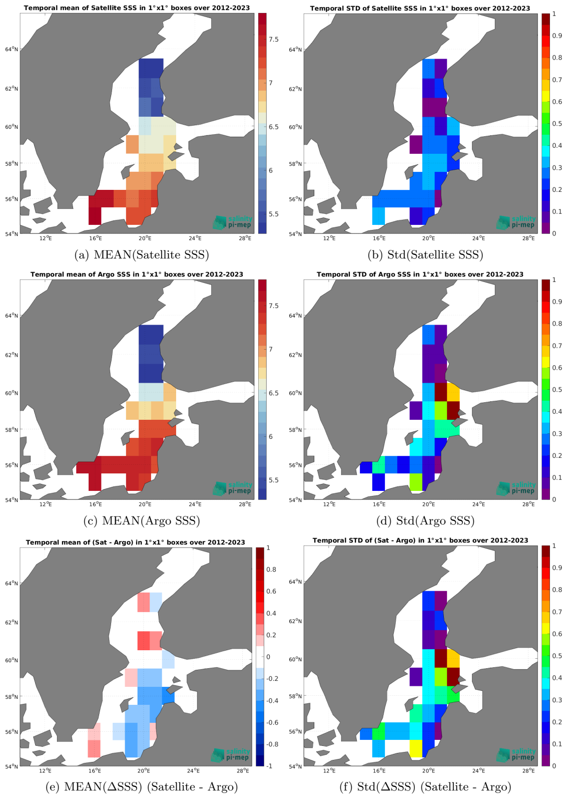
Figure 6: Temporal mean (left) and Std (right) of SSS from SMAP SSS L4 OI v2 - 7 Days (ESR) (top), Argo (middle), and of \Delta SSS (Satellite - Argo). Only match-up pairs are used to generate these maps.
