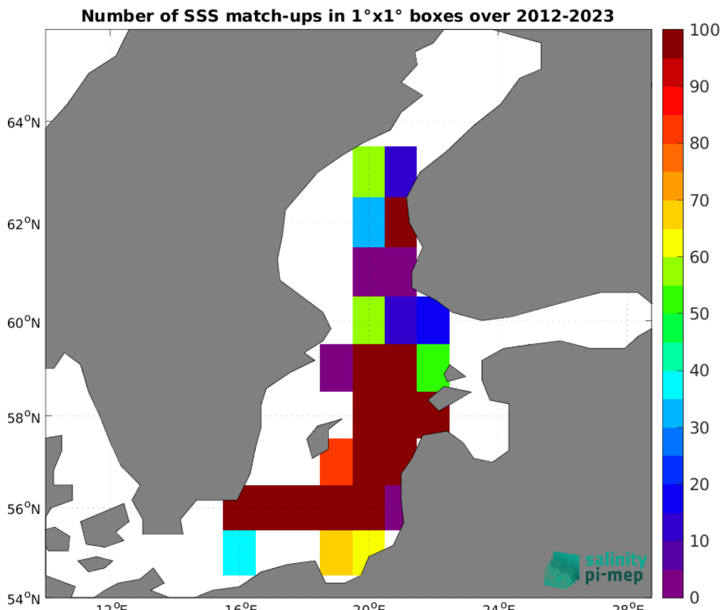
Figure 4: Number of SSS match-ups between Argo SSS and the SMAP SSS L4 OI v2 - 7 Days (ESR) SSS product for the Baltic Sea Pi-MEP region over 1^\circ \times 1^\circ boxes and for the full satellite product period.
