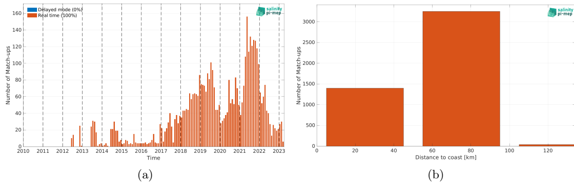
Figure 1: Number of match-ups between Argo and SMAP SSS L4 OI v2 - 7 Days (ESR) SSS as a function of time (a) and as function of the distance to coast (b) over the Baltic Sea Pi-MEP region and for the full satellite product period.
