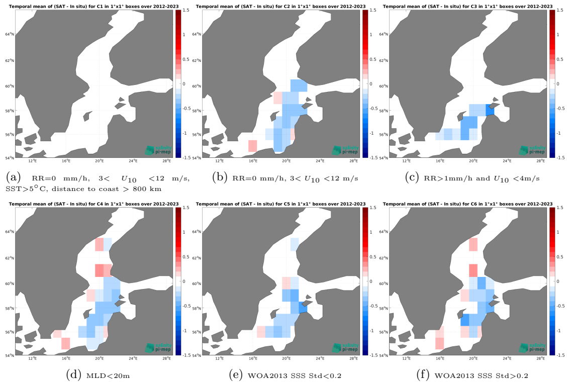
Figure 12: Temporal mean gridded over spatial boxes of size 1^{\circ}\times 1^{\circ} of \Delta\text{SSS} (SMAP SSS L4 OI v2 - 7 Days (ESR) - Argo) for 6 different subdatasets corresponding to:RR=0 mm/h, 3 < U_{10} < 12 m/s, SST >5^{\circ}\text{C} , distance to coast > 800 km (a), RR=0 mm/h, 3 < U_{10} < 12 m/s (b), RR >1 mm/h and U_{10} < 4 m/s (c),MLD <20 m (d),WOA2013 SSS Std <0.2 (e),WOA2013 SSS Std >0.2 (f).
