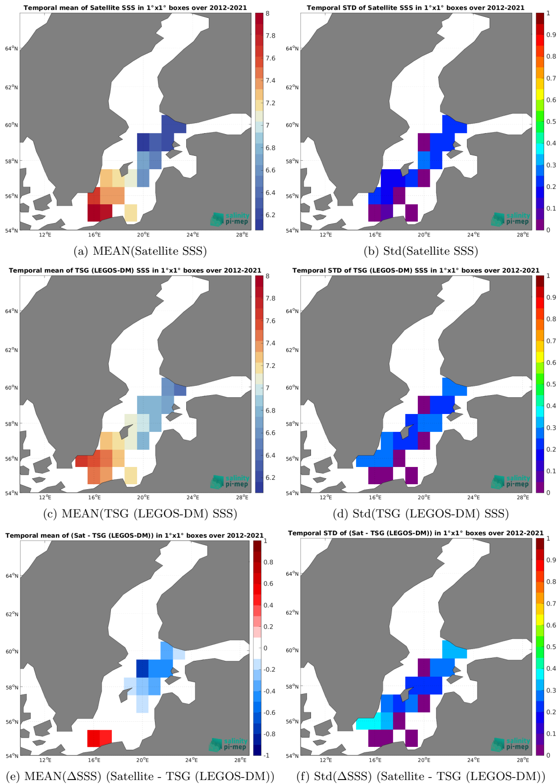
Figure 6: Temporal mean (left) and Std (right) of SSS from SMAP SSS L4 OI v2 - Monthly (IPRC) (top), TSG (LEGOS-DM) (middle), and \Delta SSS (Satellite - TSG (LEGOS-DM)). Only match-up pairs are used to generate these maps.
