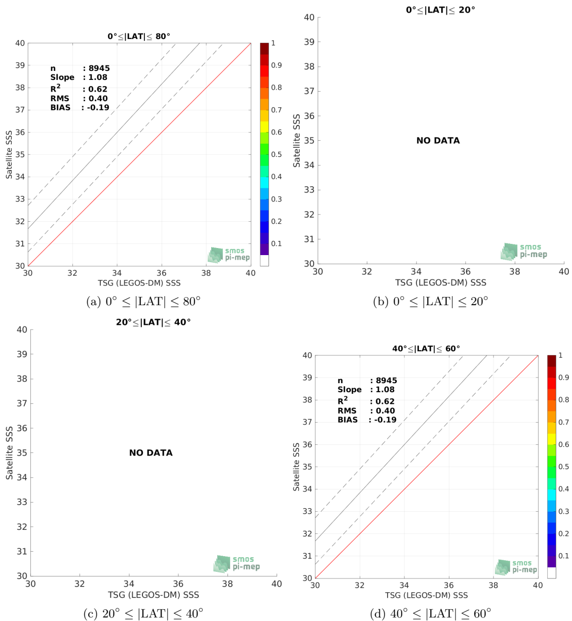
Figure 9: Contour maps of the concentration of SMAP SSS L4 OI v2 - Monthly (IPRC) SSS (y-axis) versus TSG (LEGOS-DM) SSS (x-axis) at match-up pairs for different latitude bands. For each plot, the red line shows x=y . The black thin and dashed lines indicate a linear fit through the data cloud and the \pm 95\% confidence levels, respectively. The number match-up pairs n , the slope and R^2 coefficient of the linear fit, the root mean square (RMS) and the mean bias between satellite and in situ data are indicated for each latitude band in each plots.
