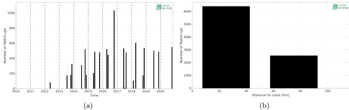
Figure 1: Number of match-ups between TSG (LEGOS-DM) and SMAP SSS L4 OI v2 - Monthly (IPRC) SSS as a function of time (a) and as function of the distance to coast (b) over the Baltic Sea Pi-MEP region and for the full satellite product period.
