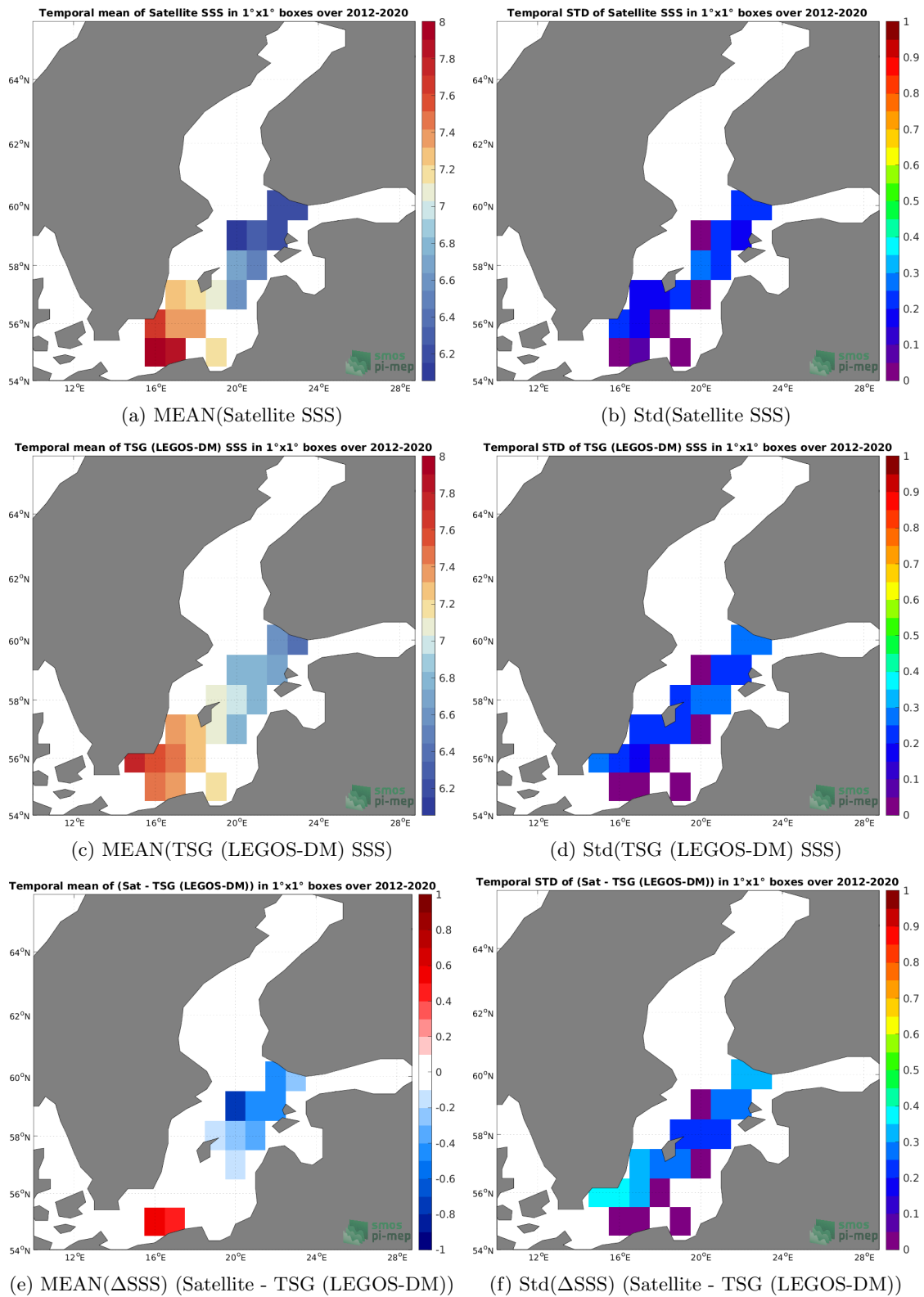
Figure 6: Temporal mean (left) and Std (right) of SSS from SMAP SSS L4 OI v2 - Monthly (IPRC) (top), TSG (LEGOS-DM) (middle), and of \Delta SSS (Satellite - TSG (LEGOS-DM)). Only match-up pairs are used to generate these maps.
