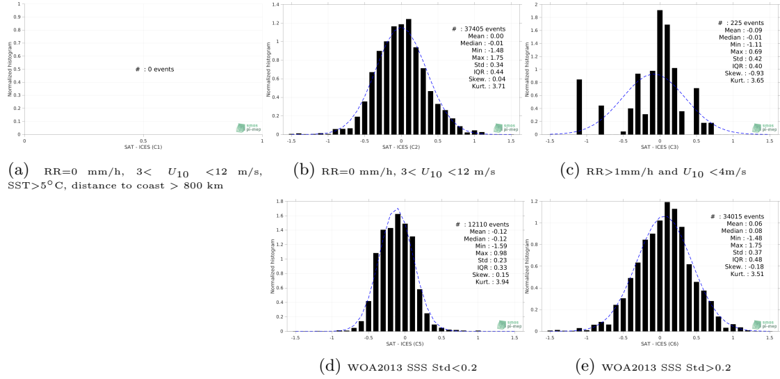
Figure 13: Normalized histogram of \Delta SSS (SMAP SSS L4 OI v2 - Monthly (IPRC) - ICES) for 5 different subdatasets corresponding to: RR=0 mm/h, 3 < U_{10} < 12 m/s, SST > 5°C, distance to coast > 800 km (a), RR=0 mm/h, 3 < U_{10} < 12 m/s (b), RR > 1mm/h and U_{10} < 4 m/s (c), WOA2013 SSS Std < 0.2 (d), WOA2013 SSS Std > 0.2 (e).
