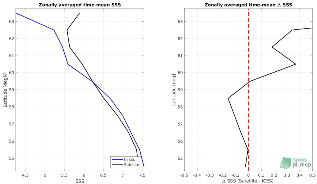
Figure 8: Left panel: Zonal mean SSS from SMAP SSS L4 OI v2 - Monthly (IPRC) satellite product (black) and from ICES (blue). Right panel: Zonal mean of \Delta SSS (Satellite - ICES) for all the collected Pi-MEP match-up pairs estimated over the full satellite product period.
