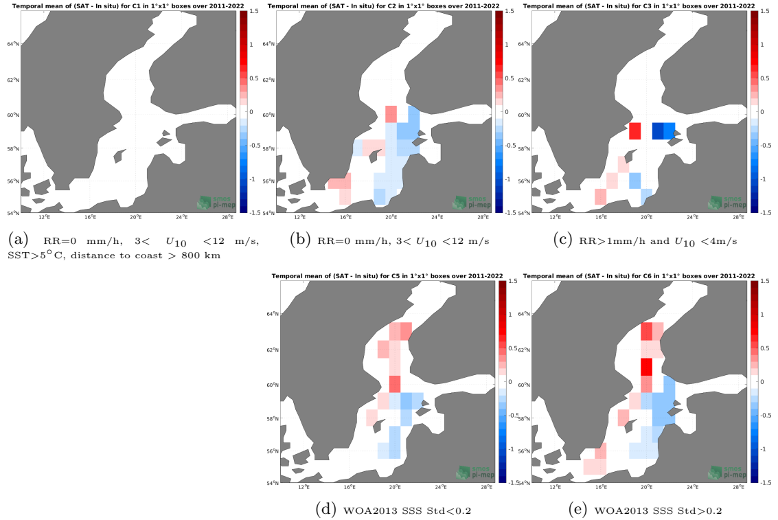
Figure 12: Temporal mean gridded over spatial boxes of size 1^{\circ}\times 1^{\circ} of \Delta\text{SSS} (SMAP SSS L4 OI v2 - Monthly (IPRC) - ICES) for 5 different subdatasets corresponding to:RR=0 mm/h, 3 < U_{10} < 12 m/s, SST >5^{\circ}\text{C} , distance to coast > 800 km (a), RR=0 mm/h, 3 < U_{10} < 12 m/s (b), RR >1 mm/h and U_{10} < 4 m/s (c), WOA2013 SSS Std <0.2 (d), WOA2013 SSS Std >0.2 (e).
