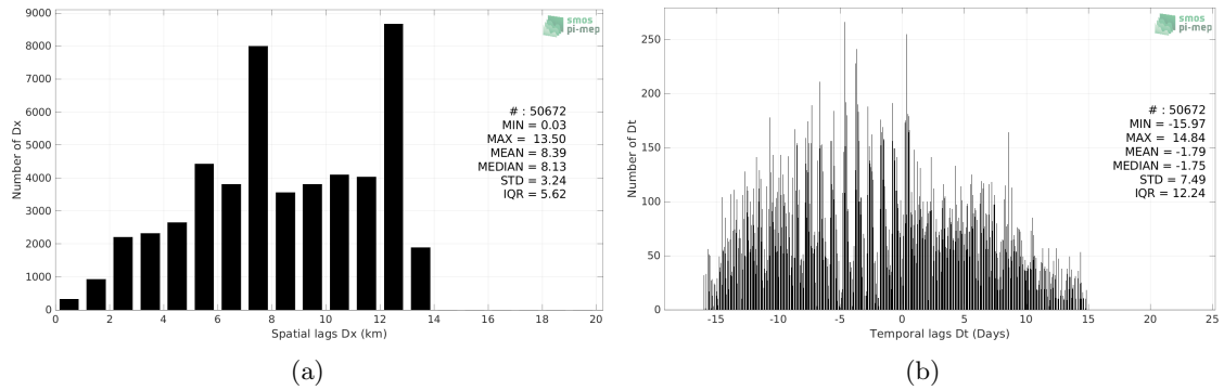
Figure 5: Histograms of the spatial (a) and temporal (b) lags between the location/time of the ICES measurement and the date of the corresponding SMAP SSS L4 OI v2 - Monthly (IPRC) SSS pixel.
