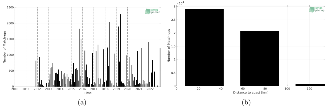
Figure 1: Number of match-ups between ICES and SMAP SSS L4 OI v2 - Monthly (IPRC) SSS as a function of time (a) and as function of the distance to coast (b) over the Baltic Sea Pi-MEP region and for the full satellite product period.
