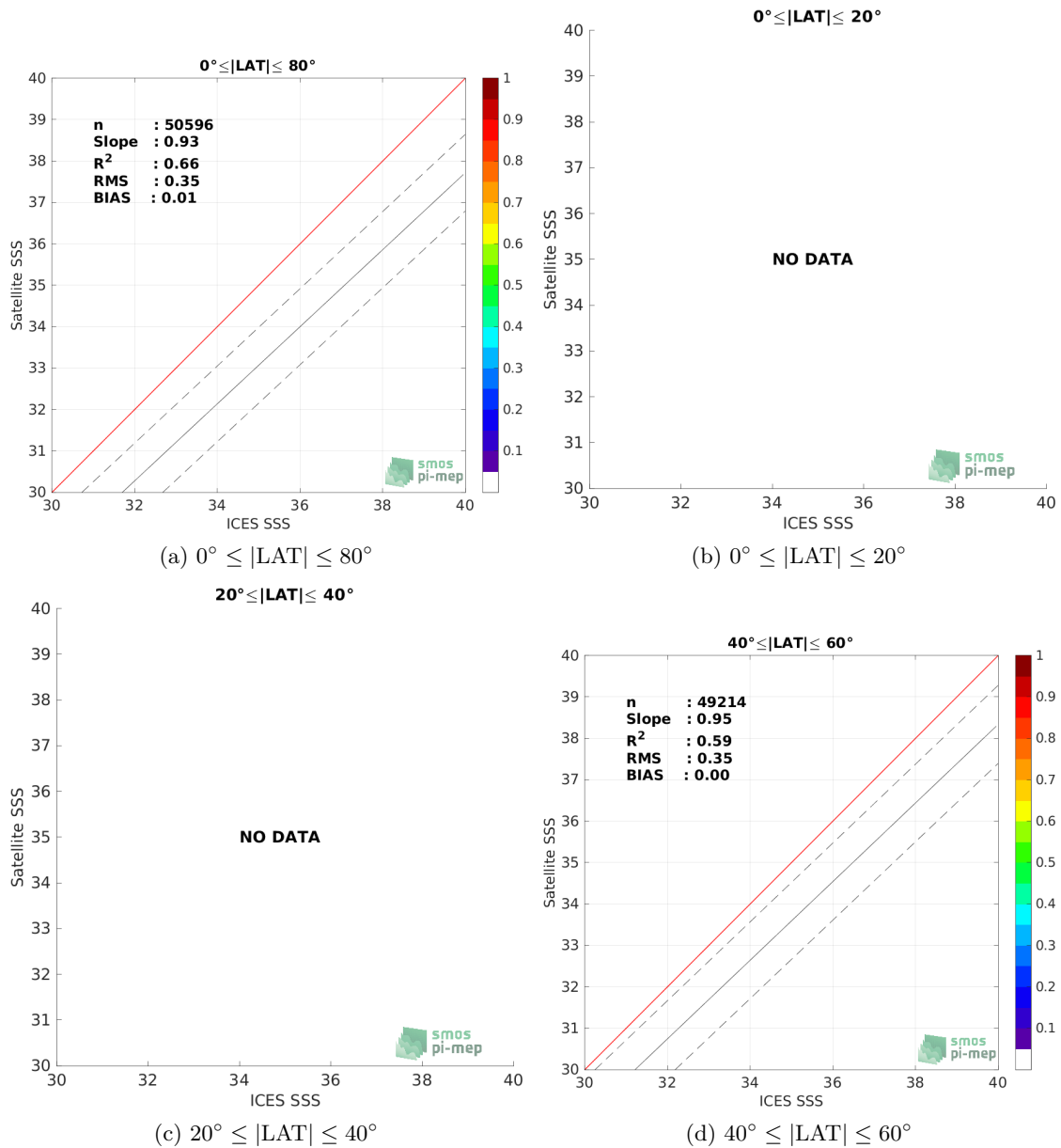
Figure 9: Contour maps of the concentration of SMAP SSS L4 OI v2 - Monthly (IPRC) SSS (y-axis) versus ICES SSS (x-axis) at match-up pairs for different latitude bands. For each plot, the red line shows x=y . The black thin and dashed lines indicate a linear fit through the data cloud and the \pm 95\% confidence levels, respectively. The number match-up pairs n , the slope and R^2 coefficient of the linear fit, the root mean square (RMS) and the mean bias between satellite and in situ data are indicated for each latitude band in each plots.
