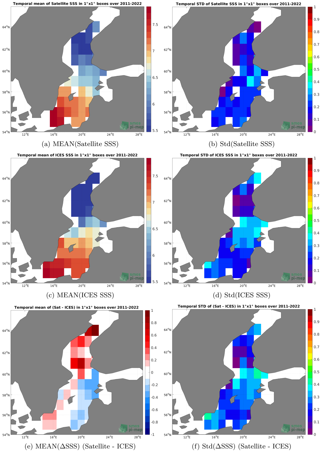
Figure 6: Temporal mean (left) and Std (right) of SSS from SMAP SSS L4 OI v2 - Monthly (IPRC) (top), ICES (middle), and of \Delta SSS (Satellite - ICES). Only match-up pairs are used to generate these maps.
