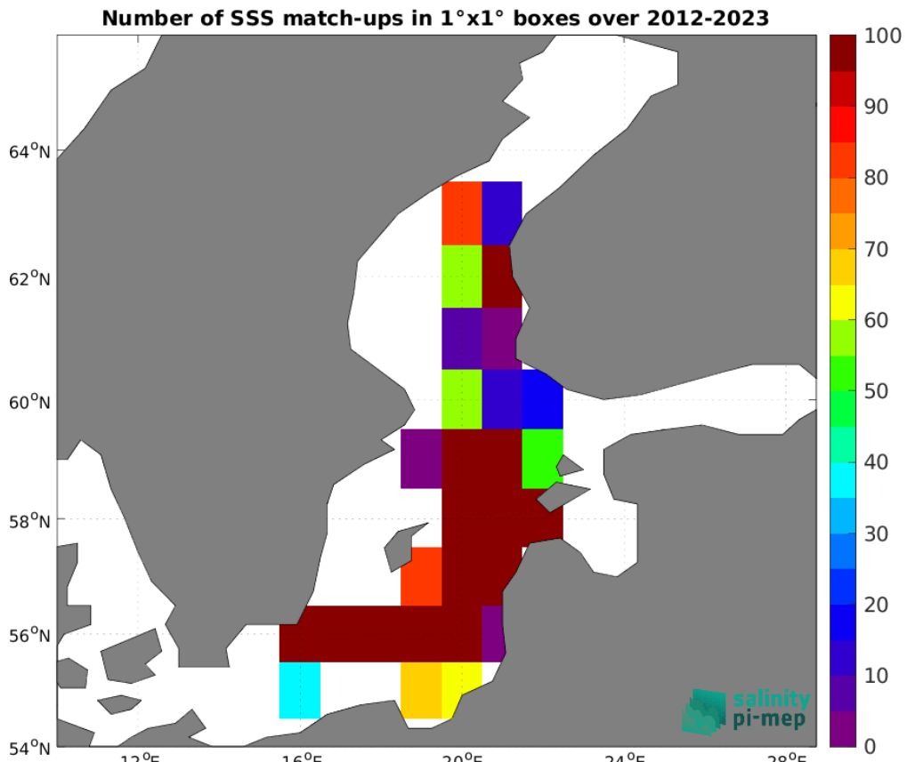
Figure 4: Number of SSS match-ups between Argo SSS and the SMAP SSS L4 OI v2 - Monthly (IPRC) SSS product for the Baltic Sea Pi-MEP region over 1^\circ \times 1^\circ boxes and for the full satellite product period.
