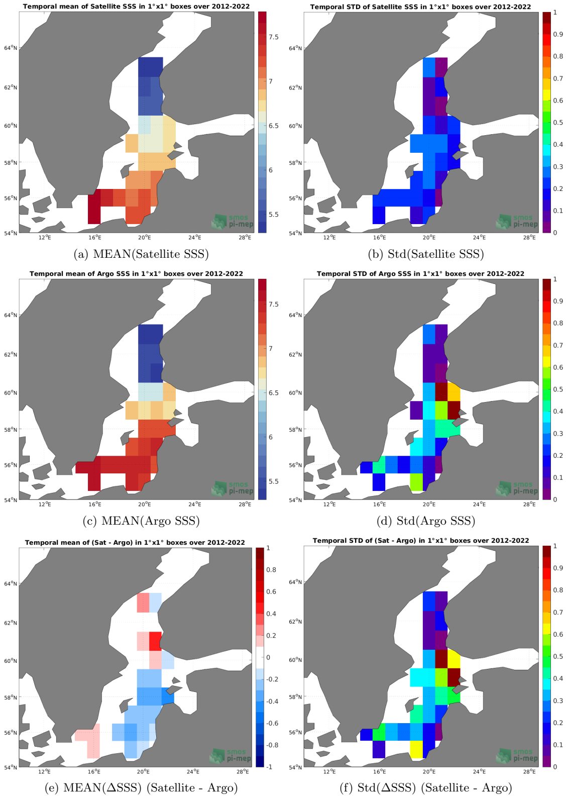
Figure 6: Temporal mean (left) and Std (right) of SSS from SMAP SSS L4 OI v2 - Monthly (IPRC) (top), Argo (middle), and of \Delta SSS (Satellite - Argo). Only match-up pairs are used to generate these maps.
