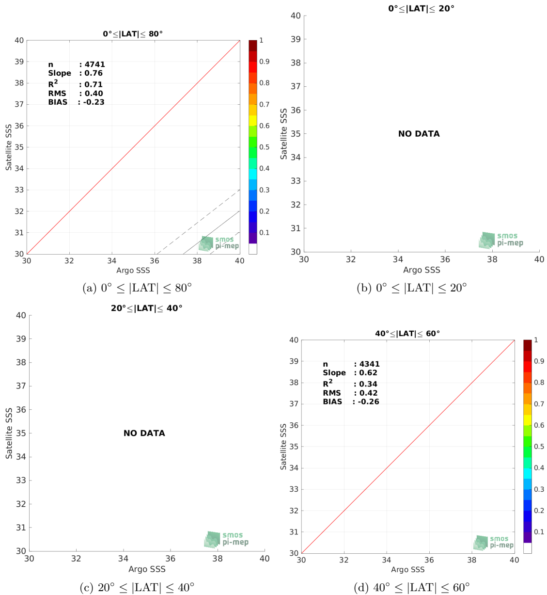
Figure 9: Contour maps of the concentration of SMAP SSS L4 OI v2 - Monthly (IPRC) SSS (y-axis) versus Argo SSS (x-axis) at match-up pairs for different latitude bands. For each plot, the red line shows x=y . The black thin and dashed lines indicate a linear fit through the data cloud and the \pm 95\% confidence levels, respectively. The number match-up pairs n , the slope and R^2 coefficient of the linear fit, the root mean square (RMS) and the mean bias between satellite and in situ data are indicated for each latitude band in each plots.
