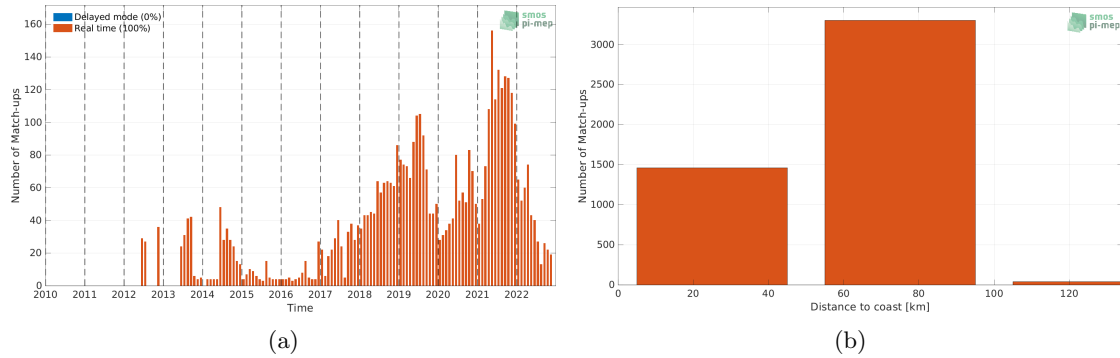
Figure 1: Number of match-ups between Argo and SMAP SSS L4 OI v2 - Monthly (IPRC) SSS as a function of time (a) and as function of the distance to coast (b) over the Baltic Sea Pi-MEP region and for the full satellite product period.
