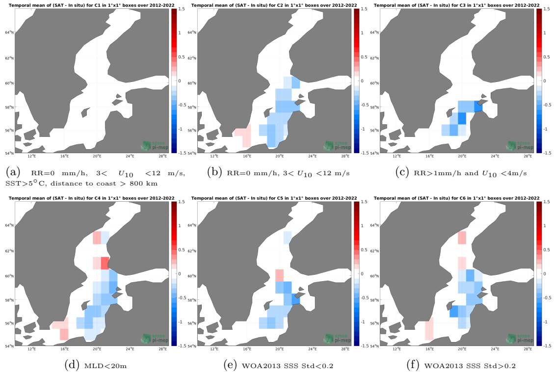
Figure 12: Temporal mean gridded over spatial boxes of size 1^{\circ}\times 1^{\circ} of \Delta\text{SSS} (SMAP SSS L4 OI v2 - Monthly (IPRC) - Argo) for 6 different subdatasets corresponding to:RR=0 mm/h, 3 < U_{10} < 12 m/s, SST >5^{\circ}\text{C} , distance to coast > 800 km (a), RR=0 mm/h, 3 < U_{10} < 12 m/s (b), RR >1 mm/h and U_{10} < 4 m/s (c),MLD <20 m (d),WOA2013 SSS Std <0.2 (e),WOA2013 SSS Std >0.2 (f).
