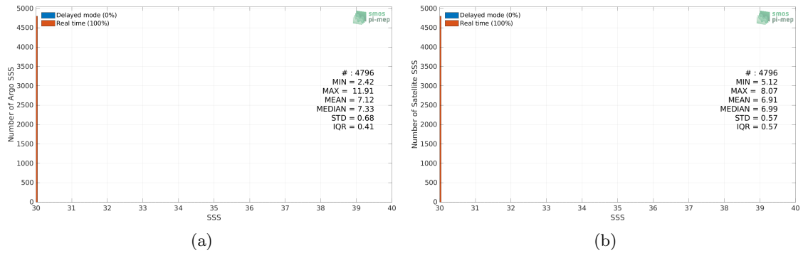
Figure 2: Histograms of SSS from Argo (a) and SMAP SSS L4 OI v2 - Monthly (IPRC) (b) considering all match-up pairs per bins of 0.1 over the Baltic Sea Pi-MEP region and for the full satellite product period.
