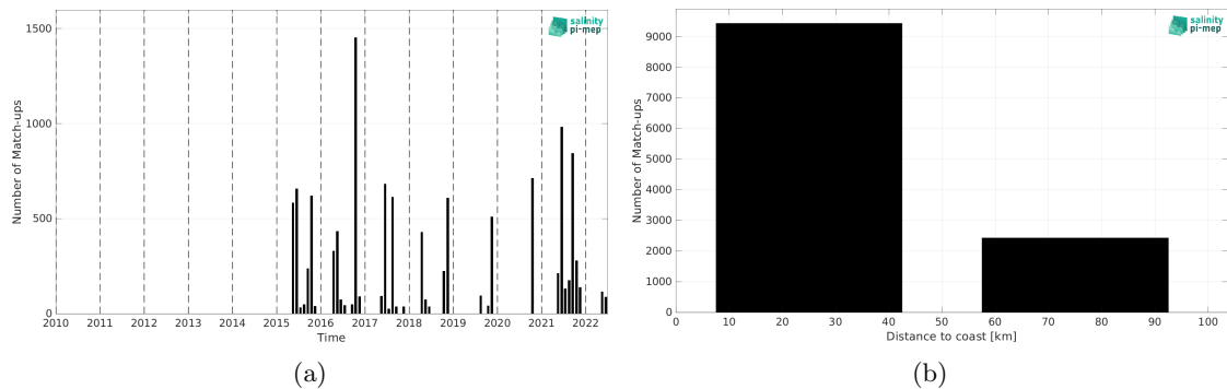
Figure 2: Number of match-ups between TSG (LEGOS-DM) and SMAP SSS L3 v6 - 8-Day running (RSS) SSS as a function of time (a) and as function of the distance to coast (b) over the Baltic Sea Pi-MEP region and for the full satellite product period.
