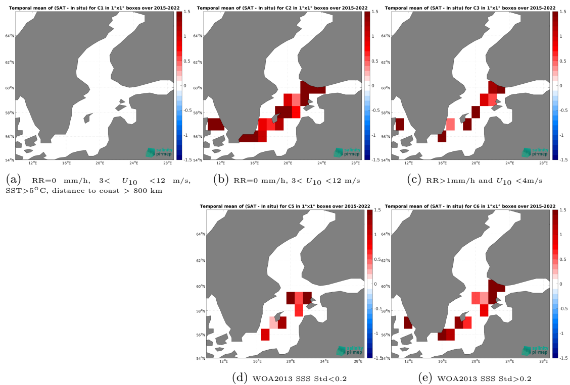
Figure 14: Temporal mean gridded over spatial boxes of size 1^\circ \times 1^\circ of \Delta SSS (SMAP SSS L3 v6 - 8-Day running (RSS) - TSG (LEGOS-DM)) for 5 different subdatasets corresponding to:RR=0 mm/h, 3 < U_{10} < 12 m/s, SST >5^\circ\text{C} , distance to coast > 800 km (a), RR=0 mm/h, 3 < U_{10} < 12 m/s (b), RR >1 mm/h and U_{10} < 4 m/s (c), WOA2013 SSS Std <0.2 (d), WOA2013 SSS Std >0.2 (e).
