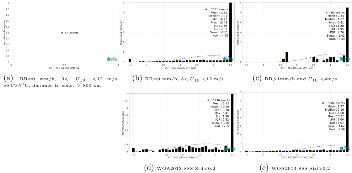
Figure 15: Normalized histogram of \Delta\text{SSS} (SMAP SSS L3 v6 - 8-Day running (RSS) - TSG (LEGOS-DM)) for 5 different subdatasets corresponding to: RR=0 mm/h, 3 < U_{10} < 12 m/s, SST > 5^{\circ}\text{C} , distance to coast > 800 km (a), RR=0 mm/h, 3 < U_{10} < 12 m/s (b), RR > 1\text{mm/h} and U_{10} < 4\text{m/s} (c), WOA2013 SSS Std < 0.2 (d), WOA2013 SSS Std > 0.2 (e).
