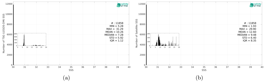
Figure 3: Histograms of SSS from TSG (LEGOS-DM) (a) and SMAP SSS L3 v6 - 8-Day running (RSS) (b) considering all match-up pairs per bins of 0.1 over the Baltic Sea Pi-MEP region and for the full satellite product period.
