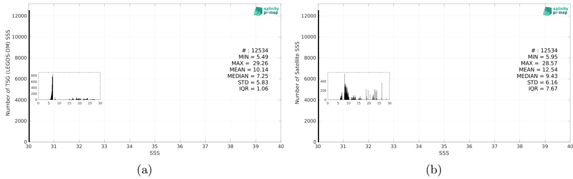
Figure 3: Histograms of SSS from TSG (LEGOS-DM) (a) and SMAP SSS L3 v6 - Monthly (RSS) (b) considering all match-up pairs per bins of 0.1 over the Baltic Sea Pi-MEP region and for the full satellite product period.
