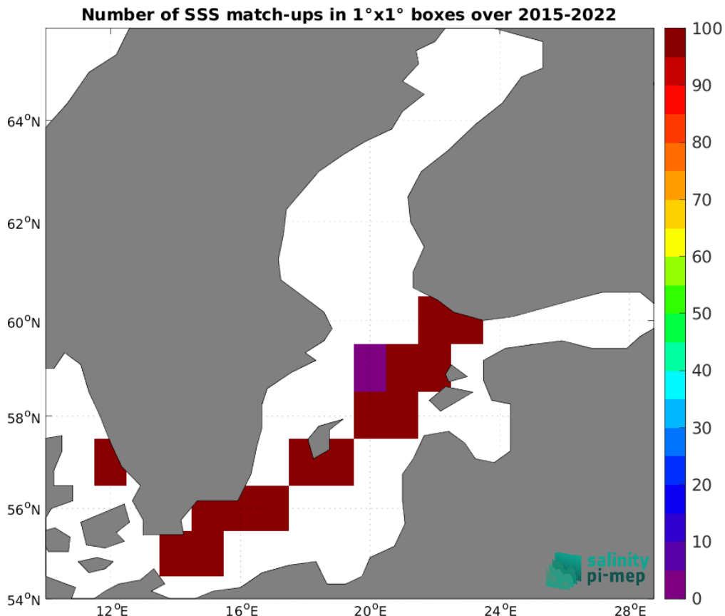
Figure 5: Number of SSS match-ups between TSG (LEGOS-DM) SSS and the SMAP SSS L3 v6 - Monthly (RSS) SSS product for the Baltic Sea Pi-MEP region over 1°×1° boxes and for the full satellite product period.
