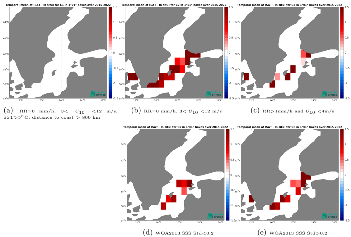
Figure 14: Temporal mean gridded over spatial boxes of size 1^\circ \times 1^\circ of \Delta SSS (SMAP SSS L3 v6 - Monthly (RSS) - TSG (LEGOS-DM)) for 5 different subdatasets corresponding to:RR=0 mm/h, 3 < U_{10} < 12 m/s, SST >5^\circ\text{C} , distance to coast > 800 km (a), RR=0 mm/h, 3 < U_{10} < 12 m/s (b), RR >1 mm/h and U_{10} < 4 m/s (c), WOA2013 SSS Std <0.2 (d), WOA2013 SSS Std >0.2 (e).
