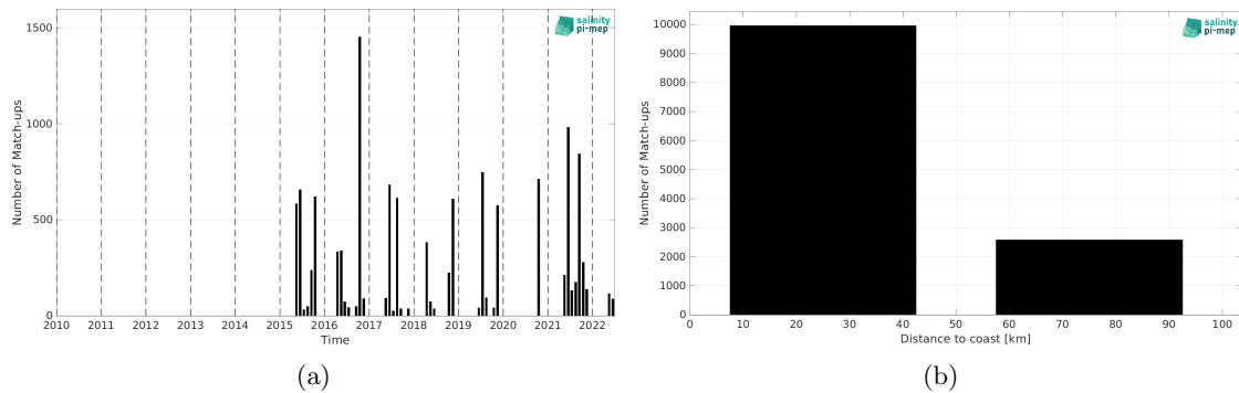
Figure 2: Number of match-ups between TSG (LEGOS-DM) and SMAP SSS L3 v6 - Monthly (RSS) SSS as a function of time (a) and as function of the distance to coast (b) over the Baltic Sea Pi-MEP region and for the full satellite product period.
